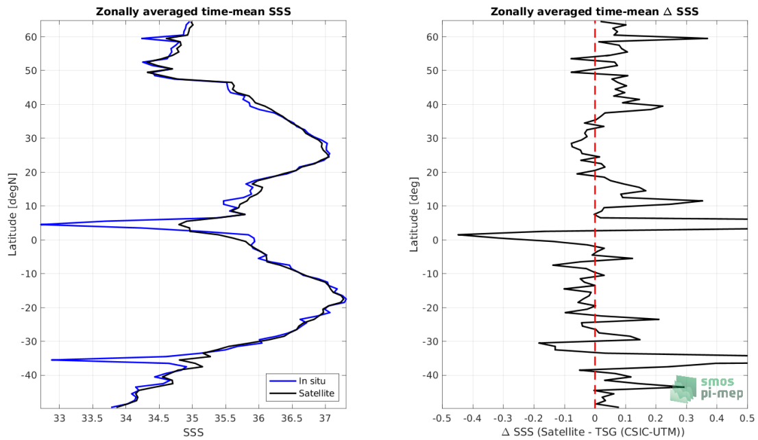
Figure 8: Left panel: Zonal mean SSS from SMOS SSS L4 v1 - Weekly (CMEMS-CNR) satellite product (black) and from TSG (CSIC-UTM) (blue). Right panel: Zonal mean of \Delta SSS (Satellite - TSG (CSIC-UTM)) for all the collected Pi-MEP match-up pairs estimated over the full satellite product period.
