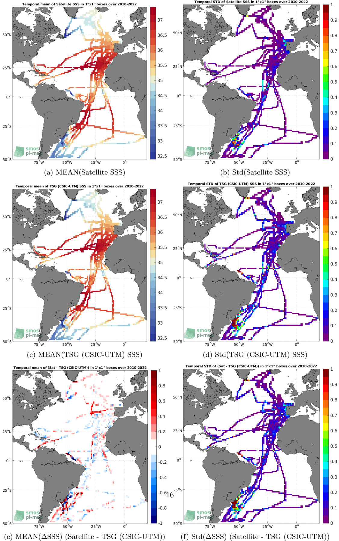
Figure 6: Temporal mean (left) and Std (right) of SSS from SMOS SSS L4 v1 - Weekly (CMEMS-CNR) (top), TSG (CSIC-UTM) (middle), and of \Delta SSS (Satellite - TSG (CSIC-UTM)). Only match-up pairs are used to generate these maps.
