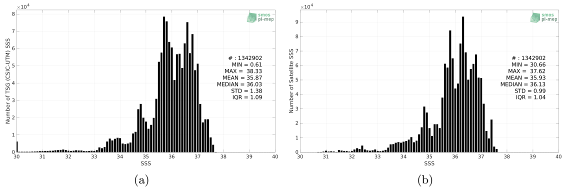
Figure 2: Histograms of SSS from TSG (CSIC-UTM) (a) and SMOS SSS L4 v1 - Weekly (CMEMS-CNR) (b) considering all match-up pairs per bins of 0.1 over the Atlantic Ocean Pi-MEP region and for the full satellite product period.
