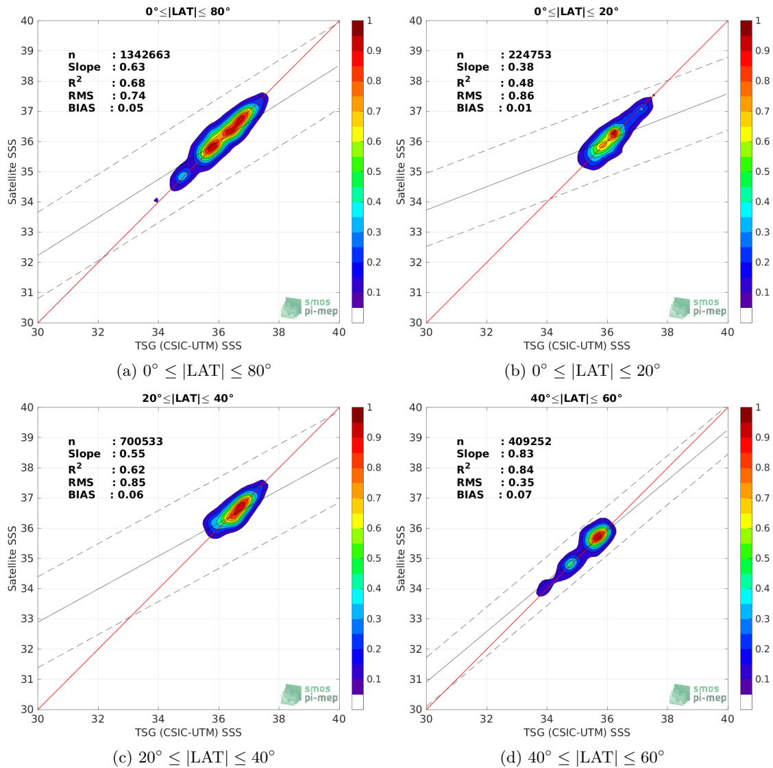
Figure 9: Contour maps of the concentration of SMOS SSS L4 v1 - Weekly (CMEMS-CNR) SSS (y-axis) versus TSG (CSIC-UTM) SSS (x-axis) at match-up pairs for different latitude bands. For each plot, the red line shows x=y . The black thin and dashed lines indicate a linear fit through the data cloud and the \pm 95\% confidence levels, respectively. The number match-up pairs n , the slope and R^2 coefficient of the linear fit, the root mean square (RMS) and the mean bias between satellite and in situ data are indicated for each latitude band in each plots.
