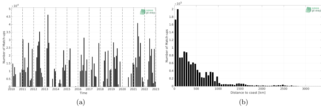
Figure 1: Number of match-ups between TSG (CSIC-UTM) and SMOS SSS L4 v1 - Weekly (CMEMS-CNR) SSS as a function of time (a) and as function of the distance to coast (b) over the Atlantic Ocean Pi-MEP region and for the full satellite product period.
