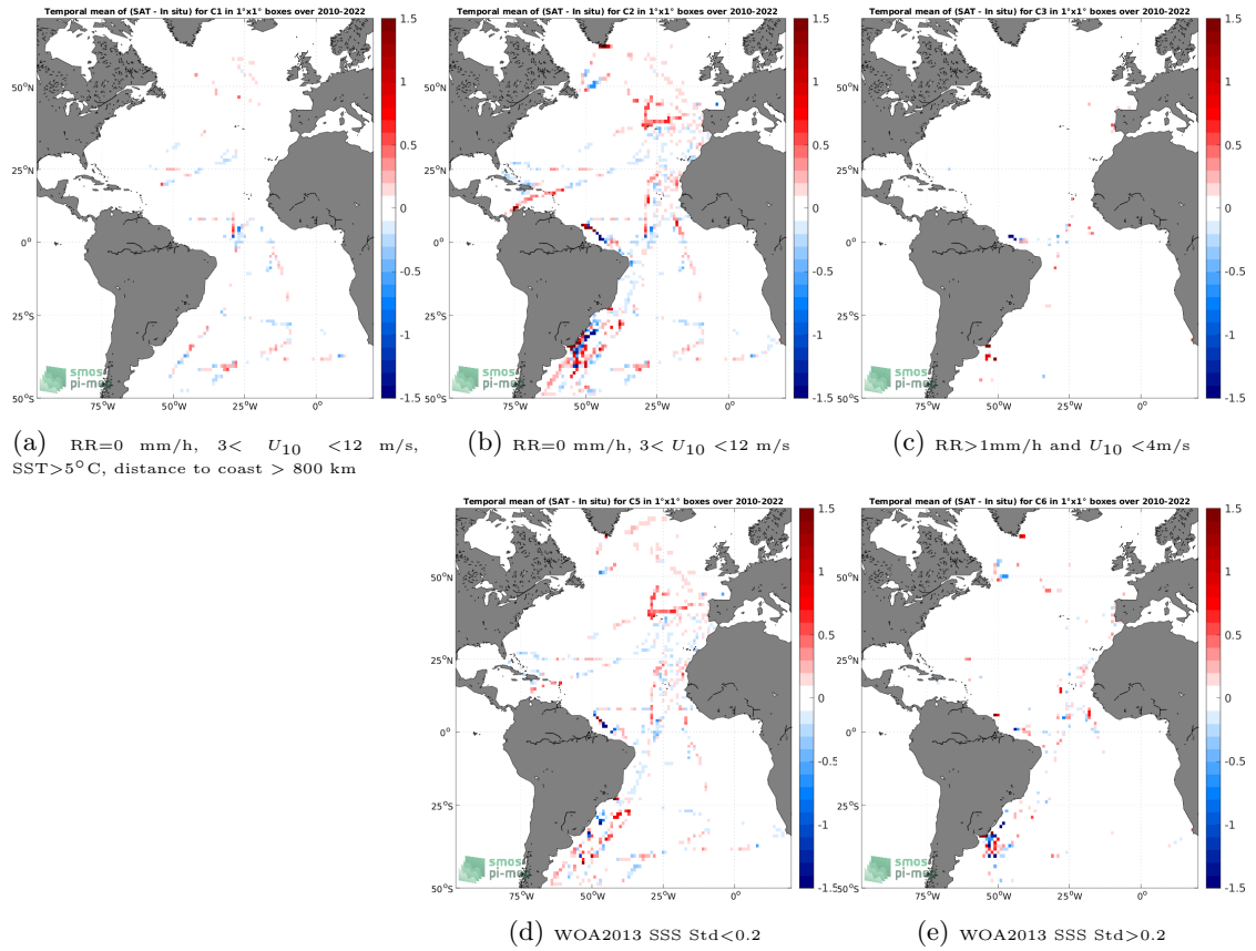
Figure 12: Temporal mean gridded over spatial boxes of size 1^\circ \times 1^\circ of \Delta SSS (SMOS SSS L4 v1 - Weekly (CMEMS-CNR) - TSG (CSIC-UTM)) for 5 different subdatasets corresponding to:RR=0 mm/h, 3 < U_{10} < 12 m/s, SST >5^\circ\text{C} , distance to coast > 800 km (a), RR=0 mm/h, 3 < U_{10} < 12 m/s (b), RR >1 mm/h and U_{10} < 4 m/s (c), WOA2013 SSS Std <0.2 (d), WOA2013 SSS Std >0.2 (e).
