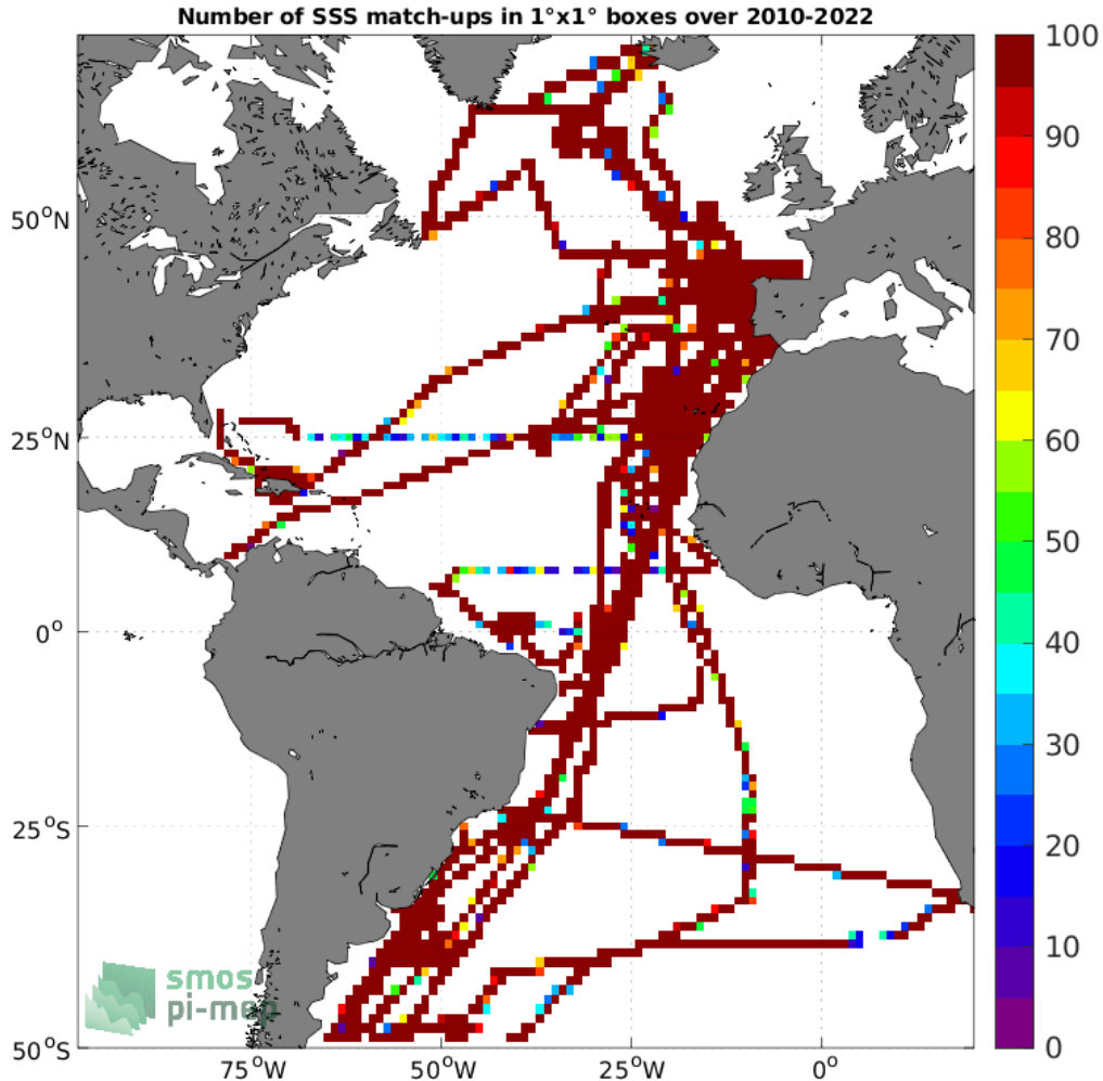
Figure 4: Number of SSS match-ups between TSG (CSIC-UTM) SSS and the SMOS SSS L4 v1 - Weekly (CMEMS-CNR) SSS product for the Atlantic Ocean Pi-MEP region over 1^\circ \times 1^\circ boxes and for the full satellite product period.
