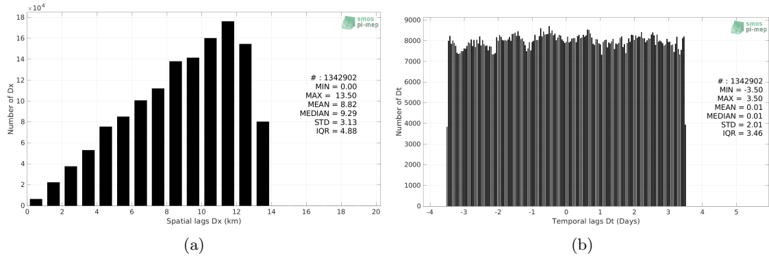
Figure 5: Histograms of the spatial (a) and temporal (b) lags between the location/time of the TSG (CSIC-UTM) measurement and the date of the corresponding SMOS SSS L4 v1 - Weekly (CMEMS-CNR) SSS pixel.
