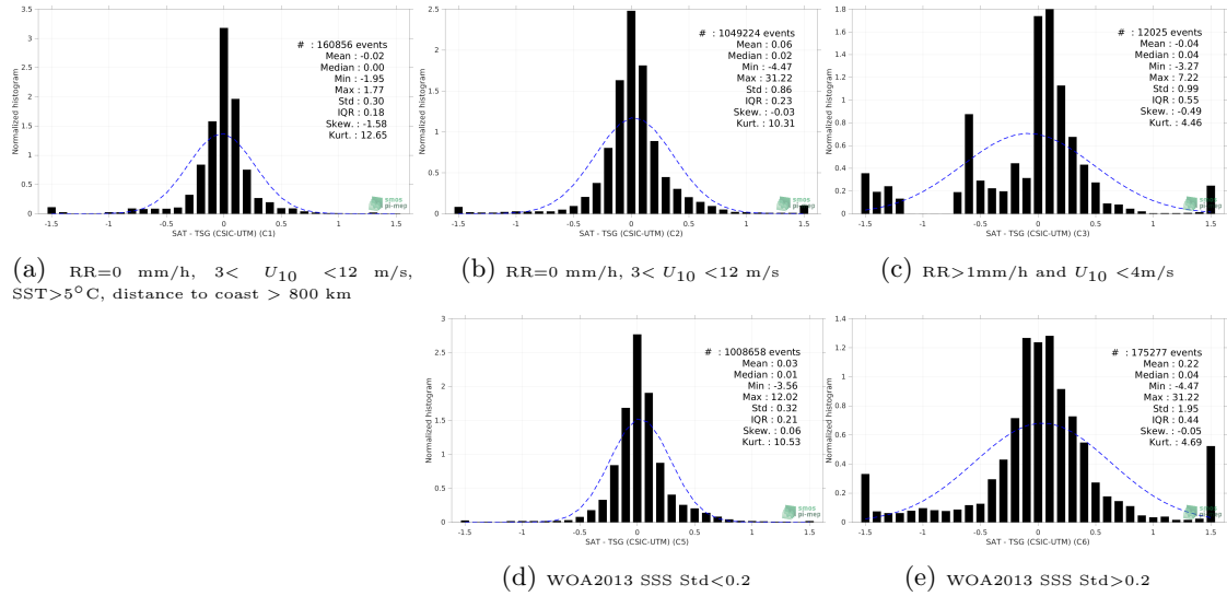
Figure 13: Normalized histogram of \Delta SSS (SMOS SSS L4 v1 - Weekly (CMEMS-CNR) - TSG (CSIC-UTM)) for 5 different subdatasets corresponding to: RR=0 mm/h, 3 < U_{10} < 12 m/s, SST > 5°C, distance to coast > 800 km (a), RR=0 mm/h, 3 < U_{10} < 12 m/s (b), RR > 1mm/h and U_{10} < 4 m/s (c), WOA2013 SSS Std < 0.2 (d), WOA2013 SSS Std > 0.2 (e).
