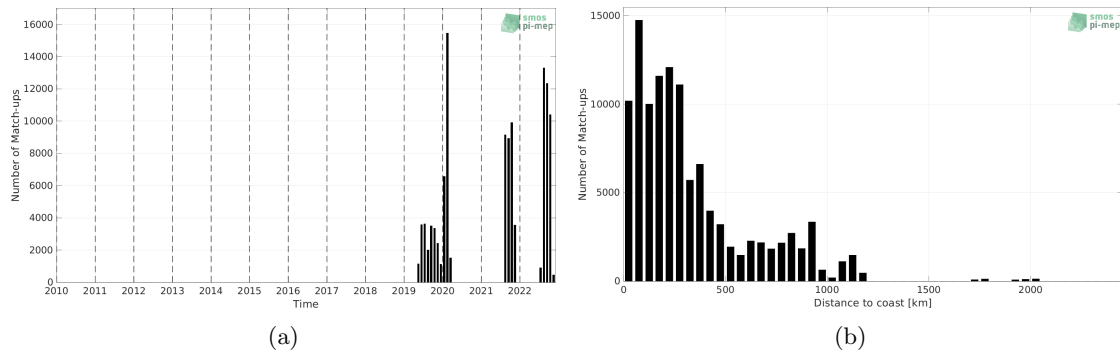
Figure 1: Number of match-ups between Saildrone and SMOS SSS L4 v1 - Weekly (CMEMS-CNR) SSS as a function of time (a) and as function of the distance to coast (b) over the Atlantic Ocean Pi-MEP region and for the full satellite product period.
