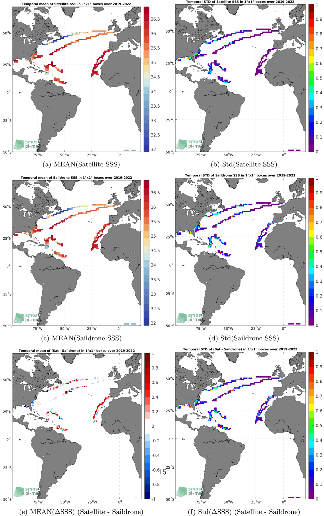
Figure 6: Temporal mean (left) and Std (right) of SSS from SMOS SSS L4 v1 - Weekly (CMEMS-CNR) (top), Saildrone (middle), and of \Delta SSS (Satellite - Saildrone). Only match-up pairs are used to generate these maps.
