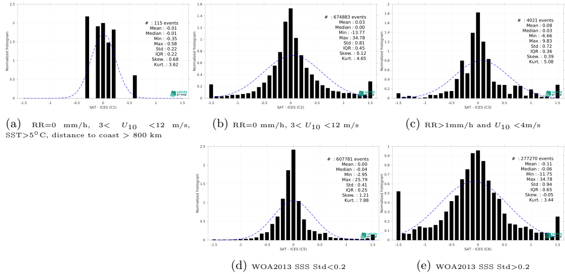
Figure 13: Normalized histogram of \Delta SSS (SMOS SSS L4 v1 - Weekly (CMEMS-CNR) - ICES) for 5 different subdatasets corresponding to: RR=0 mm/h, 3 < U_{10} < 12 m/s, SST>5°C, distance to coast > 800 km (a), RR=0 mm/h, 3 < U_{10} < 12 m/s (b), RR>1mm/h and U_{10} < 4 m/s (c), WOA2013 SSS Std<0.2 (d), WOA2013 SSS Std>0.2 (e).
