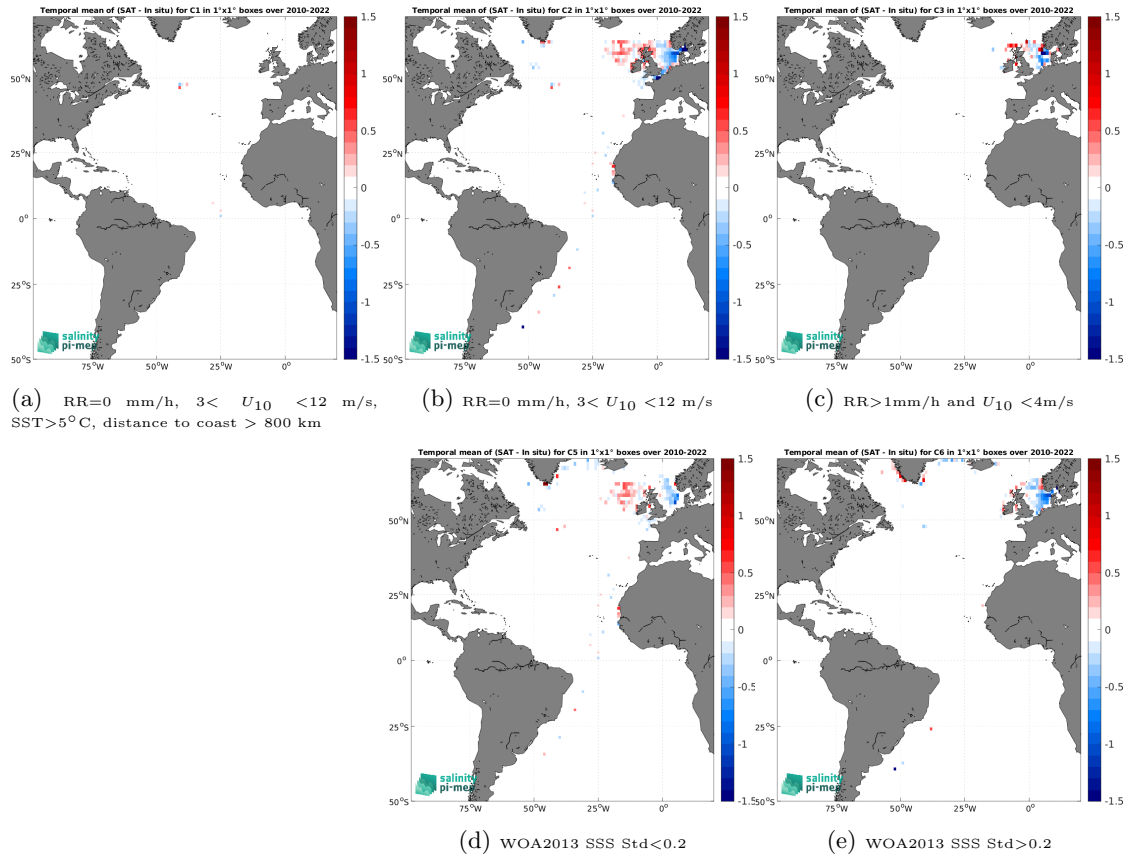
Figure 12: Temporal mean gridded over spatial boxes of size 1^\circ \times 1^\circ of \Delta SSS (SMOS SSS L4 v1 - Weekly (CMEMS-CNR) - ICES) for 5 different subdatasets corresponding to:RR=0 mm/h, 3 < U_{10} < 12 m/s, SST >5^\circ\text{C} , distance to coast > 800 km (a), RR=0 mm/h, 3 < U_{10} < 12 m/s (b), RR >1 mm/h and U_{10} < 4 m/s (c), WOA2013 SSS Std <0.2 (d), WOA2013 SSS Std >0.2 (e).
