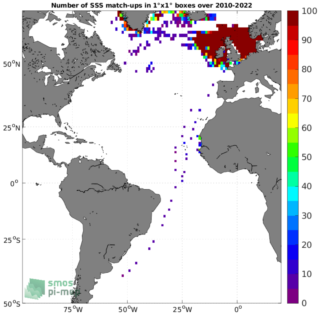
Figure 4: Number of SSS match-ups between ICES SSS and the SMOS SSS L4 v1 - Weekly (CMEMS-CNR) SSS product for the Atlantic Ocean Pi-MEP region over 1^\circ \times 1^\circ boxes and for the full satellite product period.
