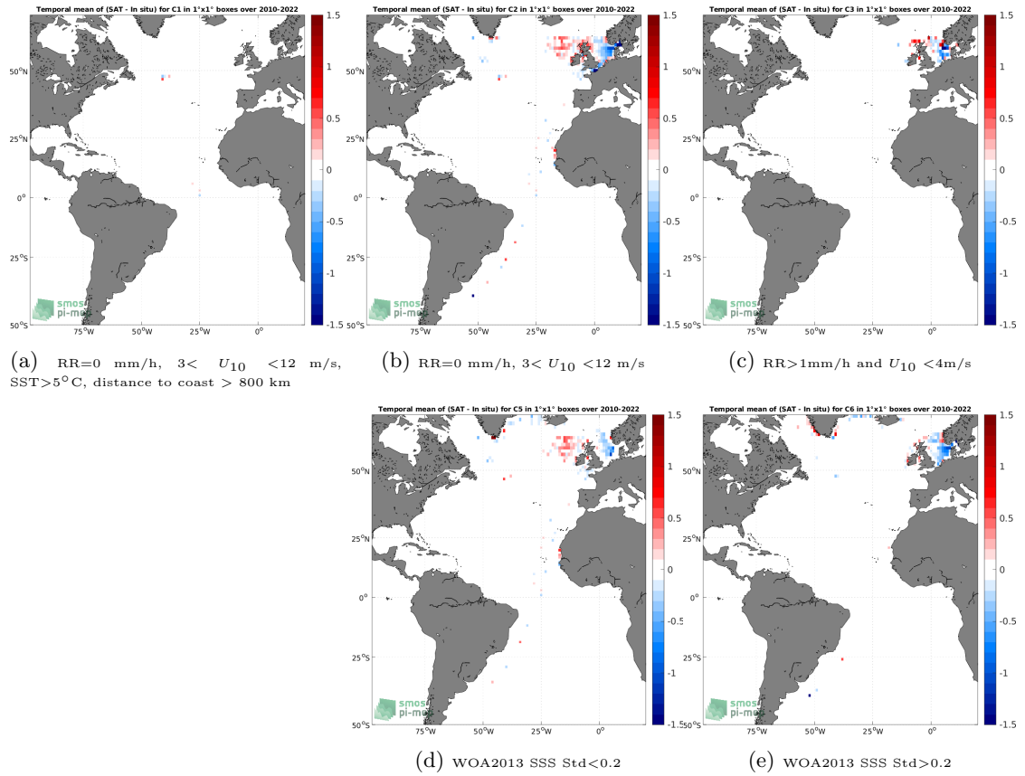
Figure 12: Temporal mean gridded over spatial boxes of size 1^\circ \times 1^\circ of \Delta\text{SSS} (SMOS SSS L4 v1 - Weekly (CMEMS-CNR) - ICES) for 5 different subdatasets corresponding to:RR=0 mm/h, 3 < U_{10} < 12 m/s, SST >5^\circ\text{C} , distance to coast > 800 km (a), RR=0 mm/h, 3 < U_{10} < 12 m/s (b), RR >1 mm/h and U_{10} < 4 m/s (c), WOA2013 SSS Std <0.2 (d), WOA2013 SSS Std >0.2 (e).
