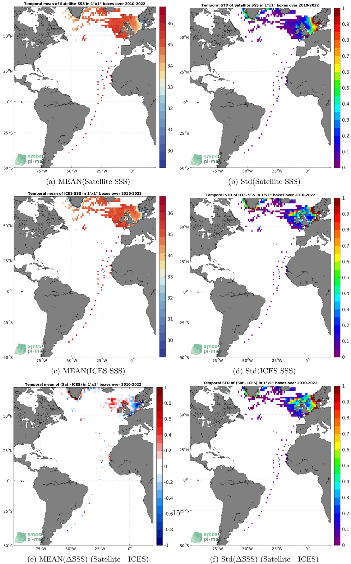
Figure 6: Temporal mean (left) and Std (right) of SSS from SMOS SSS L4 v1 - Weekly (CMEMS-CNR) (top), ICES (middle), and of \Delta SSS (Satellite - ICES). Only match-up pairs are used to generate these maps.
