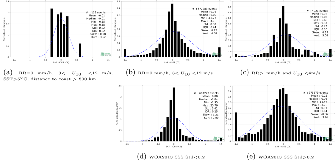
Figure 13: Normalized histogram of \Delta SSS (SMOS SSS L4 v1 - Weekly (CMEMS-CNR) - ICES) for 5 different subdatasets corresponding to: RR=0 mm/h, 3 < U_{10} < 12 m/s, SST > 5°C, distance to coast > 800 km (a), RR=0 mm/h, 3 < U_{10} < 12 m/s (b), RR > 1mm/h and U_{10} < 4 m/s (c), WOA2013 SSS Std < 0.2 (d), WOA2013 SSS Std > 0.2 (e).
