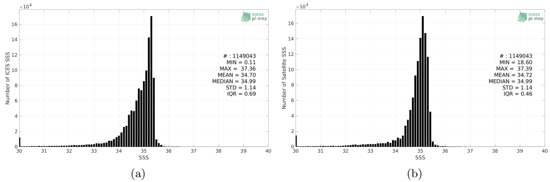
Figure 2: Histograms of SSS from ICES (a) and SMOS SSS L4 v1 - Weekly (CMEMS-CNR) (b) considering all match-up pairs per bins of 0.1 over the Atlantic Ocean Pi-MEP region and for the full satellite product period.
