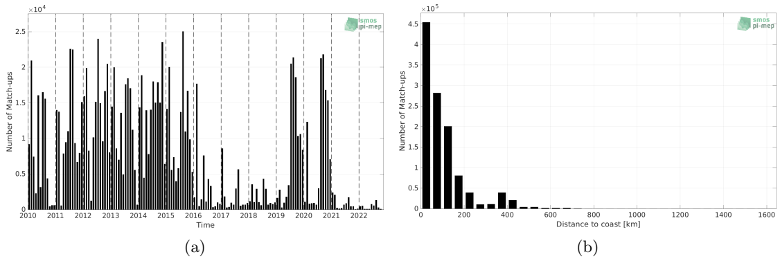
Figure 1: Number of match-ups between ICES and SMOS SSS L4 v1 - Weekly (CMEMS-CNR) SSS as a function of time (a) and as function of the distance to coast (b) over the Atlantic Ocean Pi-MEP region and for the full satellite product period.
