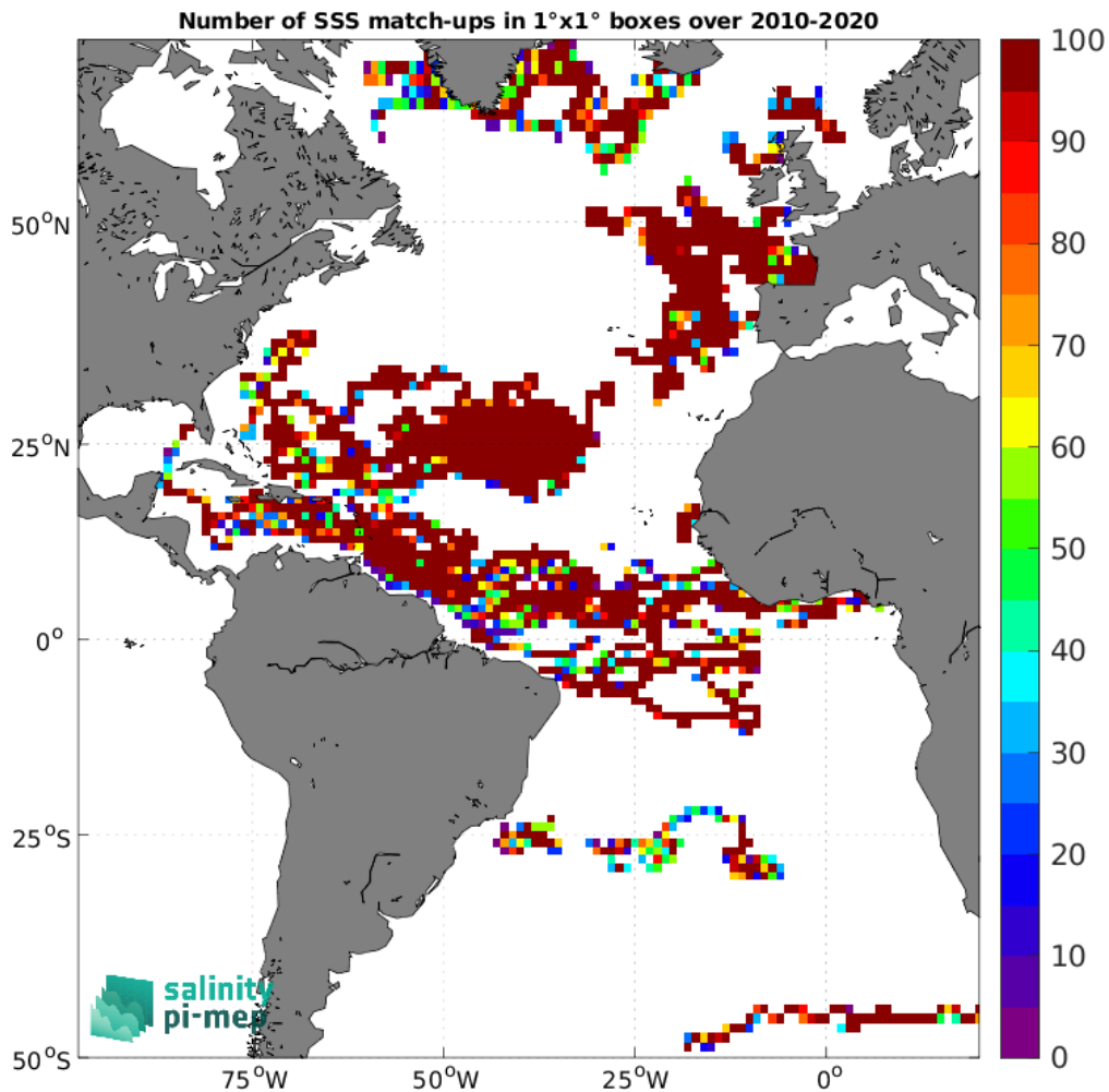
Figure 3: Number of SSS match-ups between Surface drifters SSS and the SMOS SSS L4 v1 - Weekly (CMEMS-CNR) SSS product for the Atlantic Ocean Pi-MEP region over 1°×1° boxes and for the full satellite product period.
