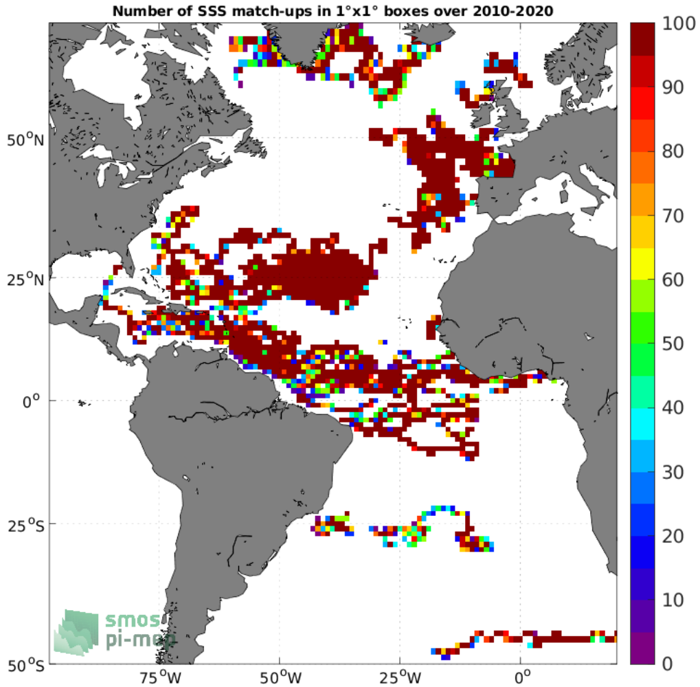
Figure 3: Number of SSS match-ups between Surface drifters SSS and the SMOS SSS L4 v1 - Weekly (CMEMS-CNR) SSS product for the Atlantic Ocean Pi-MEP region over 1^\circ \times 1^\circ boxes and for the full satellite product period.
