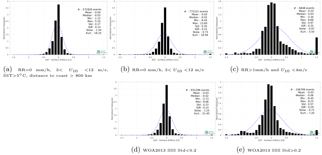
Figure 12: Normalized histogram of \Delta\text{SSS} (SMOS SSS L4 v1 - Weekly (CMEMS-CNR) - Surface drifters) for 5 different subdatasets corresponding to: RR=0 mm/h, 3 < U_{10} < 12 m/s, SST>5°C, distance to coast > 800 km (a), RR=0 mm/h, 3 < U_{10} < 12 m/s (b), RR>1mm/h and U_{10} < 4 m/s (c), WOA2013 SSS Std<0.2 (d), WOA2013 SSS Std>0.2 (e).
