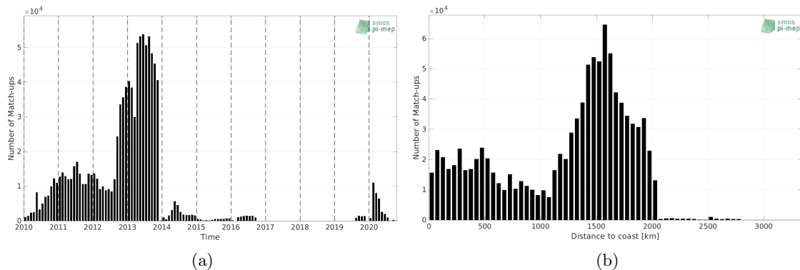
Figure 1: Number of match-ups between Surface drifters and SMOS SSS L4 v1 - Weekly (CMEMS-CNR) SSS as a function of time (a) and as function of the distance to coast (b) over the Atlantic Ocean Pi-MEP region and for the full satellite product period.
