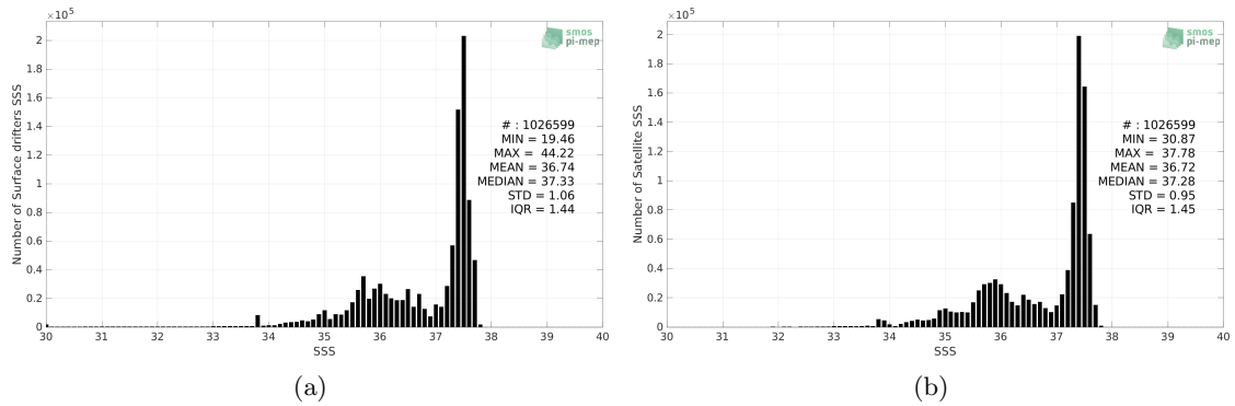
Figure 2: Histograms of SSS from Surface drifters (a) and SMOS SSS L4 v1 - Weekly (CMEMS-CNR) (b) considering all match-up pairs per bins of 0.1 over the Atlantic Ocean Pi-MEP region and for the full satellite product period.
