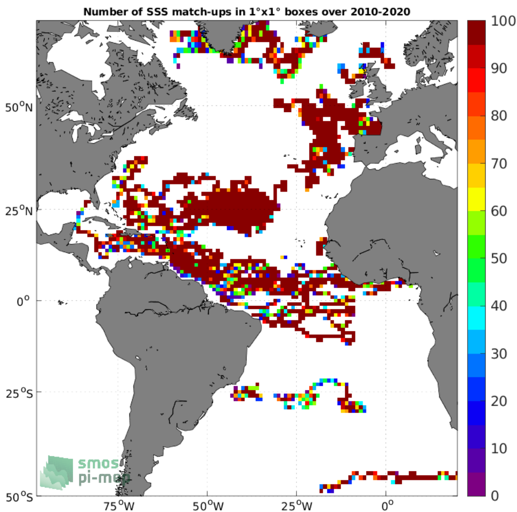
Figure 3: Number of SSS match-ups between Surface drifters SSS and the SMOS SSS L4 v1 - Weekly (CMEMS-CNR) SSS product for the Atlantic Ocean Pi-MEP region over 1°x1° boxes and for the full satellite product period.
