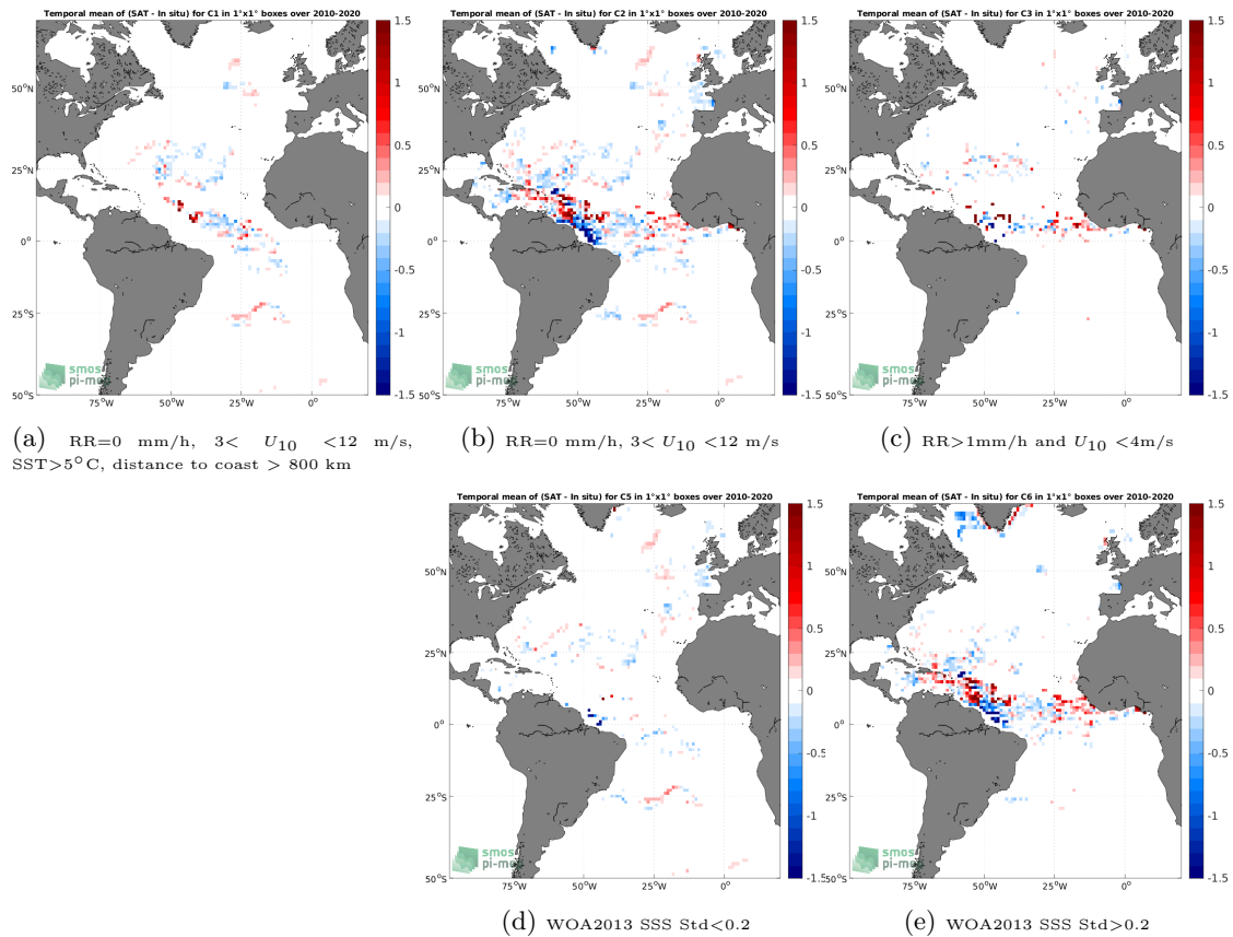
Figure 11: Temporal mean gridded over spatial boxes of size 1^\circ \times 1^\circ of \Delta SSS (SMOS SSS L4 v1 - Weekly (CMEMS-CNR) - Surface drifters) for 5 different subdatasets corresponding to:RR=0 mm/h, 3 < U_{10} < 12 m/s, SST >5^\circ C, distance to coast > 800 km (a), RR=0 mm/h, 3 < U_{10} < 12 m/s (b), RR >1 mm/h and U_{10} < 4 m/s (c), WOA2013 SSS Std <0.2 (d), WOA2013 SSS Std >0.2 (e).
