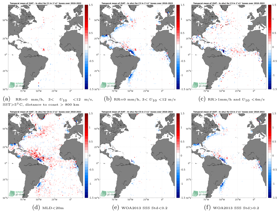
Figure 12: Temporal mean gridded over spatial boxes of size 1^\circ \times 1^\circ of \Delta SSS (SMOS SSS L4 v1 - Weekly (CMEMS-CNR) - Argo) for 6 different subdatasets corresponding to:RR=0 mm/h, 3 < U_{10} < 12 m/s, SST>5°C, distance to coast > 800 km (a), RR=0 mm/h, 3 < U_{10} < 12 m/s (b), RR>1mm/h and U_{10} < 4 m/s (c),MLD<20m (d),WOA2013 SSS Std<0.2 (e),WOA2013 SSS Std>0.2 (f).
