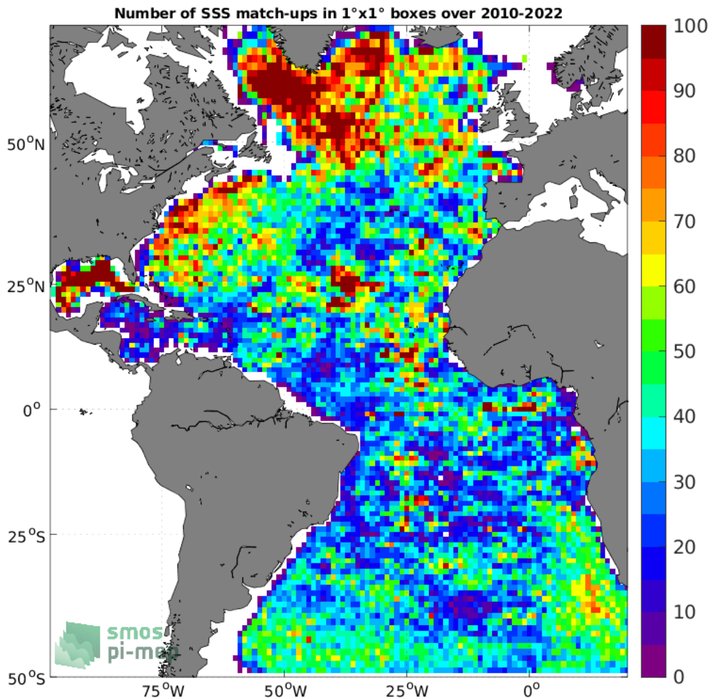
Figure 4: Number of SSS match-ups between Argo SSS and the SMOS SSS L4 v1 - Weekly (CMEMS-CNR) SSS product for the Atlantic Ocean Pi-MEP region over 1^\circ \times 1^\circ boxes and for the full satellite product period.
