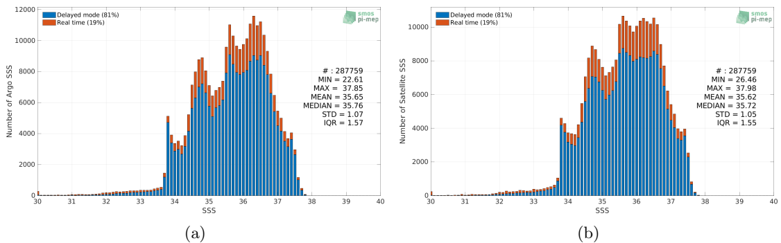
Figure 2: Histograms of SSS from Argo (a) and SMOS SSS L4 v1 - Weekly (CMEMS-CNR) (b) considering all match-up pairs per bins of 0.1 over the Atlantic Ocean Pi-MEP region and for the full satellite product period.
