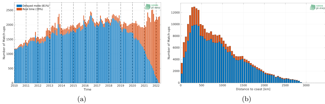
Figure 1: Number of match-ups between Argo and SMOS SSS L4 v1 - Weekly (CMEMS-CNR) SSS as a function of time (a) and as function of the distance to coast (b) over the Atlantic Ocean Pi-MEP region and for the full satellite product period.
