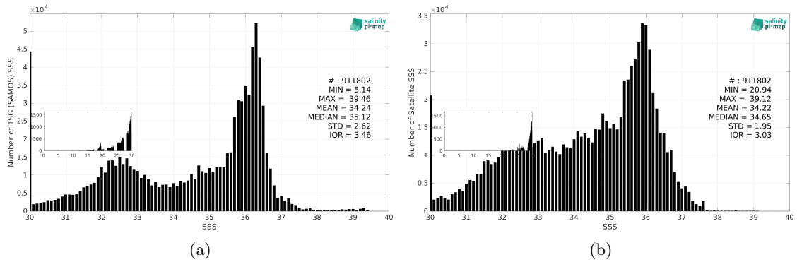
Figure 3: Histograms of SSS from TSG (SAMOS) (a) and SMOS SSS L4 v1 - Monthly (CMEMS-CNR) (b) considering all match-up pairs per bins of 0.1 over the Atlantic Ocean Pi-MEP region and for the full satellite product period.
