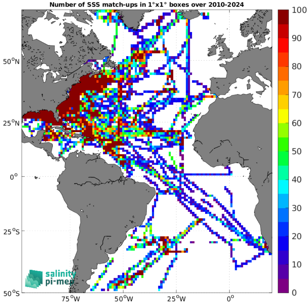
Figure 5: Number of SSS match-ups between TSG (SAMOS) SSS and the SMOS SSS L4 v1 - Monthly (CMEMS-CNR) SSS product for the Atlantic Ocean Pi-MEP region over 1^\circ \times 1^\circ boxes and for the full satellite product period.
