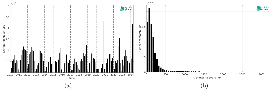
Figure 2: Number of match-ups between TSG (SAMOS) and SMOS SSS L4 v1 - Monthly (CMEMS-CNR) SSS as a function of time (a) and as function of the distance to coast (b) over the Atlantic Ocean Pi-MEP region and for the full satellite product period.
