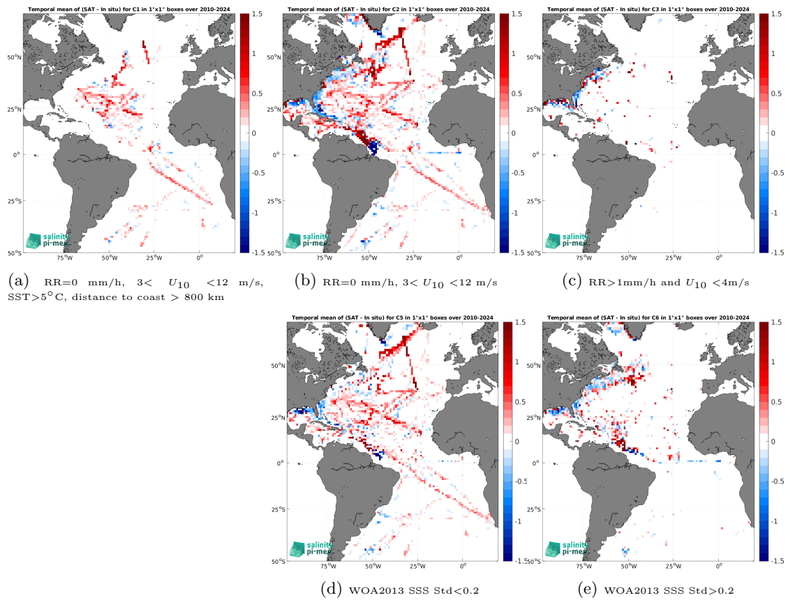
Figure 14: Temporal mean gridded over spatial boxes of size 1^\circ \times 1^\circ of \Delta\text{SSS} (SMOS SSS L4 v1 - Monthly (CMEMS-CNR) - TSG (SAMOS)) for 5 different subdatasets corresponding to:RR=0 mm/h, 3 < U_{10} < 12 m/s, SST>5°C, distance to coast > 800 km (a), RR=0 mm/h, 3 < U_{10} < 12 m/s (b), RR>1mm/h and U_{10} < 4 m/s (c), WOA2013 SSS Std<0.2 (d), WOA2013 SSS Std>0.2 (e).
