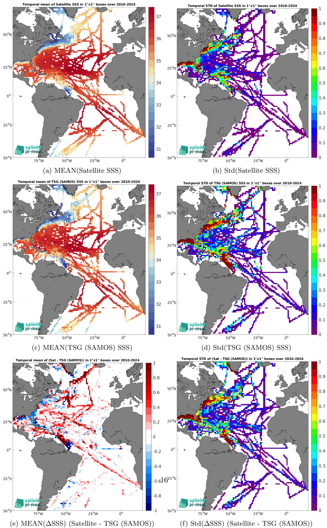
Figure 7: Temporal mean (left) and Std (right) of SSS from SMOS SSS L4 v1 - Monthly (CMEMS-CNR) (top), TSG (SAMOS) (middle), and of \Delta SSS (Satellite - TSG (SAMOS)). Only match-up pairs are used to generate these maps.
