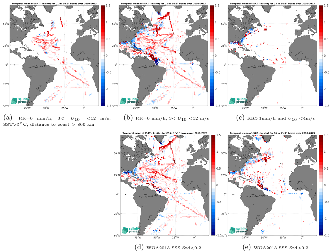
Figure 12: Temporal mean gridded over spatial boxes of size 1^\circ \times 1^\circ of \Delta SSS (SMOS SSS L4 v1 - Monthly (CMEMS-CNR) - TSG (SAMOS)) for 5 different subdatasets corresponding to:RR=0 mm/h, 3 < U_{10} < 12 m/s, SST >5^\circ\text{C} , distance to coast > 800 km (a), RR=0 mm/h, 3 < U_{10} < 12 m/s (b), RR >1 mm/h and U_{10} < 4 m/s (c), WOA2013 SSS Std <0.2 (d), WOA2013 SSS Std >0.2 (e).
