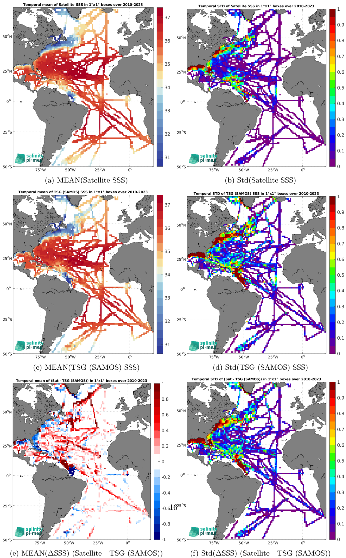
Figure 6: Temporal mean (left) and Std (right) of SSS from SMOS SSS L4 v1 - Monthly (CMEMS-CNR) (top), TSG (SAMOS) (middle), and of \Delta SSS (Satellite - TSG (SAMOS)). Only match-up pairs are used to generate these maps.
