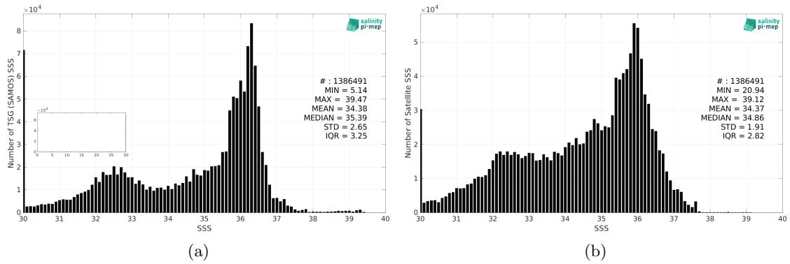
Figure 2: Histograms of SSS from TSG (SAMOS) (a) and SMOS SSS L4 v1 - Monthly (CMEMS-CNR) (b) considering all match-up pairs per bins of 0.1 over the Atlantic Ocean Pi-MEP region and for the full satellite product period.
