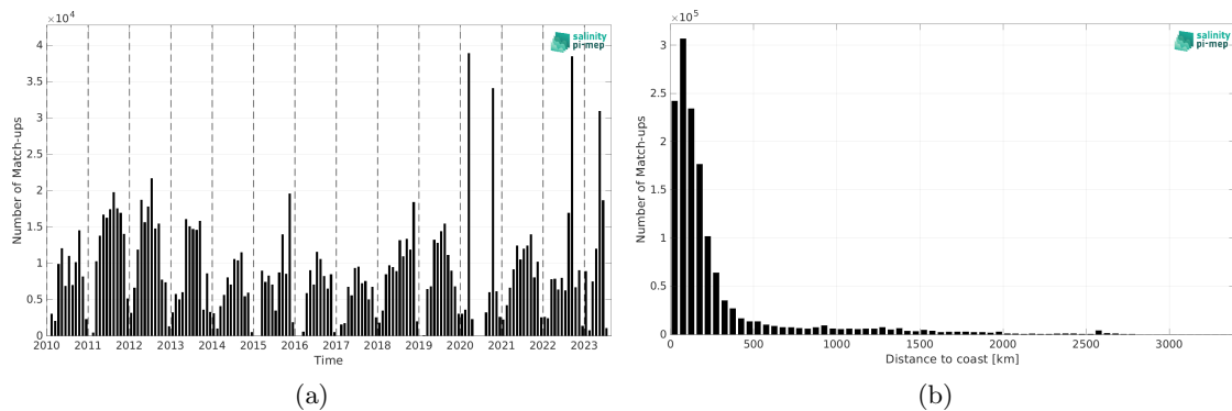
Figure 1: Number of match-ups between TSG (SAMOS) and SMOS SSS L4 v1 - Monthly (CMEMS-CNR) SSS as a function of time (a) and as function of the distance to coast (b) over the Atlantic Ocean Pi-MEP region and for the full satellite product period.
