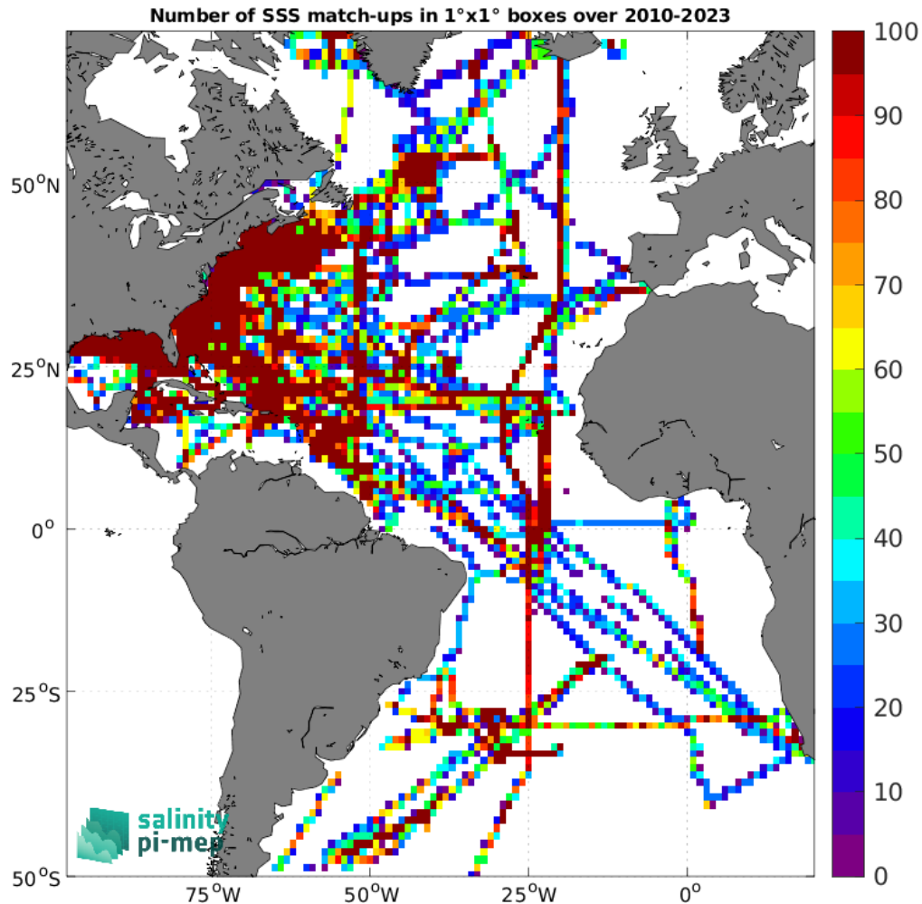
Figure 4: Number of SSS match-ups between TSG (SAMOS) SSS and the SMOS SSS L4 v1 - Monthly (CMEMS-CNR) SSS product for the Atlantic Ocean Pi-MEP region over 1^\circ \times 1^\circ boxes and for the full satellite product period.
