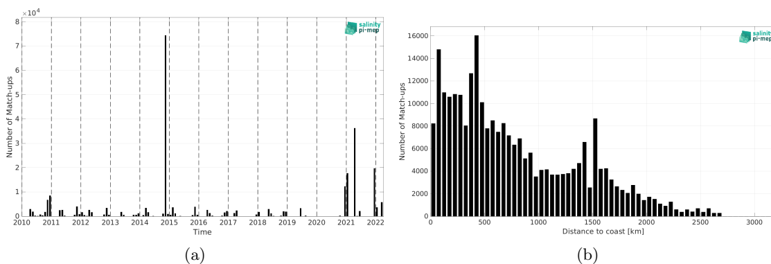
Figure 1: Number of match-ups between TSG (Polarstern) and SMOS SSS L4 v1 - Monthly (CMEMS-CNR) SSS as a function of time (a) and as function of the distance to coast (b) over the Atlantic Ocean Pi-MEP region and for the full satellite product period.
