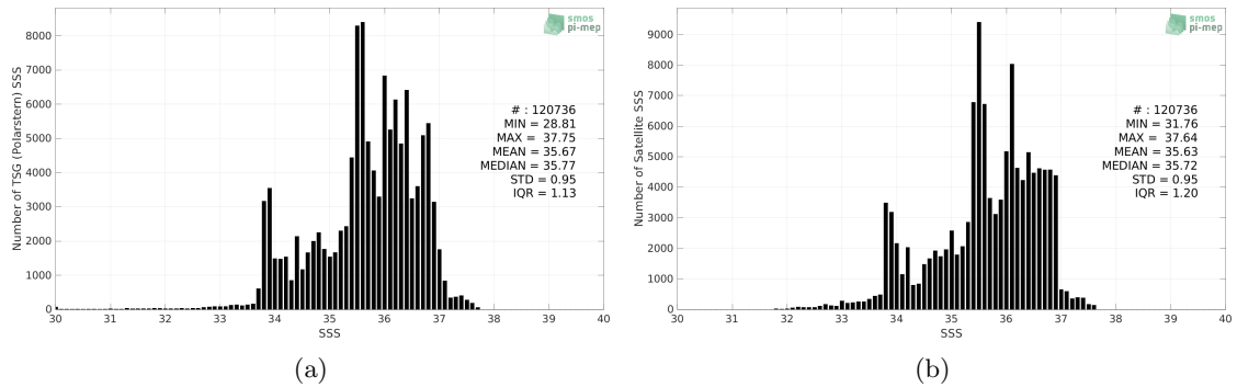
Figure 2: Histograms of SSS from TSG (Polarstern) (a) and SMOS SSS L4 v1 - Monthly (CMEMS-CNR) (b) considering all match-up pairs per bins of 0.1 over the Atlantic Ocean Pi-MEP region and for the full satellite product period.
