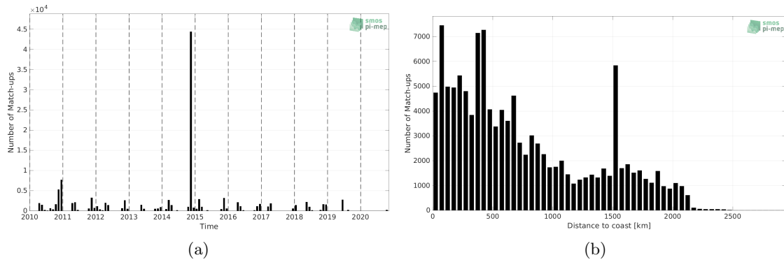
Figure 1: Number of match-ups between TSG (Polarstern) and SMOS SSS L4 v1 - Monthly (CMEMS-CNR) SSS as a function of time (a) and as function of the distance to coast (b) over the Atlantic Ocean Pi-MEP region and for the full satellite product period.
