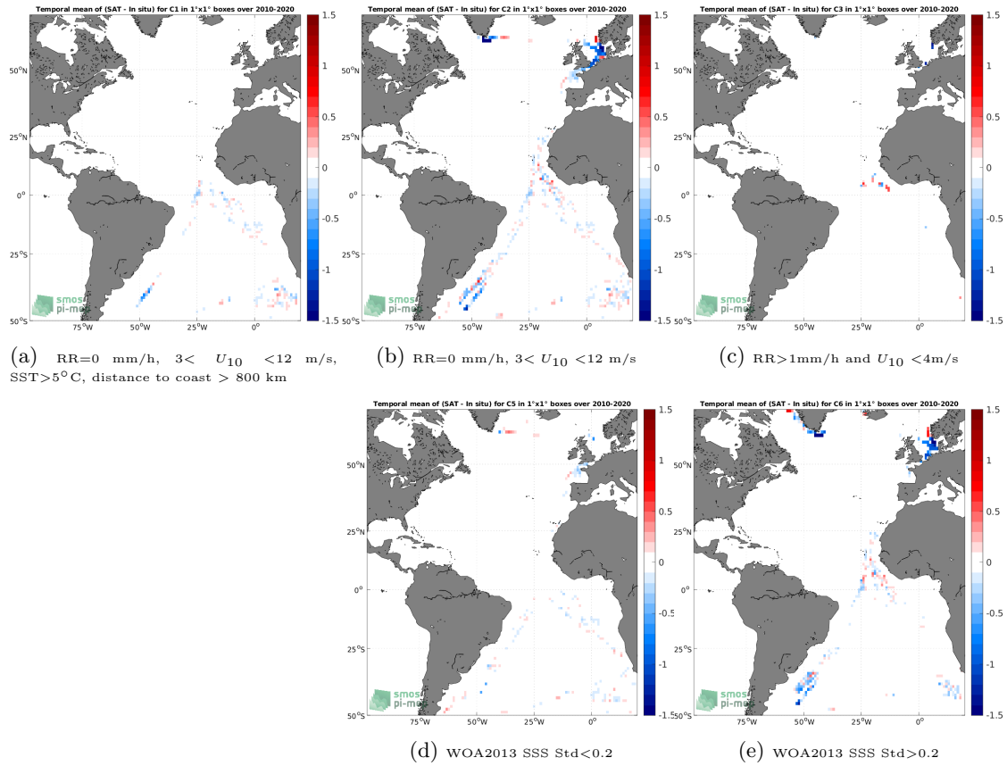
Figure 12: Temporal mean gridded over spatial boxes of size 1^\circ \times 1^\circ of \Delta SSS (SMOS SSS L4 v1 - Monthly (CMEMS-CNR) - TSG (Polarstern)) for 5 different subdatasets corresponding to:RR=0 mm/h, 3 < U_{10} < 12 m/s, SST >5^\circ C, distance to coast > 800 km (a), RR=0 mm/h, 3 < U_{10} < 12 m/s (b), RR >1 mm/h and U_{10} < 4 m/s (c), WOA2013 SSS Std <0.2 (d), WOA2013 SSS Std >0.2 (e).
