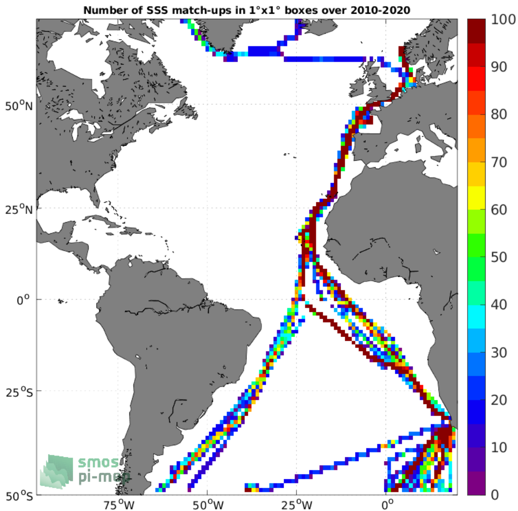
Figure 4: Number of SSS match-ups between TSG (Polarstern) SSS and the SMOS SSS L4 v1 - Monthly (CMEMS-CNR) SSS product for the Atlantic Ocean Pi-MEP region over 1^\circ \times 1^\circ boxes and for the full satellite product period.
