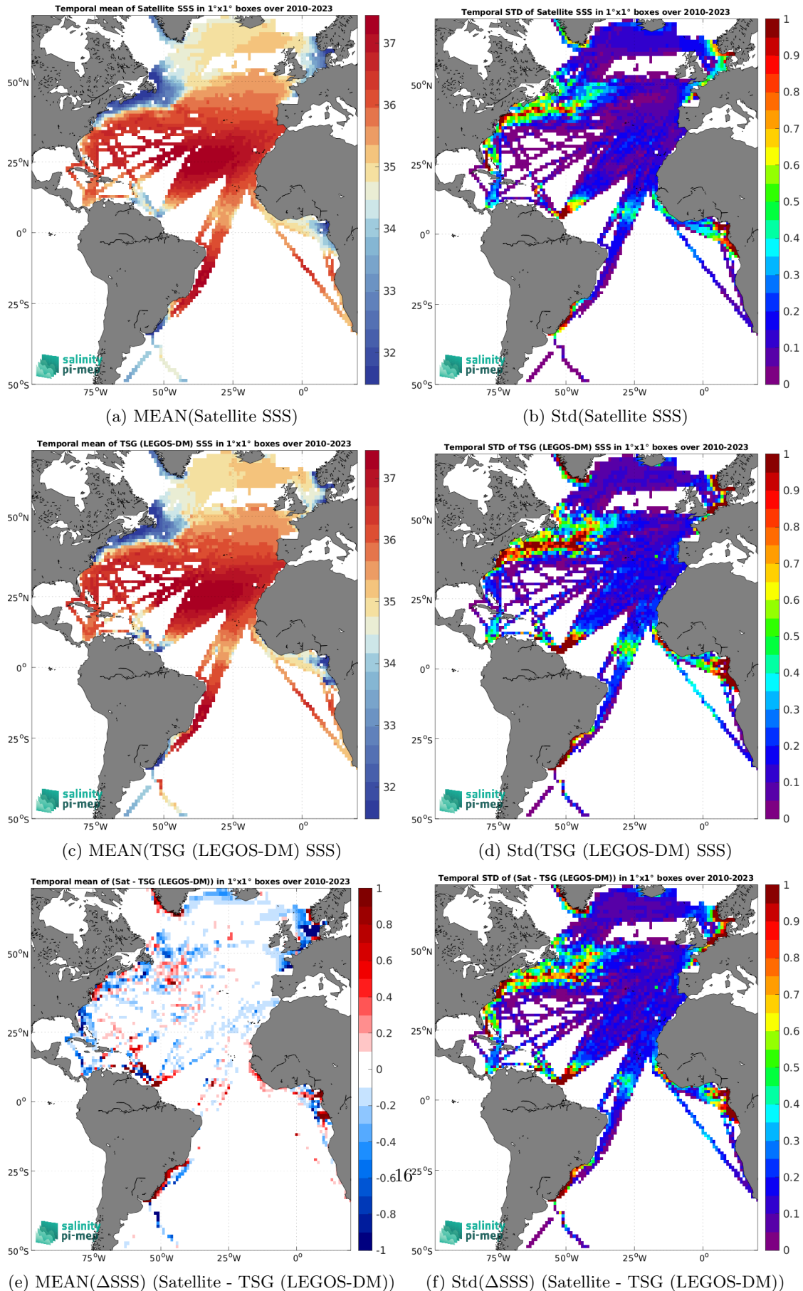
Figure 7: Temporal mean (left) and Std (right) of SSS from SMOS SSS L4 v1 - Monthly (CMEMS-CNR) (top), TSG (LEGOS-DM) (middle), and of \Delta SSS (Satellite - TSG (LEGOS-DM)). Only match-up pairs are used to generate these maps.
