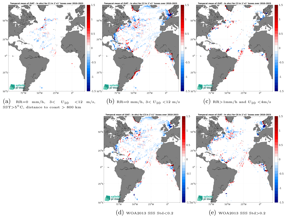
Figure 14: Temporal mean gridded over spatial boxes of size 1^\circ \times 1^\circ of \Delta\text{SSS} (SMOS SSS L4 v1 - Monthly (CMEMS-CNR) - TSG (LEGOS-DM)) for 5 different subdatasets corresponding to:RR=0 mm/h, 3 < U_{10} < 12 m/s, SST>5°C, distance to coast > 800 km (a), RR=0 mm/h, 3 < U_{10} < 12 m/s (b), RR>1mm/h and U_{10} < 4 m/s (c), WOA2013 SSS Std<0.2 (d), WOA2013 SSS Std>0.2 (e).
