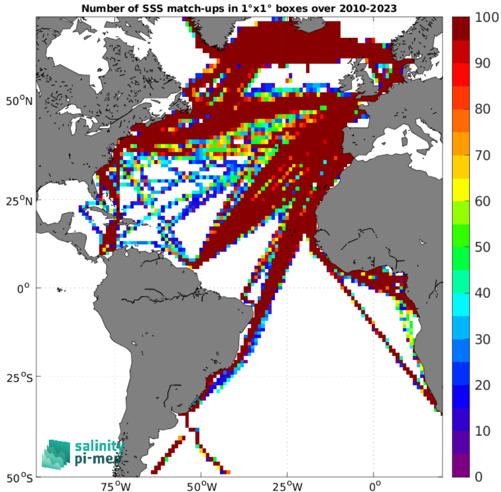
Figure 5: Number of SSS match-ups between TSG (LEGOS-DM) SSS and the SMOS SSS L4 v1 - Monthly (CMEMS-CNR) SSS product for the Atlantic Ocean Pi-MEP region over 1^\circ \times 1^\circ boxes and for the full satellite product period.
