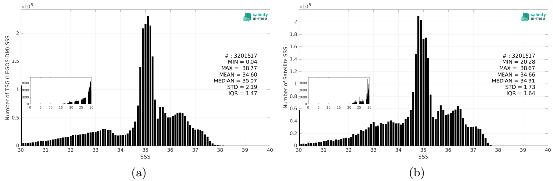
Figure 3: Histograms of SSS from TSG (LEGOS-DM) (a) and SMOS SSS L4 v1 - Monthly (CMEMS-CNR) (b) considering all match-up pairs per bins of 0.1 over the Atlantic Ocean Pi-MEP region and for the full satellite product period.
