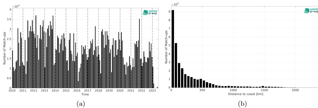
Figure 2: Number of match-ups between TSG (LEGOS-DM) and SMOS SSS L4 v1 - Monthly (CMEMS-CNR) SSS as a function of time (a) and as function of the distance to coast (b) over the Atlantic Ocean Pi-MEP region and for the full satellite product period.
