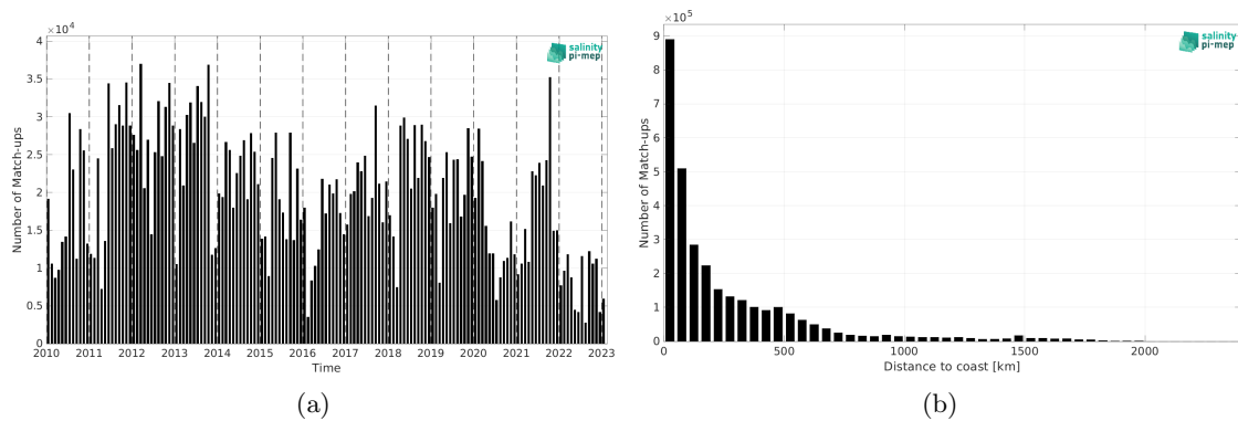
Figure 2: Number of match-ups between TSG (LEGOS-DM) and SMOS SSS L4 v1 - Monthly (CMEMS-CNR) SSS as a function of time (a) and as function of the distance to coast (b) over the Atlantic Ocean Pi-MEP region and for the full satellite product period.
