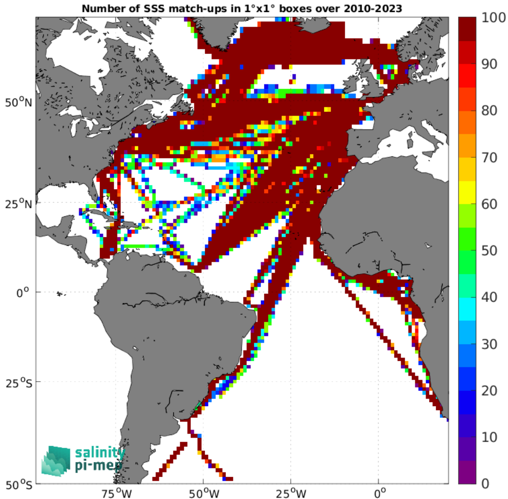
Figure 4: Number of SSS match-ups between TSG (LEGOS-DM) SSS and the SMOS SSS L4 v1 - Monthly (CMEMS-CNR) SSS product for the Atlantic Ocean Pi-MEP region over 1^\circ \times 1^\circ boxes and for the full satellite product period.
