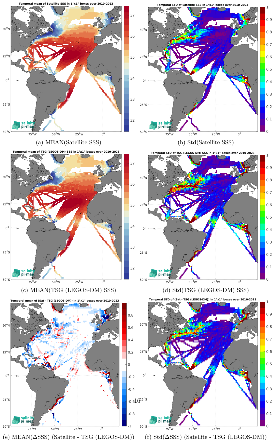
Figure 6: Temporal mean (left) and Std (right) of SSS from SMOS SSS L4 v1 - Monthly (CMEMS-CNR) (top), TSG (LEGOS-DM) (middle), and of \Delta SSS (Satellite - TSG (LEGOS-DM)). Only match-up pairs are used to generate these maps.
