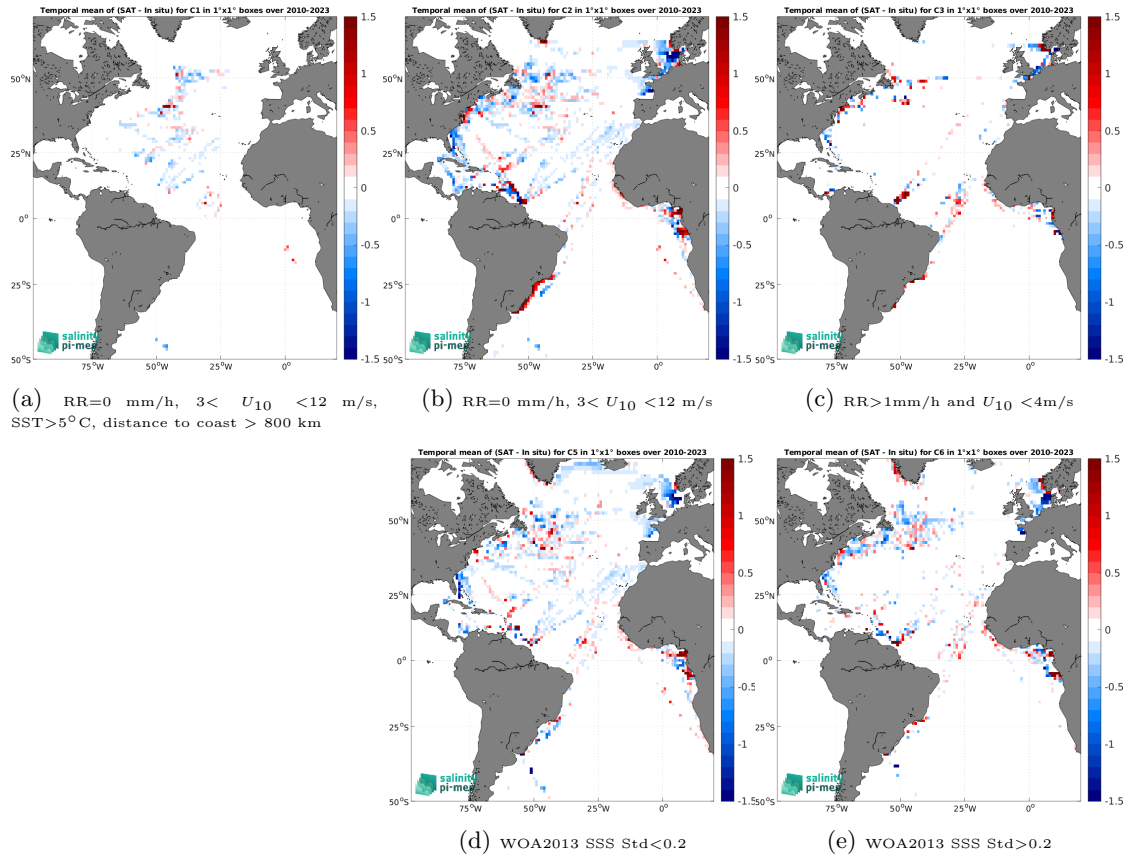
Figure 12: Temporal mean gridded over spatial boxes of size 1^\circ \times 1^\circ of \Delta\text{SSS} (SMOS SSS L4 v1 - Monthly (CMEMS-CNR) - TSG (LEGOS-DM)) for 5 different subdatasets corresponding to:RR=0 mm/h, 3 < U_{10} < 12 m/s, SST >5^\circ\text{C} , distance to coast > 800 km (a), RR=0 mm/h, 3 < U_{10} < 12 m/s (b), RR >1 mm/h and U_{10} < 4 m/s (c), WOA2013 SSS Std <0.2 (d), WOA2013 SSS Std >0.2 (e).
