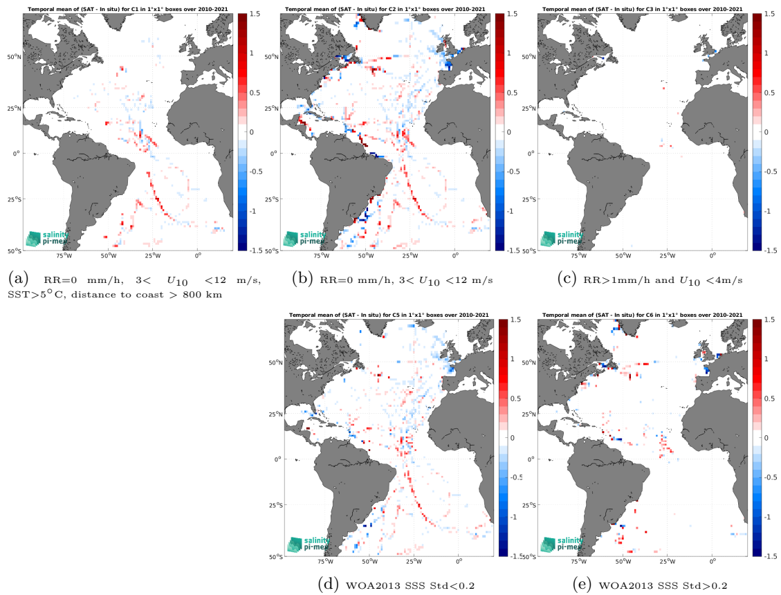
Figure 14: Temporal mean gridded over spatial boxes of size 1^\circ \times 1^\circ of \Delta\text{SSS} (SMOS SSS L4 v1 - Monthly (CMEMS-CNR) - TSG (GOSUD-Sailing-ship)) for 5 different subdatasets corresponding to:RR=0 mm/h, 3 < U_{10} < 12 m/s, SST >5^\circ\text{C} , distance to coast > 800 km (a), RR=0 mm/h, 3 < U_{10} < 12 m/s (b), RR >1 mm/h and U_{10} < 4 m/s (c), WOA2013 SSS Std <0.2 (d), WOA2013 SSS Std >0.2 (e).
