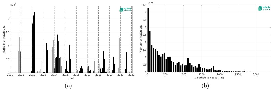
Figure 2: Number of match-ups between TSG (GOSUD-Sailing-ship) and SMOS SSS L4 v1 - Monthly (CMEMS-CNR) SSS as a function of time (a) and as function of the distance to coast (b) over the Atlantic Ocean Pi-MEP region and for the full satellite product period.
