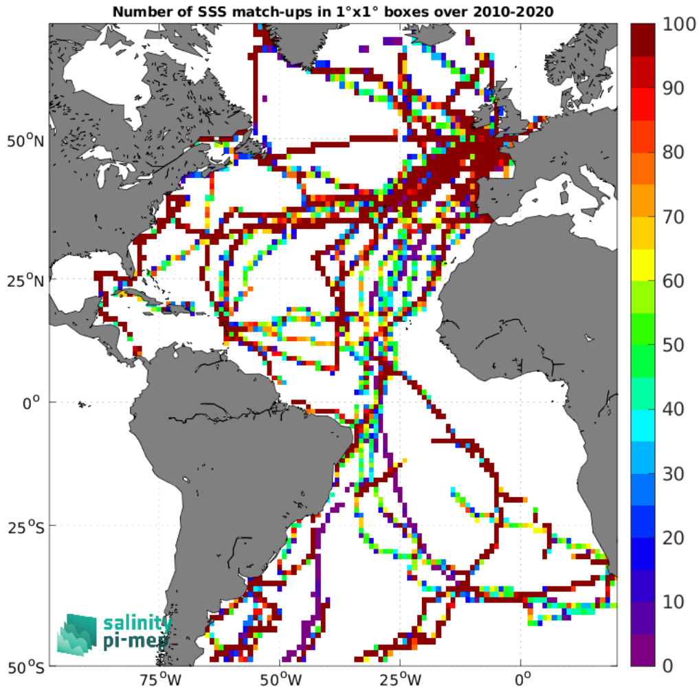
Figure 5: Number of SSS match-ups between TSG (GOSUD-Sailing-ship) SSS and the SMOS SSS L4 v1 - Monthly (CMEMS-CNR) SSS product for the Atlantic Ocean Pi-MEP region over 1^\circ \times 1^\circ boxes and for the full satellite product period.
