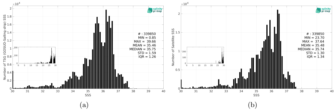
Figure 3: Histograms of SSS from TSG (GOSUD-Sailing-ship) (a) and SMOS SSS L4 v1 - Monthly (CMEMS-CNR) (b) considering all match-up pairs per bins of 0.1 over the Atlantic Ocean Pi-MEP region and for the full satellite product period.
