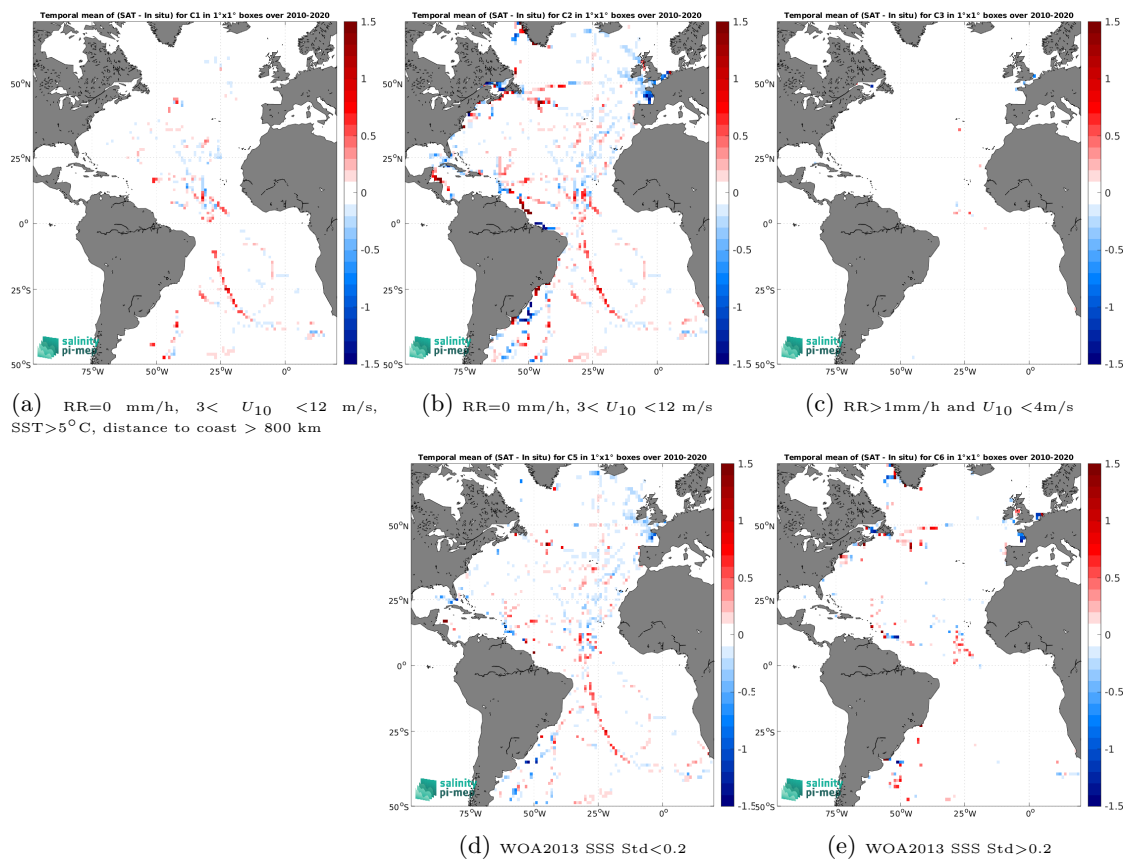
Figure 14: Temporal mean gridded over spatial boxes of size 1^\circ \times 1^\circ of \Delta SSS (SMOS SSS L4 v1 - Monthly (CMEMS-CNR) - TSG (GOSUD-Sailing-ship)) for 5 different subdatasets corresponding to:RR=0 mm/h, 3 < U_{10} < 12 m/s, SST >5^\circ\text{C} , distance to coast > 800 km (a), RR=0 mm/h, 3 < U_{10} < 12 m/s (b), RR >1 mm/h and U_{10} < 4 m/s (c), WOA2013 SSS Std <0.2 (d), WOA2013 SSS Std >0.2 (e).
