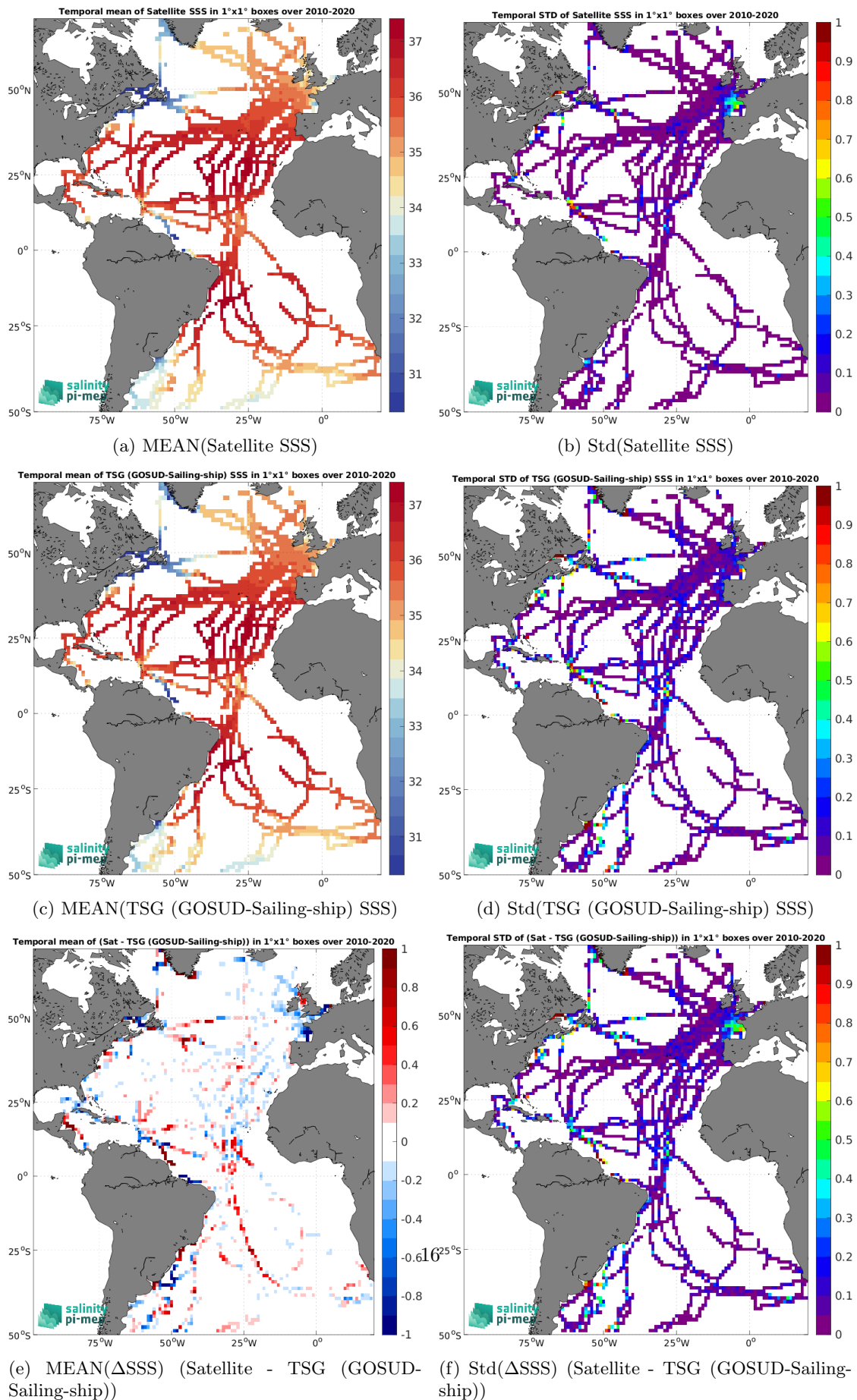
Figure 7: Temporal mean (left) and Std (right) of SSS from SMOS SSS L4 v1 - Monthly (CMEMS-CNR) (top), TSG (GOSUD-Sailing-ship) (middle), and of \Delta SSS (Satellite - TSG (GOSUD-Sailing-ship)). Only match-up pairs are used to generate these maps.
