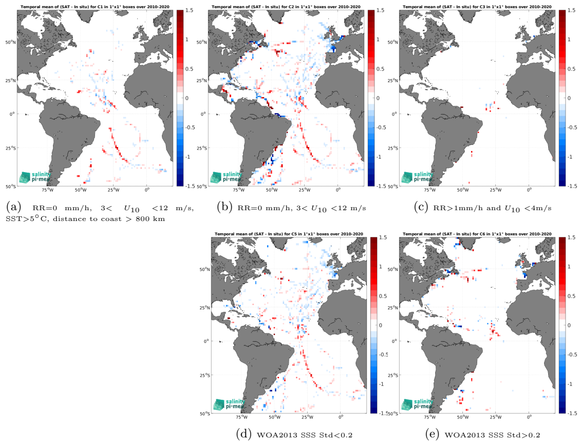
Figure 12: Temporal mean gridded over spatial boxes of size 1^\circ \times 1^\circ of \Delta SSS (SMOS SSS L4 v1 - Monthly (CMEMS-CNR) - TSG (GOSUD-Sailing-ship)) for 5 different subdatasets corresponding to:RR=0 mm/h, 3 < U_{10} < 12 m/s, SST >5^\circ\text{C} , distance to coast > 800 km (a), RR=0 mm/h, 3 < U_{10} < 12 m/s (b), RR >1 mm/h and U_{10} < 4 m/s (c), WOA2013 SSS Std <0.2 (d), WOA2013 SSS Std >0.2 (e).
