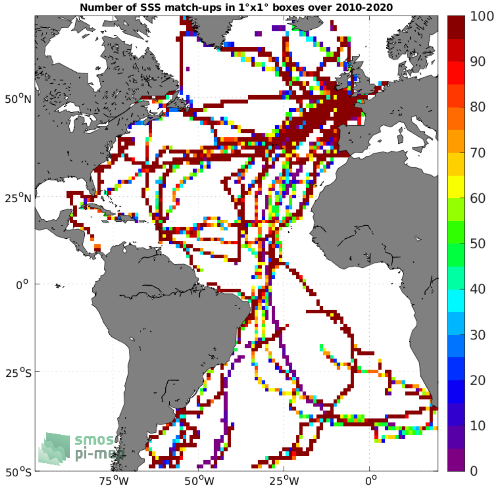
Figure 4: Number of SSS match-ups between TSG (GOSUD-Sailing-ship) SSS and the SMOS SSS L4 v1 - Monthly (CMEMS-CNR) SSS product for the Atlantic Ocean Pi-MEP region over 1^\circ \times 1^\circ boxes and for the full satellite product period.
