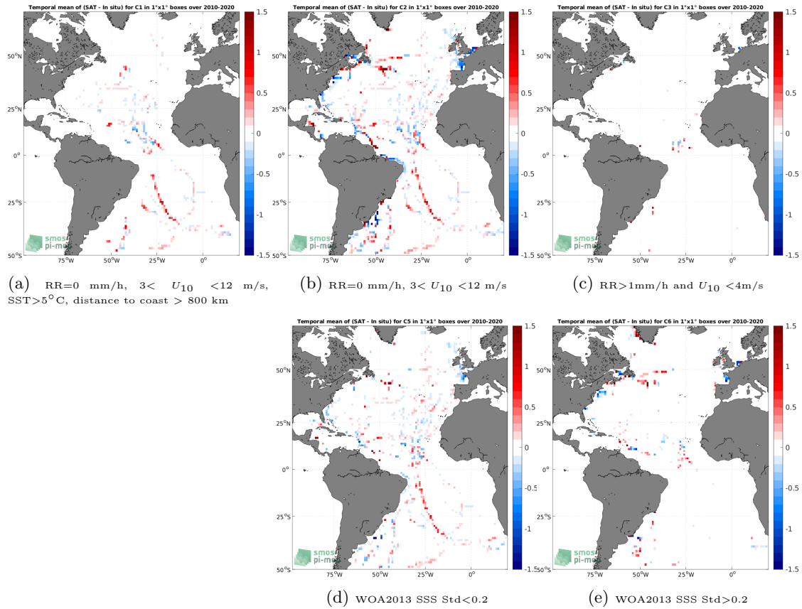
Figure 12: Temporal mean gridded over spatial boxes of size 1^\circ \times 1^\circ of \Delta\text{SSS} (SMOS SSS L4 v1 - Monthly (CMEMS-CNR) - TSG (GOSUD-Sailing-ship)) for 5 different subdatasets corresponding to:RR=0 mm/h, 3 < U_{10} < 12 m/s, SST >5^\circ\text{C} , distance to coast > 800 km (a), RR=0 mm/h, 3 < U_{10} < 12 m/s (b), RR >1 mm/h and U_{10} < 4 m/s (c), WOA2013 SSS Std <0.2 (d), WOA2013 SSS Std >0.2 (e).
