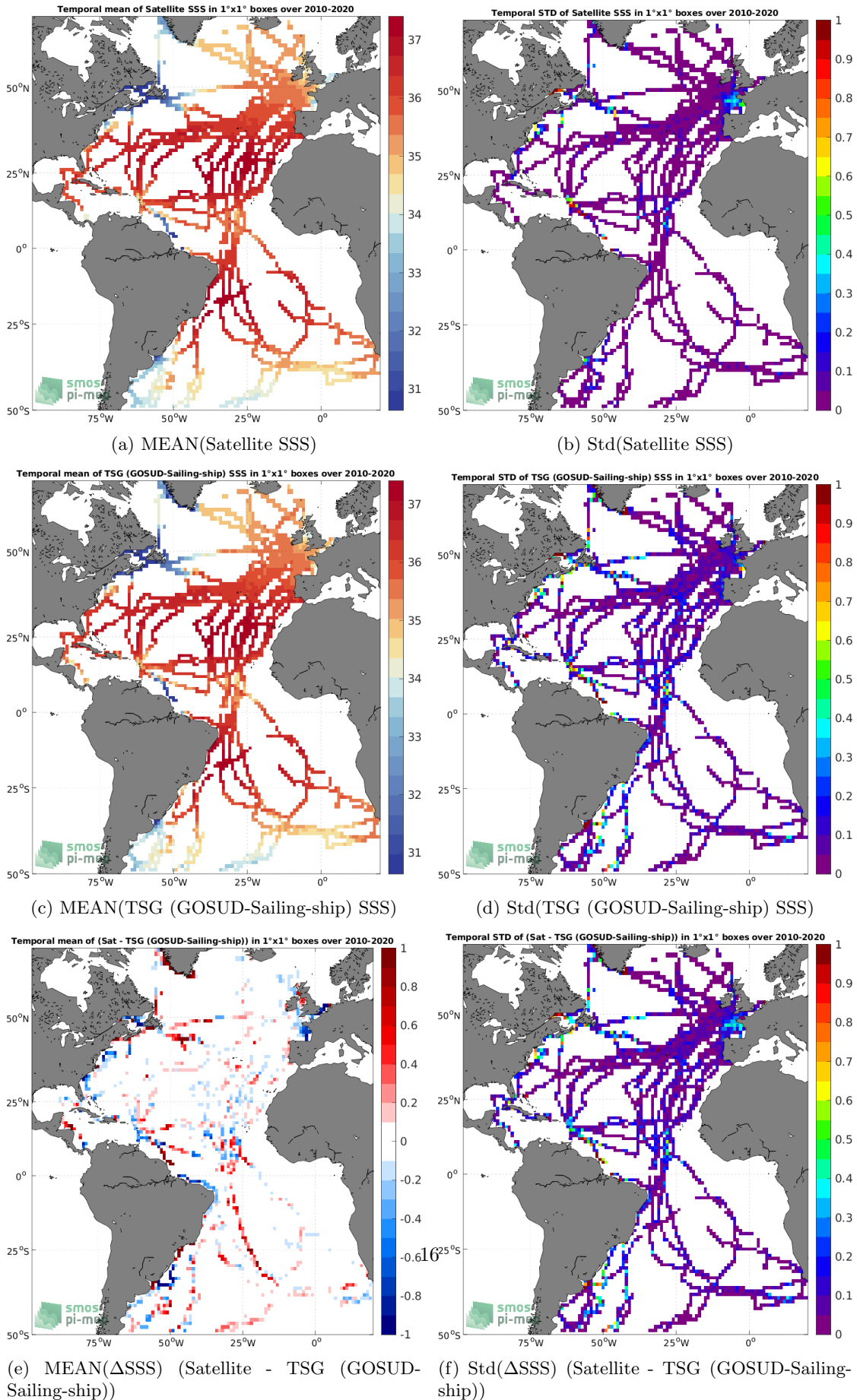
Figure 6: Temporal mean (left) and Std (right) of SSS from SMOS SSS L4 v1 - Monthly (CMEMS-CNR) (top), TSG (GOSUD-Sailing-ship) (middle), and of \Delta SSS (Satellite - TSG (GOSUD-Sailing-ship)). Only match-up pairs are used to generate these maps.
