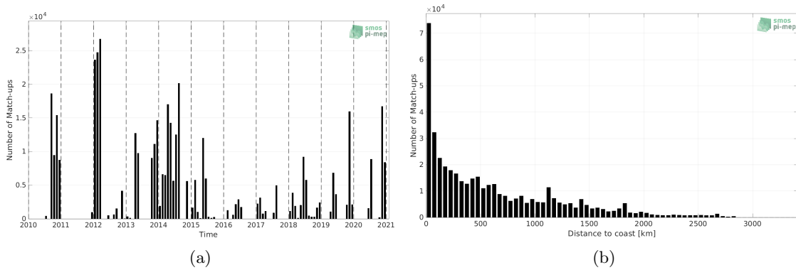
Figure 1: Number of match-ups between TSG (GOSUD-Sailing-ship) and SMOS SSS L4 v1 - Monthly (CMEMS-CNR) SSS as a function of time (a) and as function of the distance to coast (b) over the Atlantic Ocean Pi-MEP region and for the full satellite product period.
