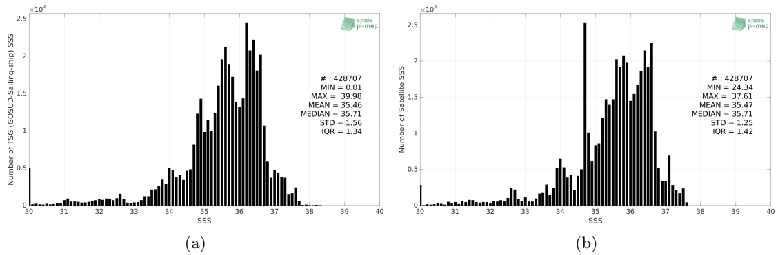
Figure 2: Histograms of SSS from TSG (GOSUD-Sailing-ship) (a) and SMOS SSS L4 v1 - Monthly (CMEMS-CNR) (b) considering all match-up pairs per bins of 0.1 over the Atlantic Ocean Pi-MEP region and for the full satellite product period.
