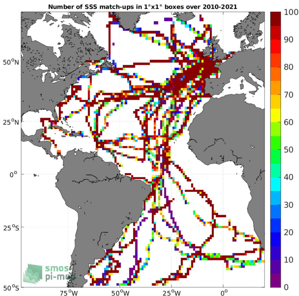
Figure 4: Number of SSS match-ups between TSG (GOSUD-Sailing-ship) SSS and the SMOS SSS L4 v1 - Monthly (CMEMS-CNR) SSS product for the Atlantic Ocean Pi-MEP region over 1°x1° boxes and for the full satellite product period.
