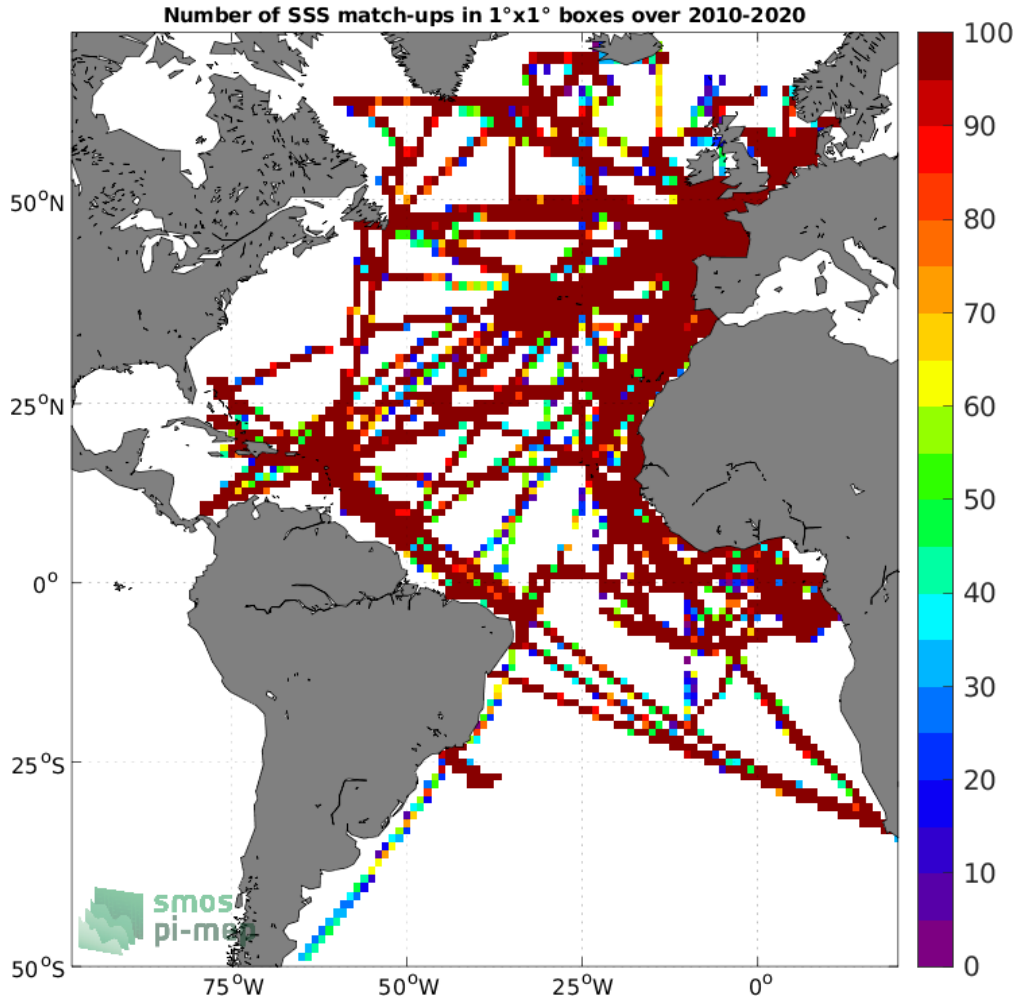
Figure 4: Number of SSS match-ups between TSG (GOSUD-Research-vessel) SSS and the SMOS SSS L4 v1 - Monthly (CMEMS-CNR) SSS product for the Atlantic Ocean Pi-MEP region over 1^\circ \times 1^\circ boxes and for the full satellite product period.
