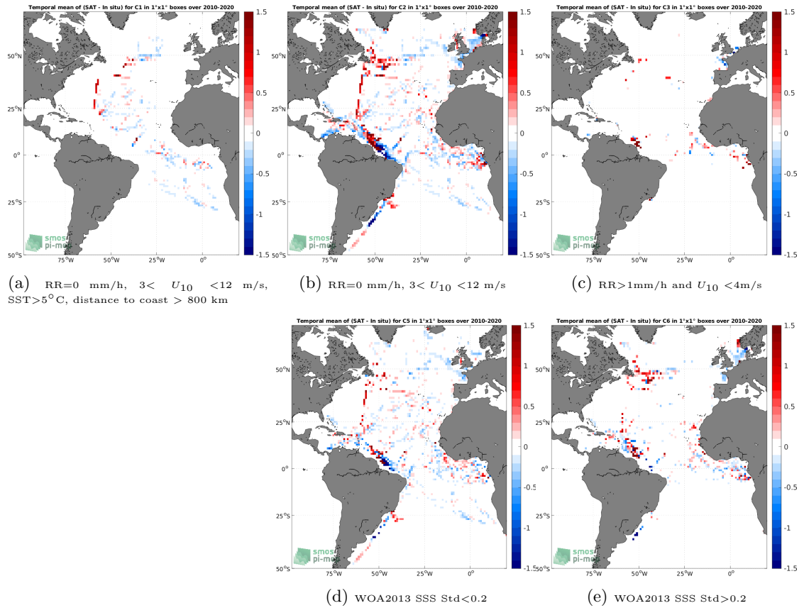
Figure 12: Temporal mean gridded over spatial boxes of size 1^\circ \times 1^\circ of \Delta\text{SSS} (SMOS SSS L4 v1 - Monthly (CMEMS-CNR) - TSG (GOSUD-Research-vessel)) for 5 different subdatasets corresponding to:RR=0 mm/h, 3 < U_{10} < 12 m/s, SST >5^\circ\text{C} , distance to coast > 800 km (a), RR=0 mm/h, 3 < U_{10} < 12 m/s (b), RR >1 mm/h and U_{10} < 4 m/s (c), WOA2013 SSS Std <0.2 (d), WOA2013 SSS Std >0.2 (e).
