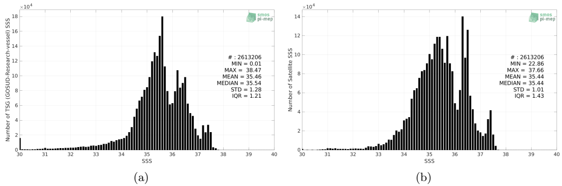
Figure 2: Histograms of SSS from TSG (GOSUD-Research-vessel) (a) and SMOS SSS L4 v1 - Monthly (CMEMS-CNR) (b) considering all match-up pairs per bins of 0.1 over the Atlantic Ocean Pi-MEP region and for the full satellite product period.
