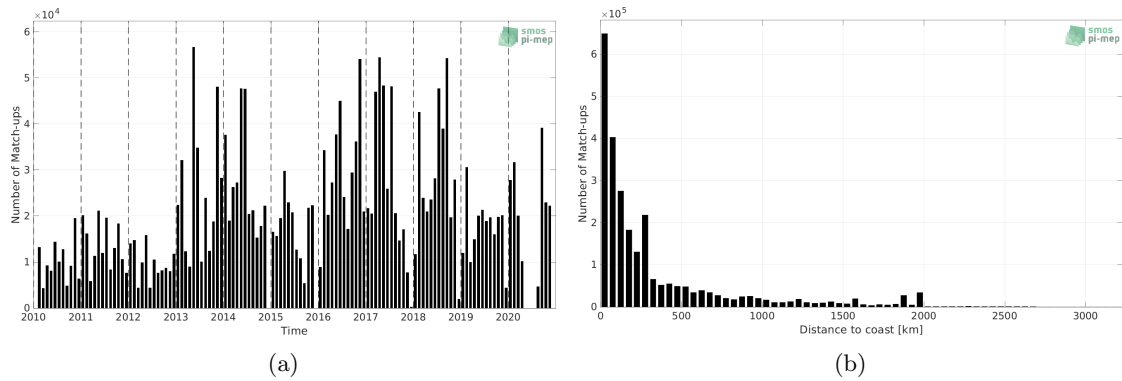
Figure 1: Number of match-ups between TSG (GOSUD-Research-vessel) and SMOS SSS L4 v1 - Monthly (CMEMS-CNR) SSS as a function of time (a) and as function of the distance to coast (b) over the Atlantic Ocean Pi-MEP region and for the full satellite product period.
