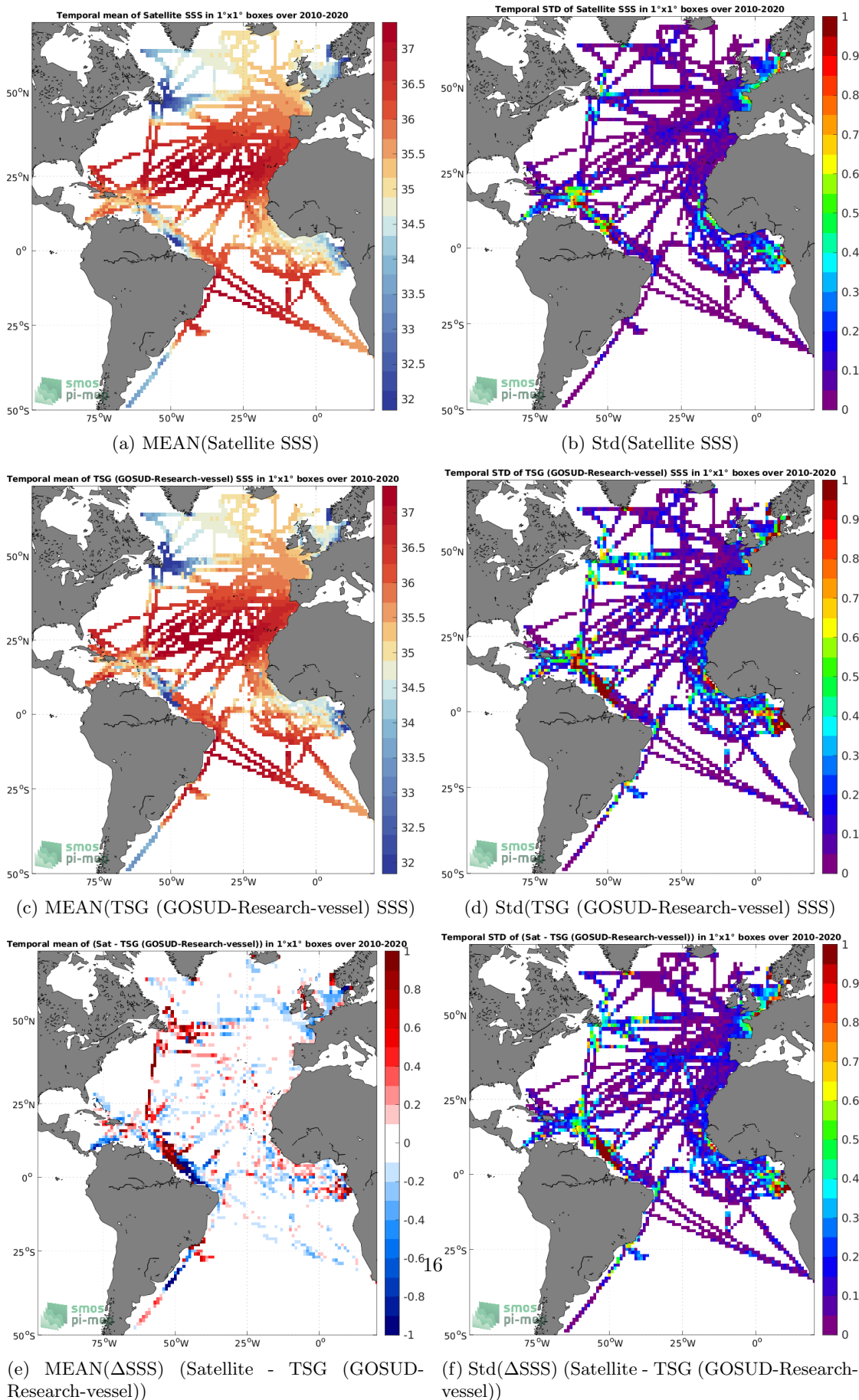
Figure 6: Temporal mean (left) and Std (right) of SSS from SMOS SSS L4 v1 - Monthly (CMEMS-CNR) (top), TSG (GOSUD-Research-vessel) (middle), and of \Delta SSS (Satellite - TSG (GOSUD-Research-vessel)). Only match-up pairs are used to generate these maps.
