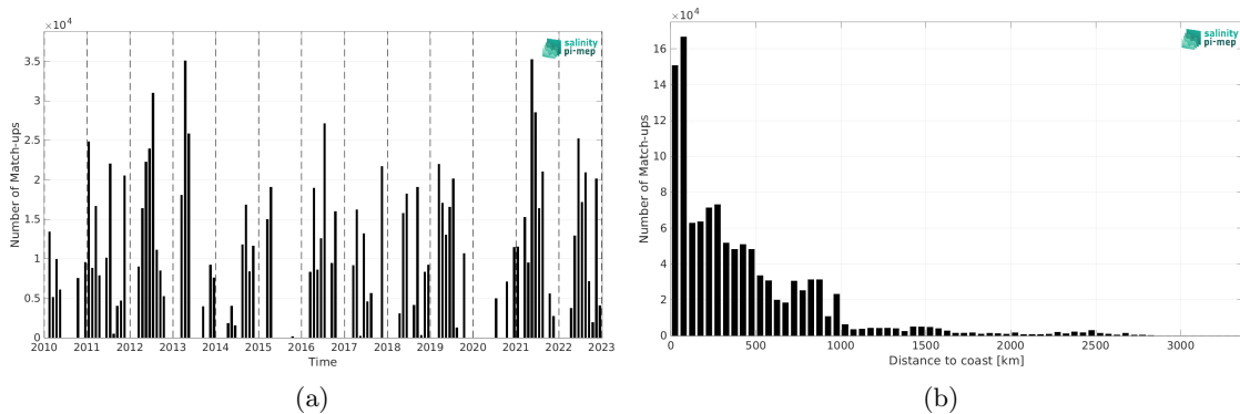
Figure 2: Number of match-ups between TSG (CSIC-UTM) and SMOS SSS L4 v1 - Monthly (CMEMS-CNR) SSS as a function of time (a) and as function of the distance to coast (b) over the Atlantic Ocean Pi-MEP region and for the full satellite product period.
