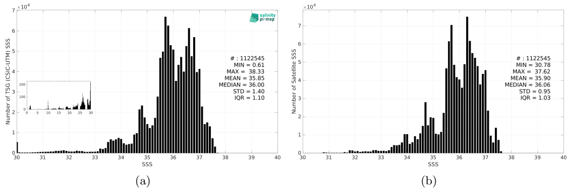
Figure 3: Histograms of SSS from TSG (CSIC-UTM) (a) and SMOS SSS L4 v1 - Monthly (CMEMS-CNR) (b) considering all match-up pairs per bins of 0.1 over the Atlantic Ocean Pi-MEP region and for the full satellite product period.
