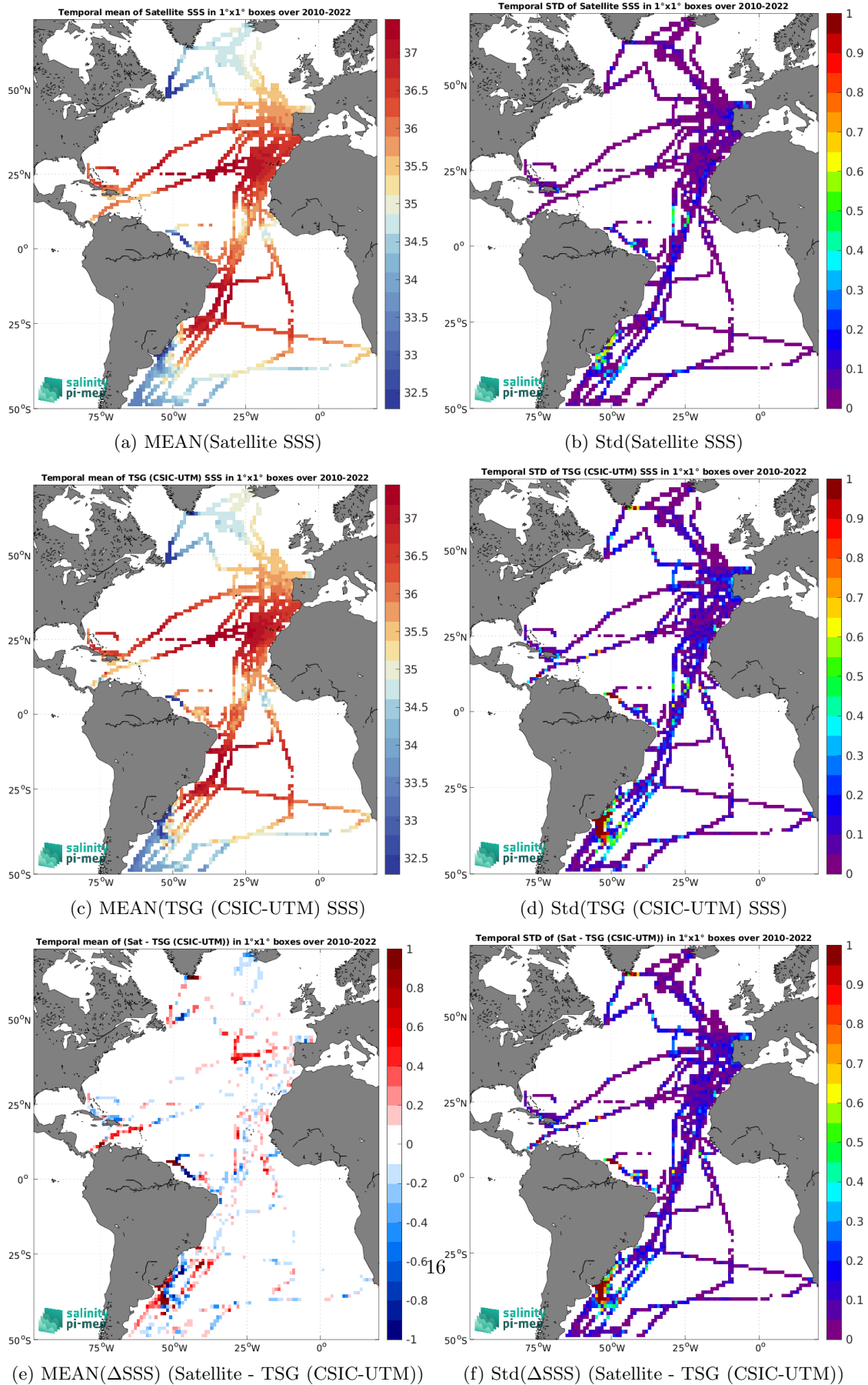
Figure 7: Temporal mean (left) and Std (right) of SSS from SMOS SSS L4 v1 - Monthly (CMEMS-CNR) (top), TSG (CSIC-UTM) (middle), and of \Delta SSS (Satellite - TSG (CSIC-UTM)). Only match-up pairs are used to generate these maps.
