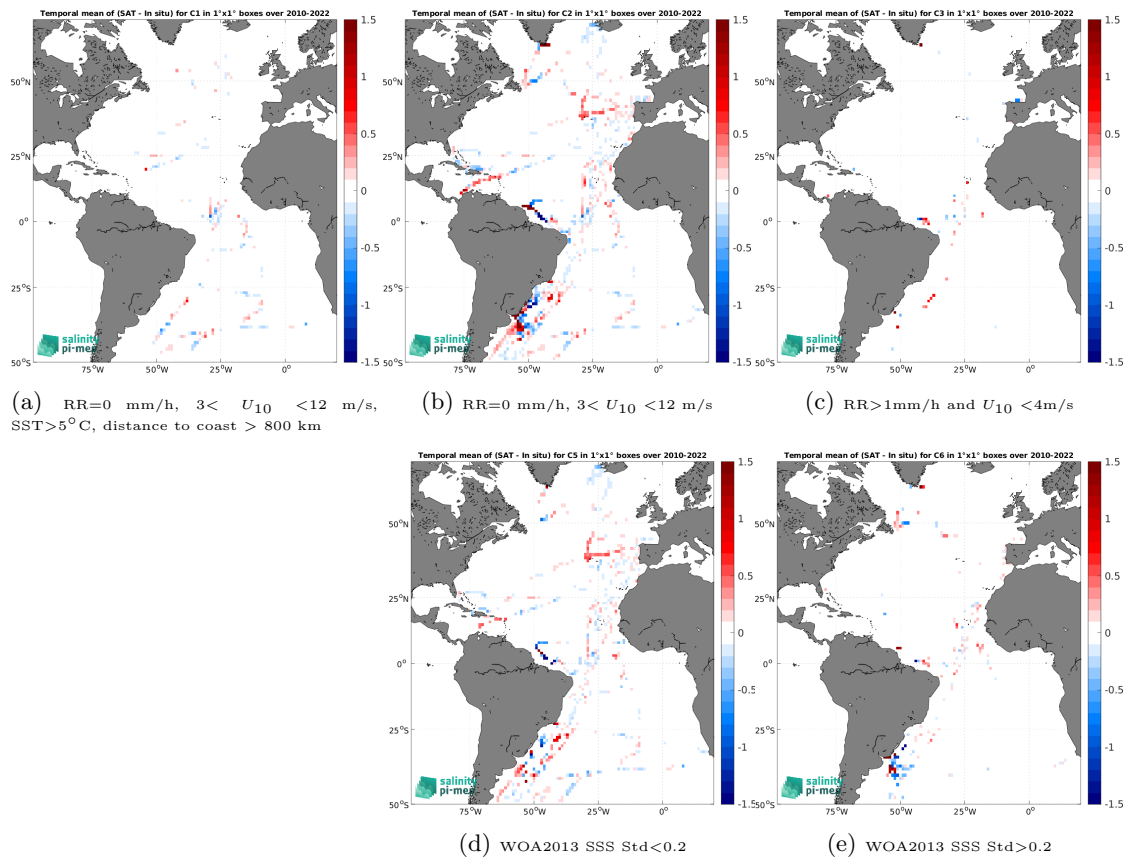
Figure 14: Temporal mean gridded over spatial boxes of size 1^\circ \times 1^\circ of \Delta\text{SSS} (SMOS SSS L4 v1 - Monthly (CMEMS-CNR) - TSG (CSIC-UTM)) for 5 different subdatasets corresponding to:RR=0 mm/h, 3 < U_{10} < 12 m/s, SST>5°C, distance to coast > 800 km (a), RR=0 mm/h, 3 < U_{10} < 12 m/s (b), RR>1mm/h and U_{10} < 4 m/s (c), WOA2013 SSS Std<0.2 (d), WOA2013 SSS Std>0.2 (e).
