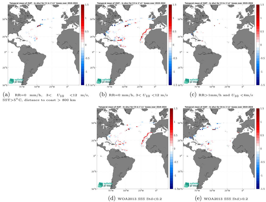
Figure 14: Temporal mean gridded over spatial boxes of size 1^\circ \times 1^\circ of \Delta SSS (SMOS SSS L4 v1 - Monthly (CMEMS-CNR) - Saildrone) for 5 different subdatasets corresponding to:RR=0 mm/h, 3 < U_{10} < 12 m/s, SST >5^\circ\text{C} , distance to coast > 800 km (a), RR=0 mm/h, 3 < U_{10} < 12 m/s (b), RR >1 mm/h and U_{10} < 4 m/s (c), WOA2013 SSS Std <0.2 (d), WOA2013 SSS Std >0.2 (e).
