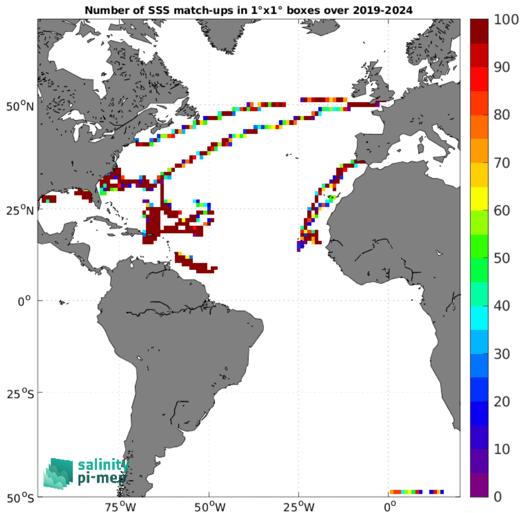
Figure 5: Number of SSS match-ups between Saildrone SSS and the SMOS SSS L4 v1 - Monthly (CMEMS-CNR) SSS product for the Atlantic Ocean Pi-MEP region over 1^\circ \times 1^\circ boxes and for the full satellite product period.
