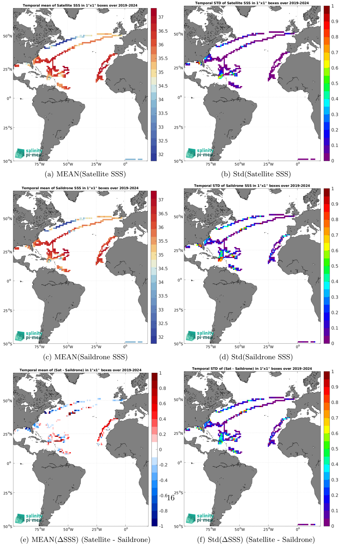
Figure 7: Temporal mean (left) and Std (right) of SSS from SMOS SSS L4 v1 - Monthly (CMEMS-CNR) (top), Saildrone (middle), and of \Delta SSS (Satellite - Saildrone). Only match-up pairs are used to generate these maps.
