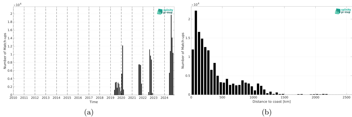
Figure 2: Number of match-ups between Saildrone and SMOS SSS L4 v1 - Monthly (CMEMS-CNR) SSS as a function of time (a) and as function of the distance to coast (b) over the Atlantic Ocean Pi-MEP region and for the full satellite product period.
