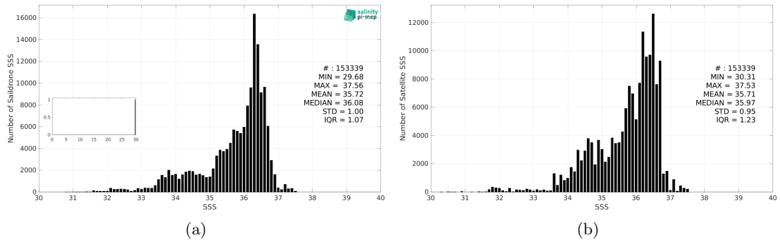
Figure 3: Histograms of SSS from Saildrone (a) and SMOS SSS L4 v1 - Monthly (CMEMS-CNR) (b) considering all match-up pairs per bins of 0.1 over the Atlantic Ocean Pi-MEP region and for the full satellite product period.
