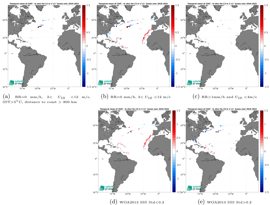
Figure 14: Temporal mean gridded over spatial boxes of size 1^\circ \times 1^\circ of \Delta\text{SSS} (SMOS SSS L4 v1 - Monthly (CMEMS-CNR) - Saildrone) for 5 different subdatasets corresponding to:RR=0 mm/h, 3 < U_{10} < 12 m/s, SST >5^\circ\text{C} , distance to coast > 800 km (a), RR=0 mm/h, 3 < U_{10} < 12 m/s (b), RR >1 mm/h and U_{10} < 4 m/s (c), WOA2013 SSS Std <0.2 (d), WOA2013 SSS Std >0.2 (e).
