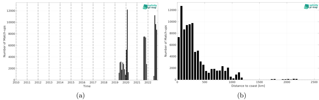
Figure 2: Number of match-ups between Saildrone and SMOS SSS L4 v1 - Monthly (CMEMS-CNR) SSS as a function of time (a) and as function of the distance to coast (b) over the Atlantic Ocean Pi-MEP region and for the full satellite product period.
