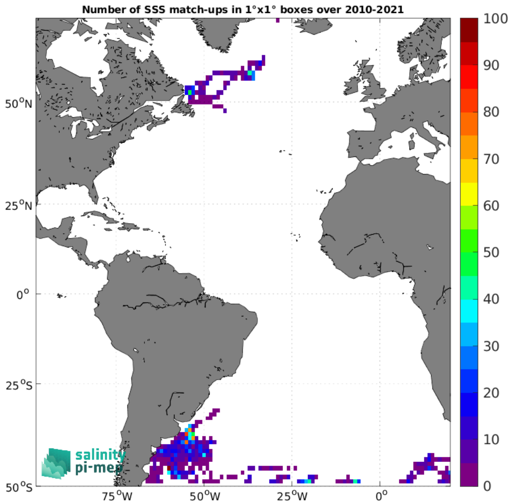
Figure 5: Number of SSS match-ups between Marine mammals SSS and the SMOS SSS L4 v1 - Monthly (CMEMS-CNR) SSS product for the Atlantic Ocean Pi-MEP region over 1°×1° boxes and for the full satellite product period.
