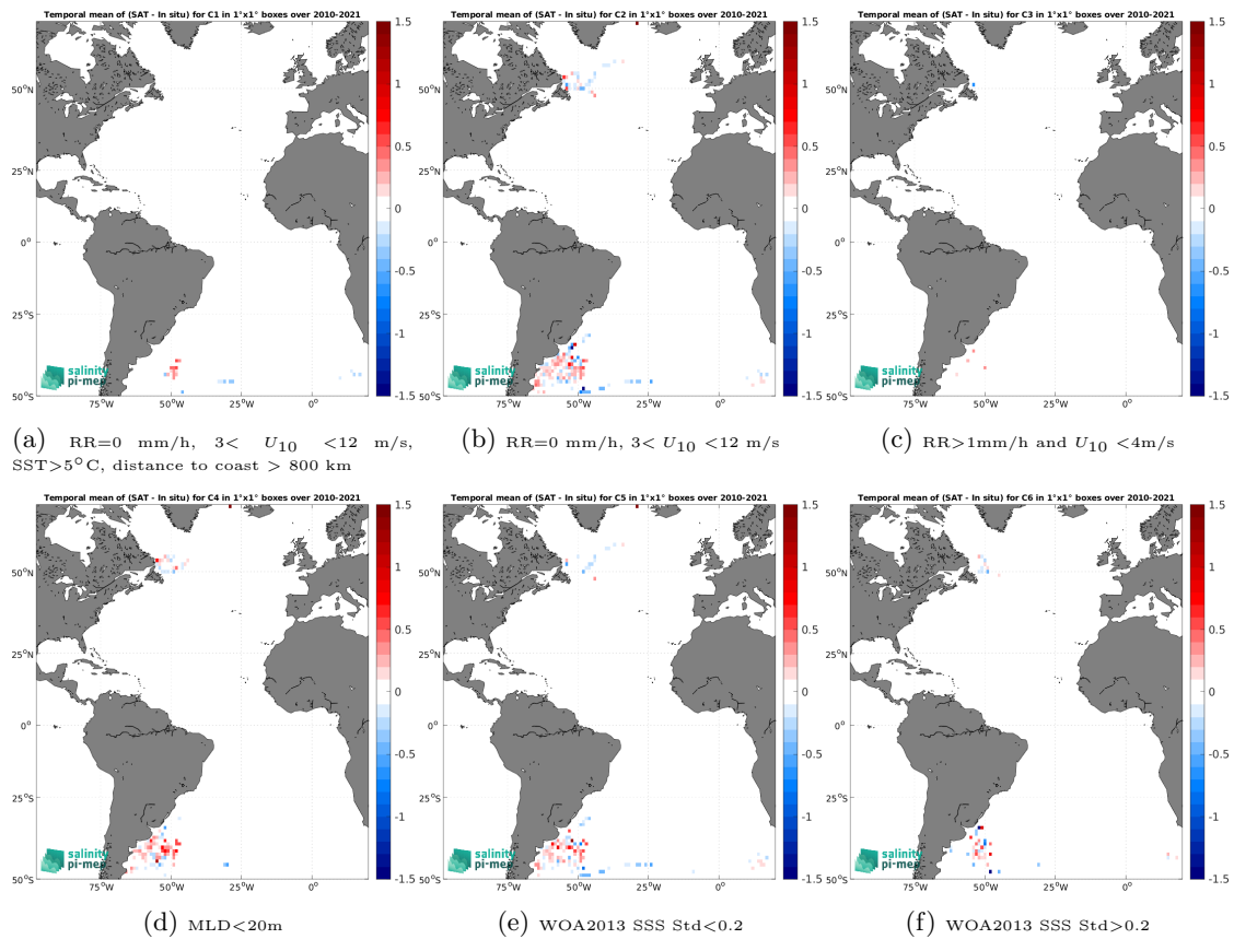
Figure 14: Temporal mean gridded over spatial boxes of size 1^\circ \times 1^\circ of \Delta SSS (SMOS SSS L4 v1 - Monthly (CMEMS-CNR) - Marine mammals) for 6 different subdatasets corresponding to:RR=0 mm/h, 3 < U_{10} < 12 m/s, SST > 5^\circ\text{C} , distance to coast > 800 km (a), RR=0 mm/h, 3 < U_{10} < 12 m/s (b), RR > 1 mm/h and U_{10} < 4 m/s (c),MLD < 20 m (d),WOA2013 SSS Std < 0.2 (e),WOA2013 SSS Std > 0.2 (f).
