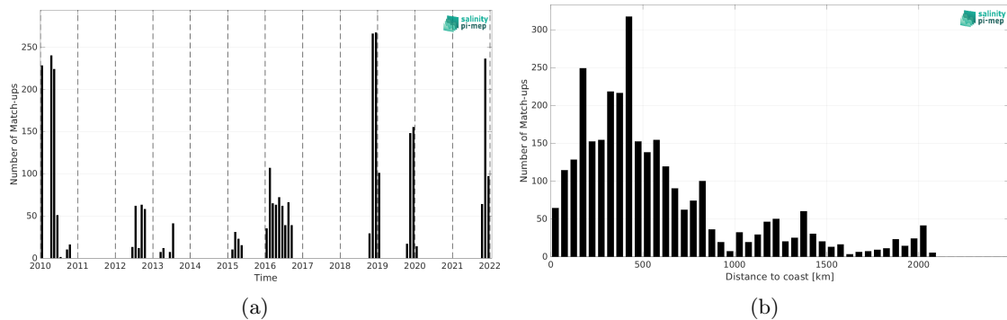
Figure 2: Number of match-ups between Marine mammals and SMOS SSS L4 v1 - Monthly (CMEMS-CNR) SSS as a function of time (a) and as function of the distance to coast (b) over the Atlantic Ocean Pi-MEP region and for the full satellite product period.
