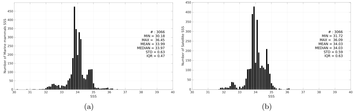
Figure 3: Histograms of SSS from Marine mammals (a) and SMOS SSS L4 v1 - Monthly (CMEMS-CNR) (b) considering all match-up pairs per bins of 0.1 over the Atlantic Ocean Pi-MEP region and for the full satellite product period.
