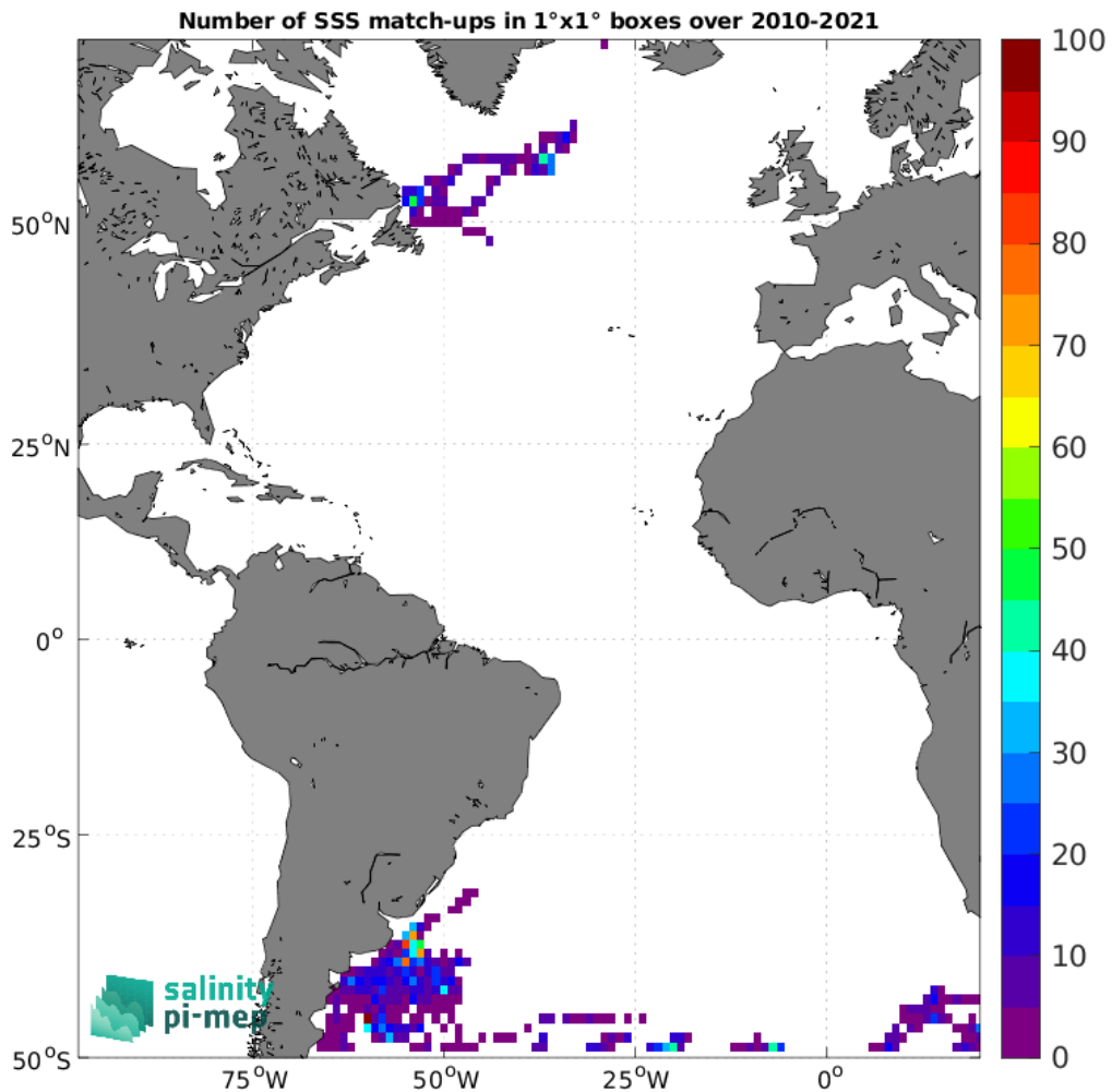
Figure 5: Number of SSS match-ups between Marine mammals SSS and the SMOS SSS L4 v1 - Monthly (CMEMS-CNR) SSS product for the Atlantic Ocean Pi-MEP region over 1^\circ \times 1^\circ boxes and for the full satellite product period.
