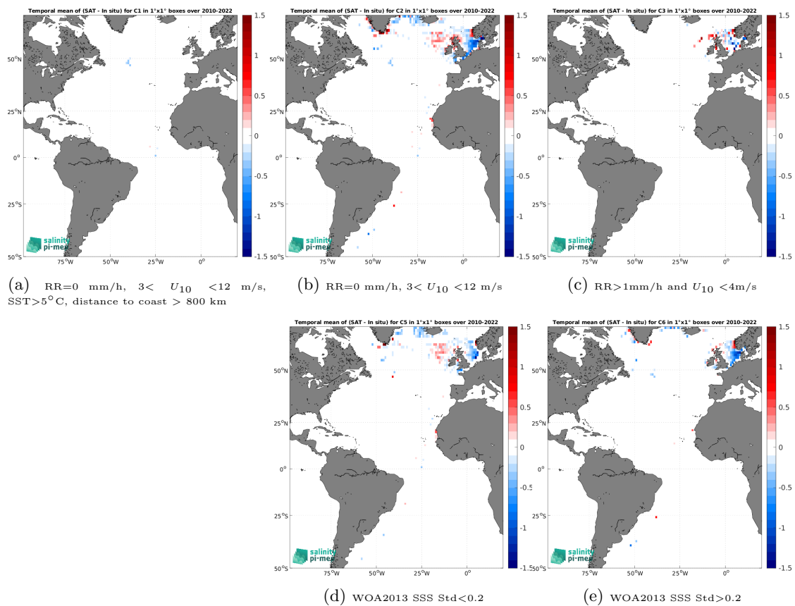
Figure 14: Temporal mean gridded over spatial boxes of size 1^\circ \times 1^\circ of \Delta\text{SSS} (SMOS SSS L4 v1 - Monthly (CMEMS-CNR) - ICES) for 5 different subdatasets corresponding to:RR=0 mm/h, 3 < U_{10} < 12 m/s, SST>5°C, distance to coast > 800 km (a), RR=0 mm/h, 3 < U_{10} < 12 m/s (b), RR>1mm/h and U_{10} < 4 m/s (c), WOA2013 SSS Std<0.2 (d), WOA2013 SSS Std>0.2 (e).
