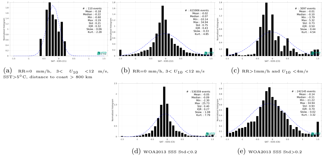
Figure 15: Normalized histogram of \Delta SSS (SMOS SSS L4 v1 - Monthly (CMEMS-CNR) - ICES) for 5 different subdatasets corresponding to: RR=0 mm/h, 3 < U_{10} < 12 m/s, SST > 5°C, distance to coast > 800 km (a), RR=0 mm/h, 3 < U_{10} < 12 m/s (b), RR > 1mm/h and U_{10} < 4 m/s (c), WOA2013 SSS Std < 0.2 (d), WOA2013 SSS Std > 0.2 (e).
