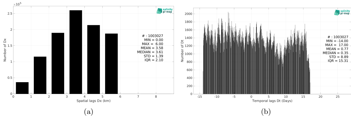
Figure 6: Histograms of the spatial (a) and temporal (b) lags between the location/time of the ICES measurement and the date of the corresponding SMOS SSS L4 v1 - Monthly (CMEMS-CNR) SSS pixel.
