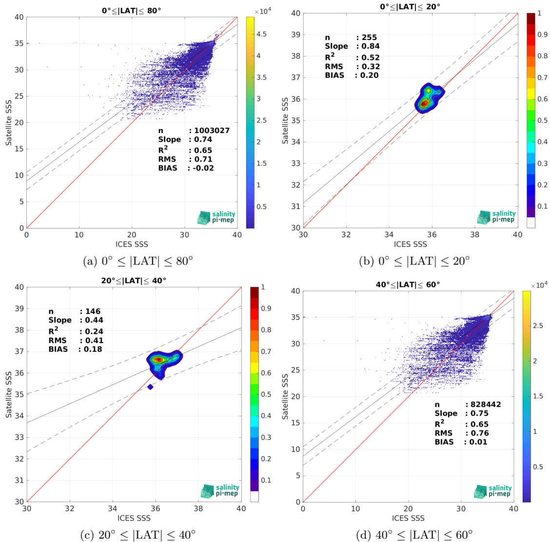
Figure 10: Contour maps of the concentration of SMOS SSS L4 v1 - Monthly (CMEMS-CNR) SSS (y-axis) versus ICES SSS (x-axis) at match-up pairs for different latitude bands. For each plot, the red line shows x=y . The black thin and dashed lines indicate a linear fit through the data cloud and the \pm 95\% confidence levels, respectively. The number match-up pairs n , the slope and R^2 coefficient of the linear fit, the root mean square (RMS) and the mean bias between satellite and in situ data are indicated for each latitude band in each plots.
