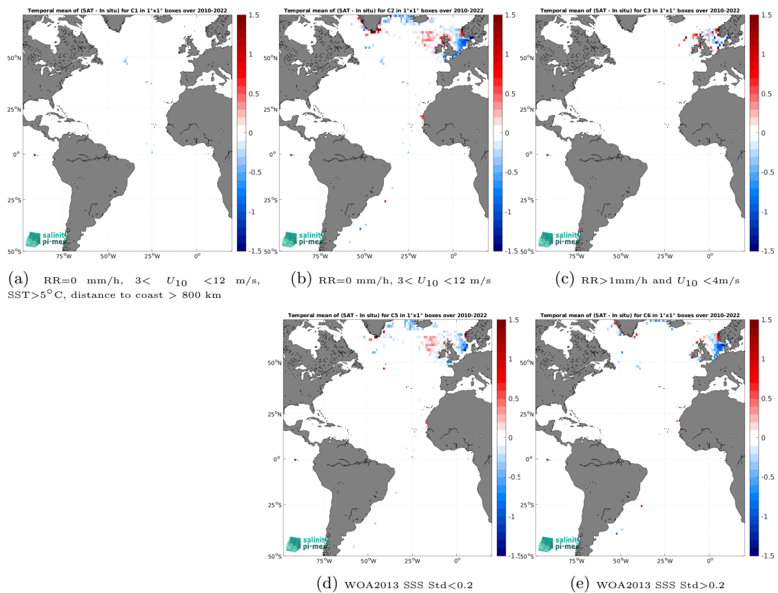
Figure 14: Temporal mean gridded over spatial boxes of size 1^\circ \times 1^\circ of \Delta SSS (SMOS SSS L4 v1 - Monthly (CMEMS-CNR) - ICES) for 5 different subdatasets corresponding to:RR=0 mm/h, 3 < U_{10} < 12 m/s, SST>5°C, distance to coast > 800 km (a), RR=0 mm/h, 3 < U_{10} < 12 m/s (b), RR>1mm/h and U_{10} < 4 m/s (c), WOA2013 SSS Std<0.2 (d), WOA2013 SSS Std>0.2 (e).
