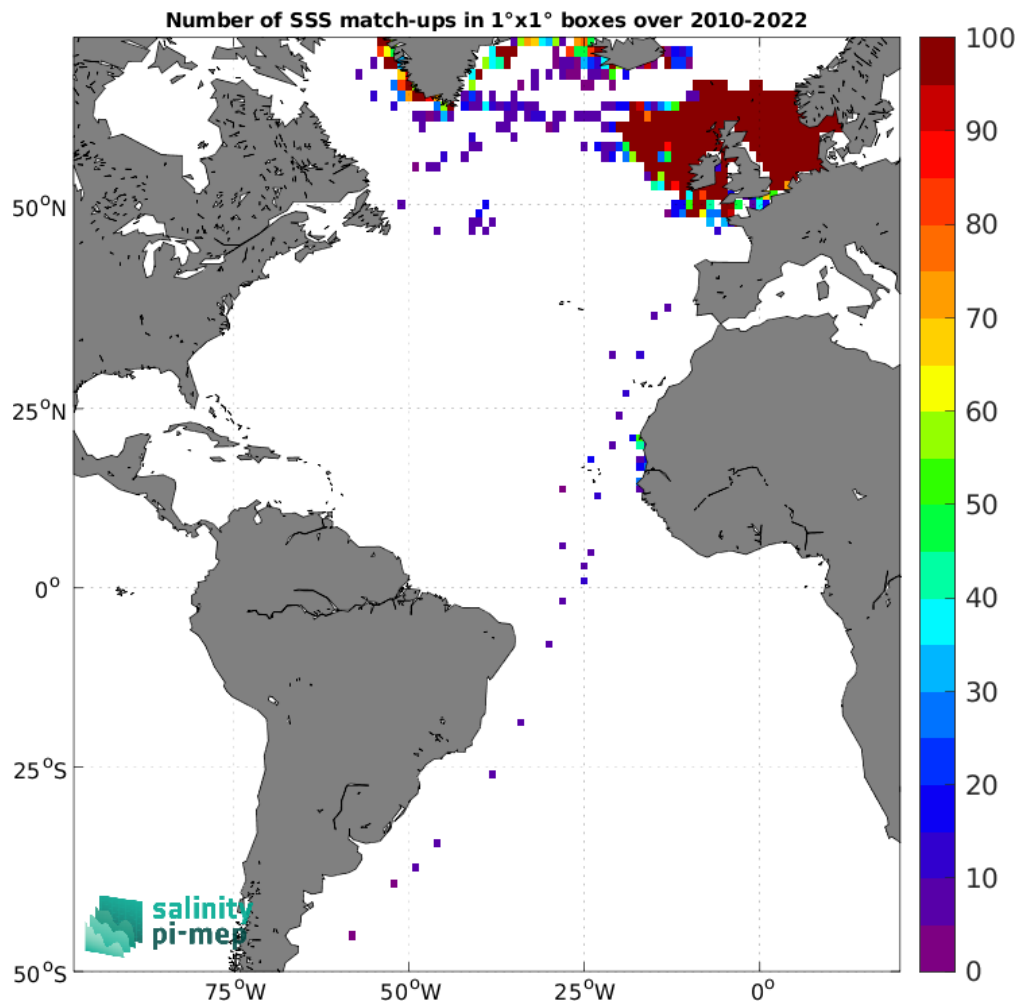
Figure 5: Number of SSS match-ups between ICES SSS and the SMOS SSS L4 v1 - Monthly (CMEMS-CNR) SSS product for the Atlantic Ocean Pi-MEP region over 1^\circ \times 1^\circ boxes and for the full satellite product period.
