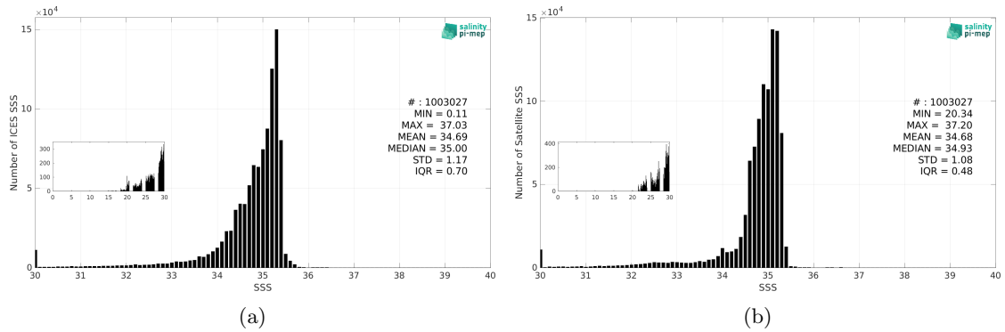
Figure 3: Histograms of SSS from ICES (a) and SMOS SSS L4 v1 - Monthly (CMEMS-CNR) (b) considering all match-up pairs per bins of 0.1 over the Atlantic Ocean Pi-MEP region and for the full satellite product period.
