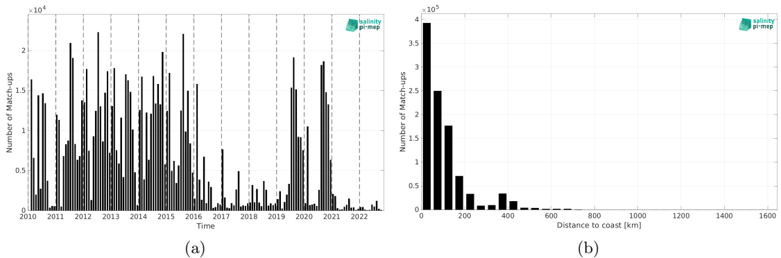
Figure 2: Number of match-ups between ICES and SMOS SSS L4 v1 - Monthly (CMEMS-CNR) SSS as a function of time (a) and as function of the distance to coast (b) over the Atlantic Ocean Pi-MEP region and for the full satellite product period.
