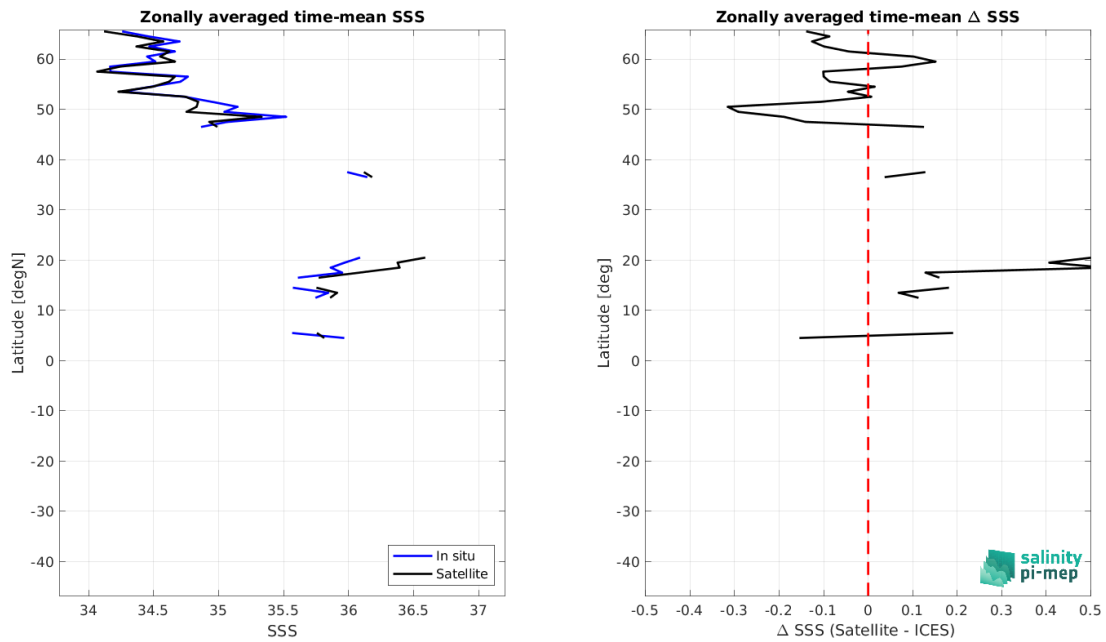
Figure 9: Left panel: Zonal mean SSS from SMOS SSS L4 v1 - Monthly (CMEMS-CNR) satellite product (black) and from ICES (blue). Right panel: Zonal mean of \Delta SSS (Satellite - ICES) for all the collected Pi-MEP match-up pairs estimated over the full satellite product period.
