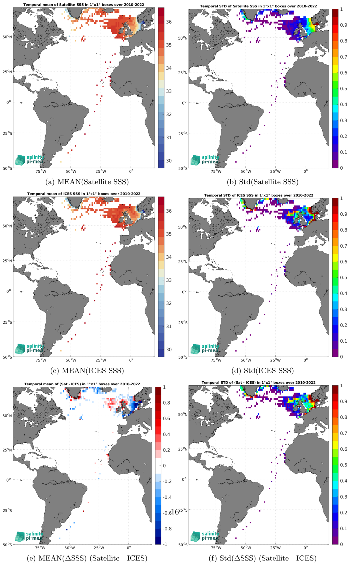
Figure 7: Temporal mean (left) and Std (right) of SSS from SMOS SSS L4 v1 - Monthly (CMEMS-CNR) (top), ICES (middle), and of \Delta SSS (Satellite - ICES). Only match-up pairs are used to generate these maps.
