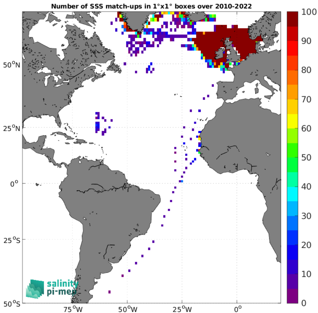
Figure 4: Number of SSS match-ups between ICES SSS and the SMOS SSS L4 v1 - Monthly (CMEMS-CNR) SSS product for the Atlantic Ocean Pi-MEP region over 1^\circ \times 1^\circ boxes and for the full satellite product period.
