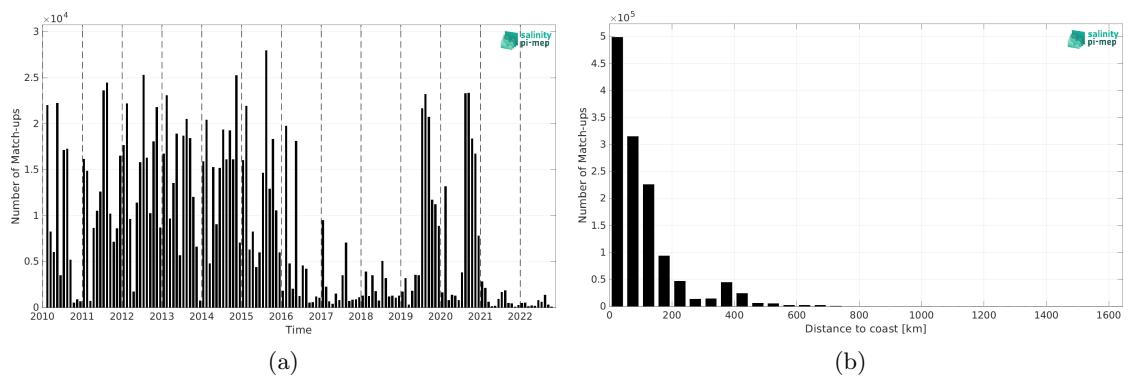
Figure 1: Number of match-ups between ICES and SMOS SSS L4 v1 - Monthly (CMEMS-CNR) SSS as a function of time (a) and as function of the distance to coast (b) over the Atlantic Ocean Pi-MEP region and for the full satellite product period.
