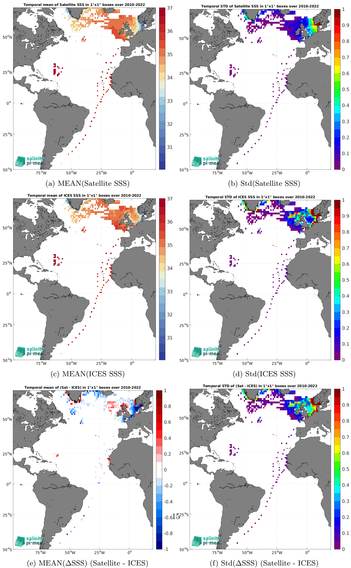
Figure 6: Temporal mean (left) and Std (right) of SSS from SMOS SSS L4 v1 - Monthly (CMEMS-CNR) (top), ICES (middle), and of \Delta SSS (Satellite - ICES). Only match-up pairs are used to generate these maps.
