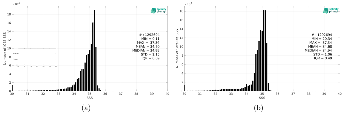
Figure 2: Histograms of SSS from ICES (a) and SMOS SSS L4 v1 - Monthly (CMEMS-CNR) (b) considering all match-up pairs per bins of 0.1 over the Atlantic Ocean Pi-MEP region and for the full satellite product period.
