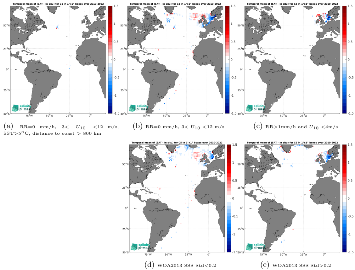
Figure 12: Temporal mean gridded over spatial boxes of size 1^\circ \times 1^\circ of \Delta SSS (SMOS SSS L4 v1 - Monthly (CMEMS-CNR) - ICES) for 5 different subdatasets corresponding to:RR=0 mm/h, 3 < U_{10} < 12 m/s, SST >5^\circ\text{C} , distance to coast > 800 km (a), RR=0 mm/h, 3 < U_{10} < 12 m/s (b), RR >1 mm/h and U_{10} < 4 m/s (c), WOA2013 SSS Std <0.2 (d), WOA2013 SSS Std >0.2 (e).
