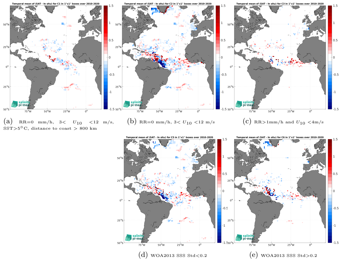
Figure 13: Temporal mean gridded over spatial boxes of size 1^\circ \times 1^\circ of \Delta SSS (SMOS SSS L4 v1 - Monthly (CMEMS-CNR) - Surface drifters) for 5 different subdatasets corresponding to:RR=0 mm/h, 3 < U_{10} < 12 m/s, SST >5^\circ\text{C} , distance to coast > 800 km (a), RR=0 mm/h, 3 < U_{10} < 12 m/s (b), RR >1 mm/h and U_{10} < 4 m/s (c), WOA2013 SSS Std <0.2 (d), WOA2013 SSS Std >0.2 (e).
