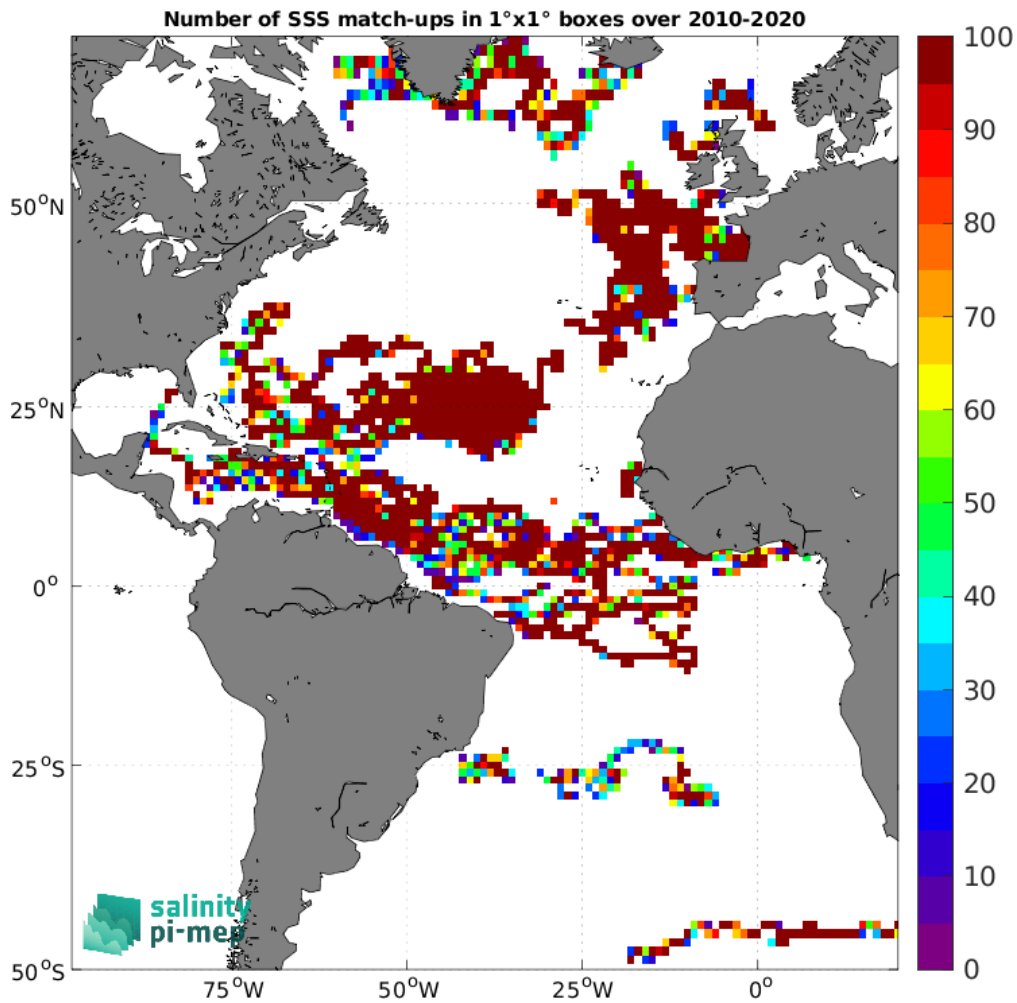
Figure 4: Number of SSS match-ups between Surface drifters SSS and the SMOS SSS L4 v1 - Monthly (CMEMS-CNR) SSS product for the Atlantic Ocean Pi-MEP region over 1°×1° boxes and for the full satellite product period.
