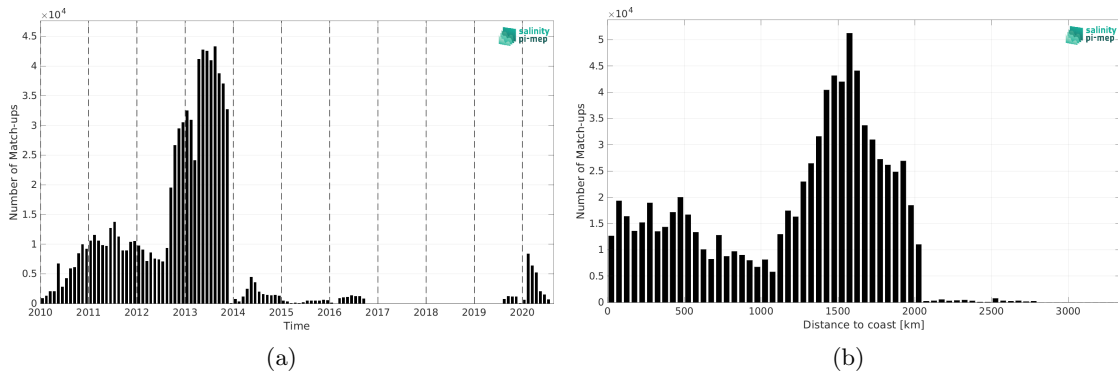
Figure 2: Number of match-ups between Surface drifters and SMOS SSS L4 v1 - Monthly (CMEMS-CNR) SSS as a function of time (a) and as function of the distance to coast (b) over the Atlantic Ocean Pi-MEP region and for the full satellite product period.
