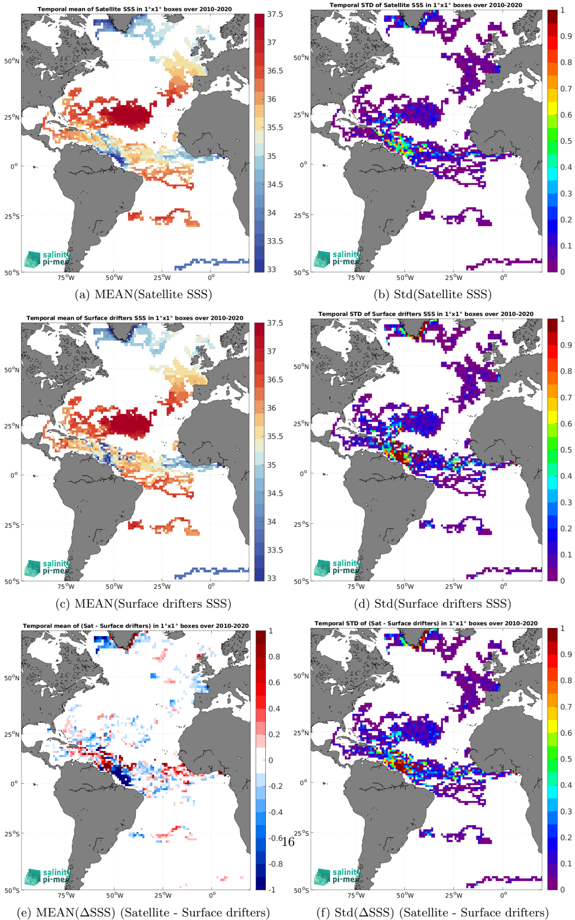
Figure 6: Temporal mean (left) and Std (right) of SSS from SMOS SSS L4 v1 - Monthly (CMEMS-CNR) (top), Surface drifters (middle), and of \Delta SSS (Satellite - Surface drifters). Only match-up pairs are used to generate these maps.
