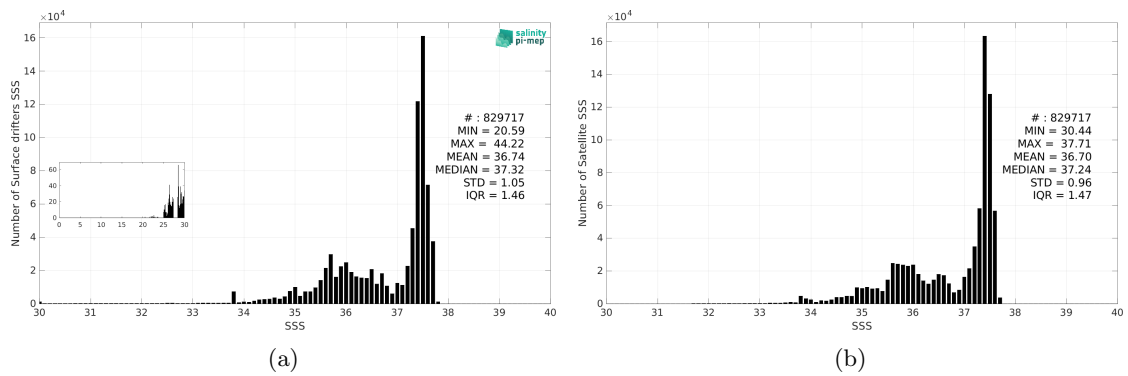
Figure 3: Histograms of SSS from Surface drifters (a) and SMOS SSS L4 v1 - Monthly (CMEMS-CNR) (b) considering all match-up pairs per bins of 0.1 over the Atlantic Ocean Pi-MEP region and for the full satellite product period.
