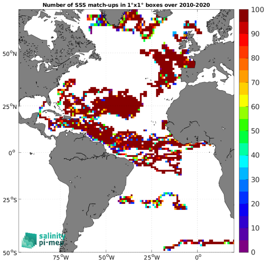
Figure 3: Number of SSS match-ups between Surface drifters SSS and the SMOS SSS L4 v1 - Monthly (CMEMS-CNR) SSS product for the Atlantic Ocean Pi-MEP region over 1°×1° boxes and for the full satellite product period.
