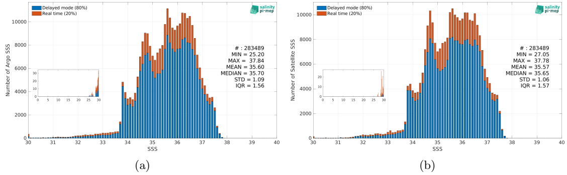
Figure 3: Histograms of SSS from Argo (a) and SMOS SSS L4 v1 - Monthly (CMEMS-CNR) (b) considering all match-up pairs per bins of 0.1 over the Atlantic Ocean Pi-MEP region and for the full satellite product period.
