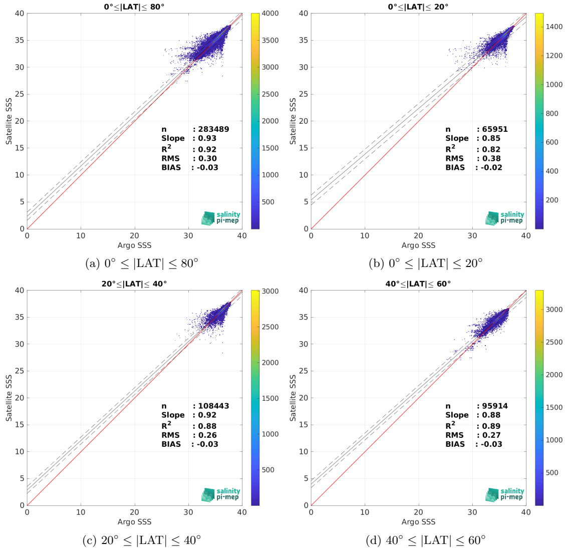
Figure 10: Contour maps of the concentration of SMOS SSS L4 v1 - Monthly (CMEMS-CNR) SSS (y-axis) versus Argo SSS (x-axis) at match-up pairs for different latitude bands. For each plot, the red line shows x=y . The black thin and dashed lines indicate a linear fit through the data cloud and the \pm 95\% confidence levels, respectively. The number match-up pairs n , the slope and R^2 coefficient of the linear fit, the root mean square (RMS) and the mean bias between satellite and in situ data are indicated for each latitude band in each plots.
