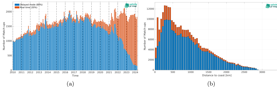
Figure 2: Number of match-ups between Argo and SMOS SSS L4 v1 - Monthly (CMEMS-CNR) SSS as a function of time (a) and as function of the distance to coast (b) over the Atlantic Ocean Pi-MEP region and for the full satellite product period.
