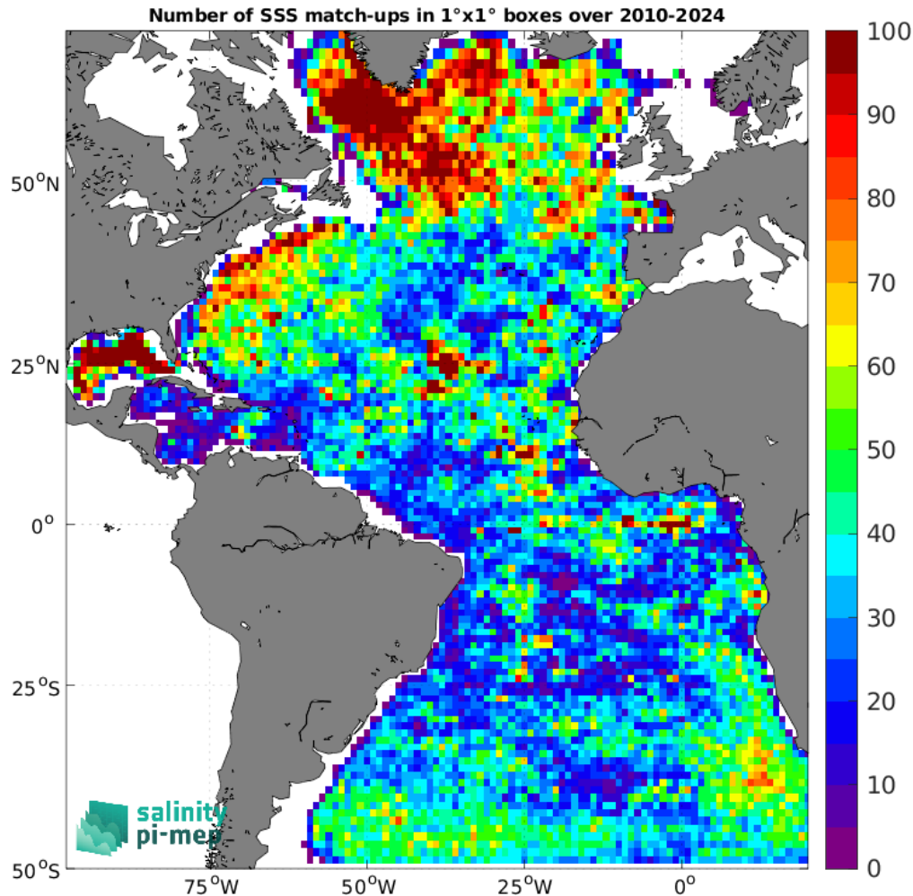
Figure 5: Number of SSS match-ups between Argo SSS and the SMOS SSS L4 v1 - Monthly (CMEMS-CNR) SSS product for the Atlantic Ocean Pi-MEP region over 1^\circ \times 1^\circ boxes and for the full satellite product period.
