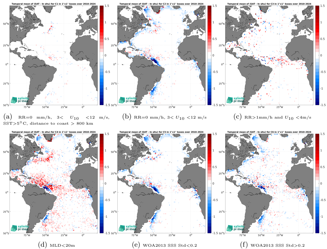
Figure 14: Temporal mean gridded over spatial boxes of size 1^\circ \times 1^\circ of \Delta SSS (SMOS SSS L4 v1 - Monthly (CMEMS-CNR) - Argo) for 6 different subdatasets corresponding to:RR=0 mm/h, 3 < U_{10} < 12 m/s, SST>5°C, distance to coast > 800 km (a), RR=0 mm/h, 3 < U_{10} < 12 m/s (b), RR>1mm/h and U_{10} < 4 m/s (c),MLD<20m (d),WOA2013 SSS Std<0.2 (e),WOA2013 SSS Std>0.2 (f).
