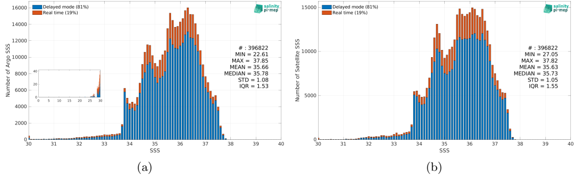
Figure 2: Histograms of SSS from Argo (a) and SMOS SSS L4 v1 - Monthly (CMEMS-CNR) (b) considering all match-up pairs per bins of 0.1 over the Atlantic Ocean Pi-MEP region and for the full satellite product period.
