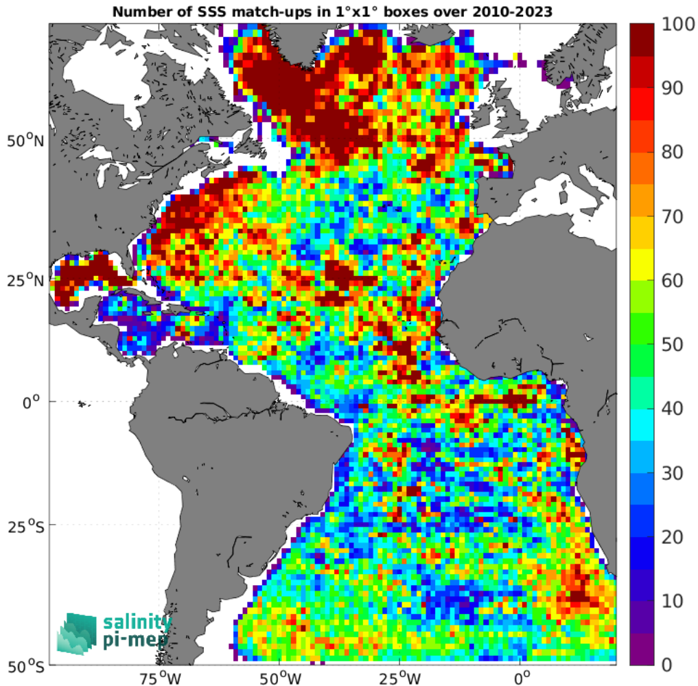
Figure 4: Number of SSS match-ups between Argo SSS and the SMOS SSS L4 v1 - Monthly (CMEMS-CNR) SSS product for the Atlantic Ocean Pi-MEP region over 1^\circ \times 1^\circ boxes and for the full satellite product period.
