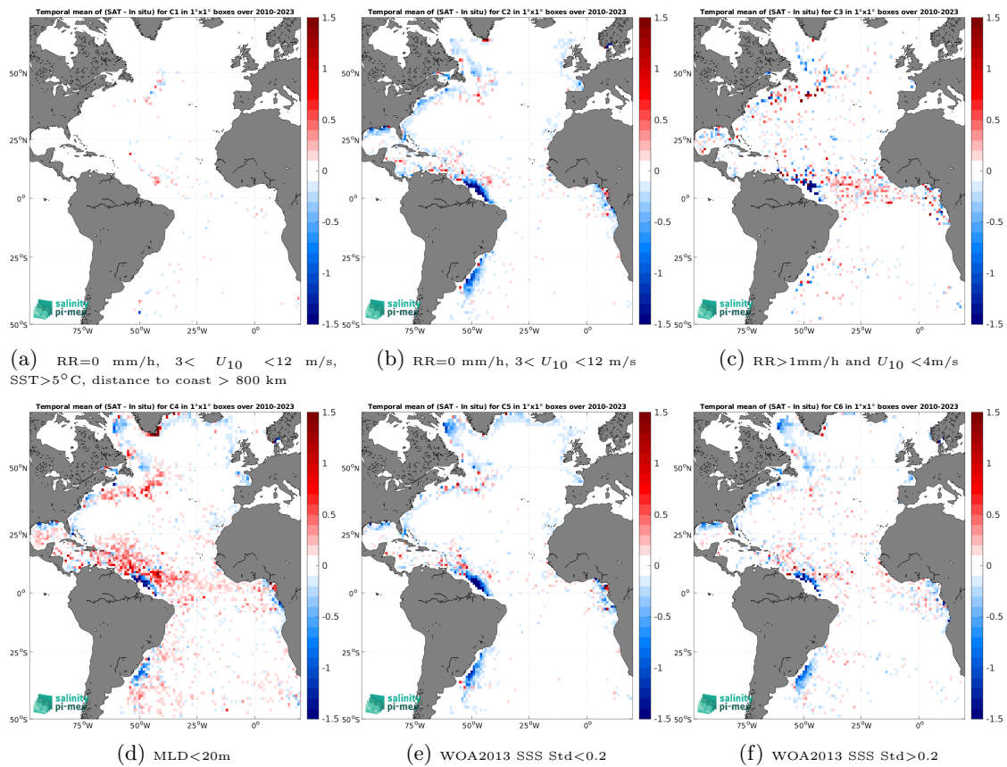
Figure 12: Temporal mean gridded over spatial boxes of size 1^\circ \times 1^\circ of \Delta SSS (SMOS SSS L4 v1 - Monthly (CMEMS-CNR) - Argo) for 6 different subdatasets corresponding to:RR=0 mm/h, 3 < U_{10} < 12 m/s, SST >5^\circ C, distance to coast > 800 km (a), RR=0 mm/h, 3 < U_{10} < 12 m/s (b), RR >1 mm/h and U_{10} < 4 m/s (c),MLD <20 m (d),WOA2013 SSS Std <0.2 (e),WOA2013 SSS Std >0.2 (f).
