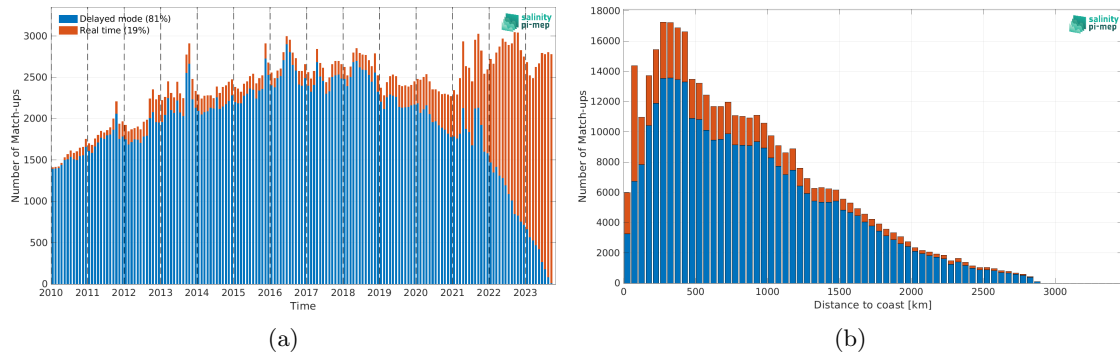
Figure 1: Number of match-ups between Argo and SMOS SSS L4 v1 - Monthly (CMEMS-CNR) SSS as a function of time (a) and as function of the distance to coast (b) over the Atlantic Ocean Pi-MEP region and for the full satellite product period.
