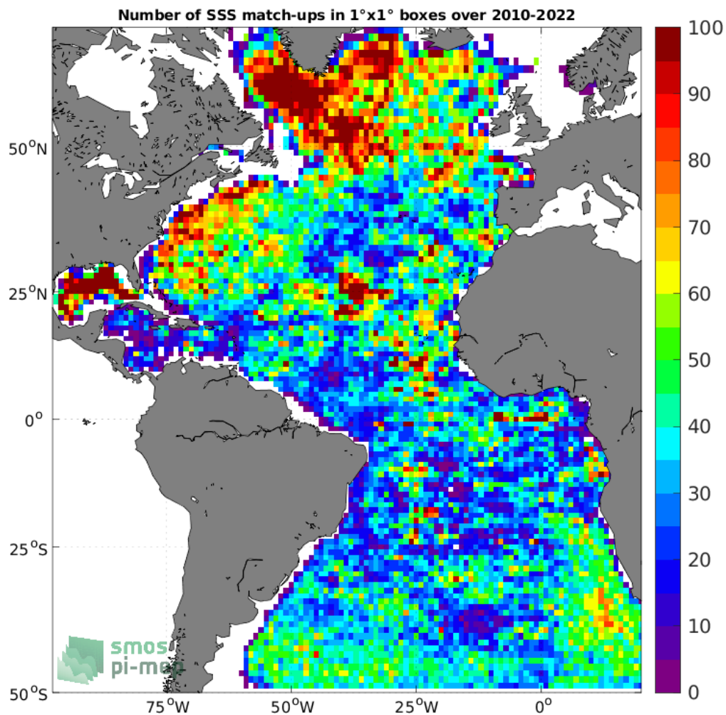
Figure 4: Number of SSS match-ups between Argo SSS and the SMOS SSS L4 v1 - Monthly (CMEMS-CNR) SSS product for the Atlantic Ocean Pi-MEP region over 1°×1° boxes and for the full satellite product period.
