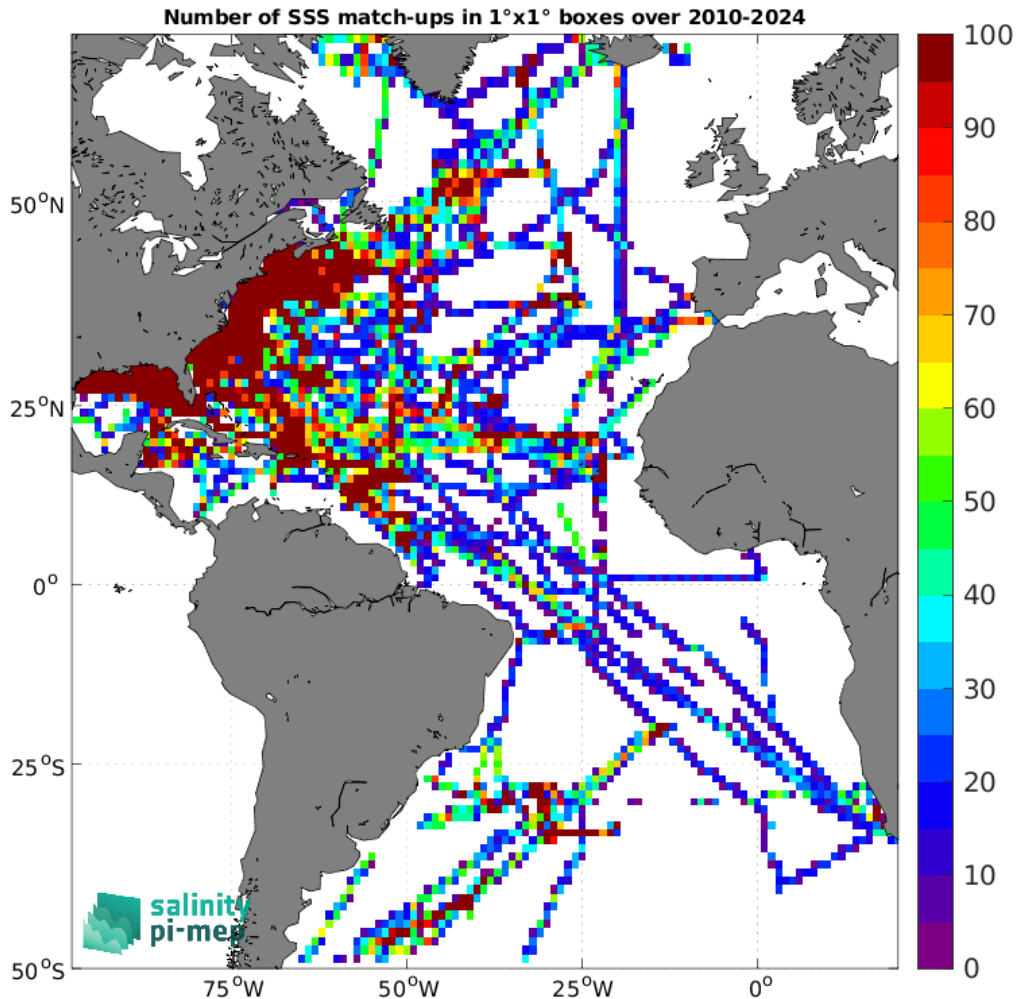
Figure 5: Number of SSS match-ups between TSG (SAMOS) SSS and the SMOS SSS L4 v1 - Daily (CMEMS-CNR) SSS product for the Atlantic Ocean Pi-MEP region over 1^\circ \times 1^\circ boxes and for the full satellite product period.
