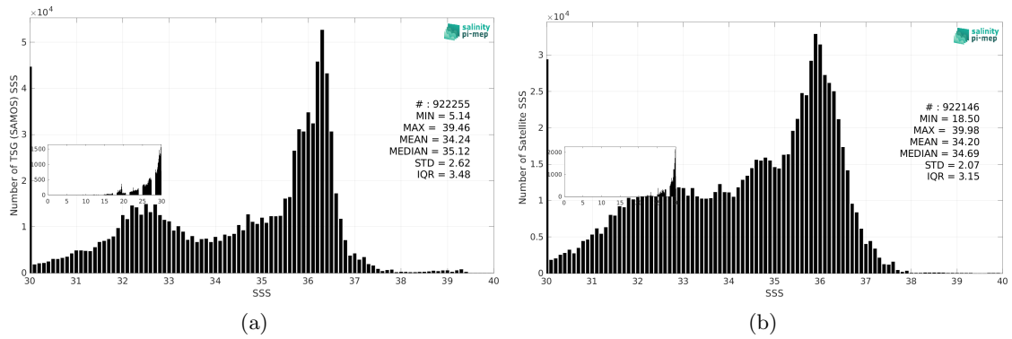
Figure 3: Histograms of SSS from TSG (SAMOS) (a) and SMOS SSS L4 v1 - Daily (CMEMS-CNR) (b) considering all match-up pairs per bins of 0.1 over the Atlantic Ocean Pi-MEP region and for the full satellite product period.
