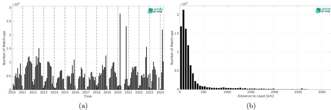
Figure 2: Number of match-ups between TSG (SAMOS) and SMOS SSS L4 v1 - Daily (CMEMS-CNR) SSS as a function of time (a) and as function of the distance to coast (b) over the Atlantic Ocean Pi-MEP region and for the full satellite product period.
