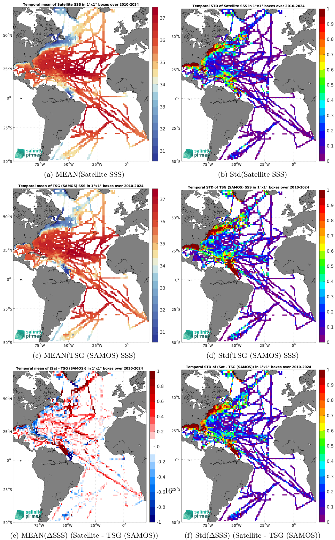
Figure 7: Temporal mean (left) and Std (right) of SSS from SMOS SSS L4 v1 - Daily (CMEMS-CNR) (top), TSG (SAMOS) (middle), and of \Delta SSS (Satellite - TSG (SAMOS)). Only match-up pairs are used to generate these maps.
