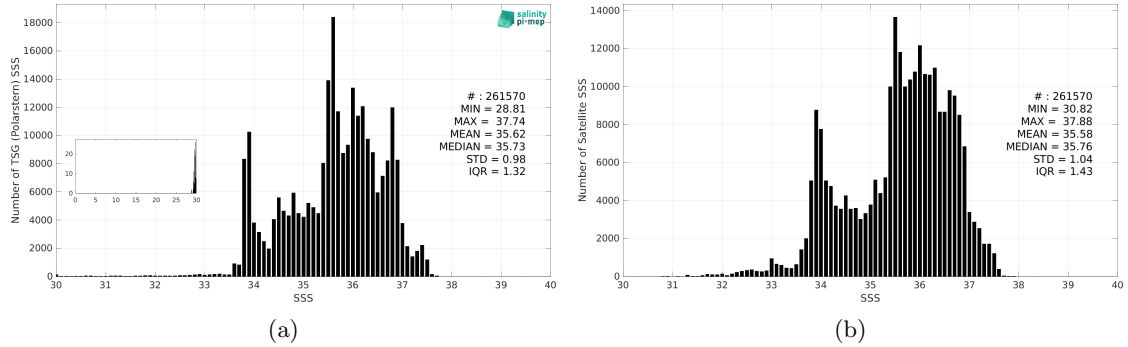
Figure 3: Histograms of SSS from TSG (Polarstern) (a) and SMOS SSS L4 v1 - Daily (CMEMS-CNR) (b) considering all match-up pairs per bins of 0.1 over the Atlantic Ocean Pi-MEP region and for the full satellite product period.
