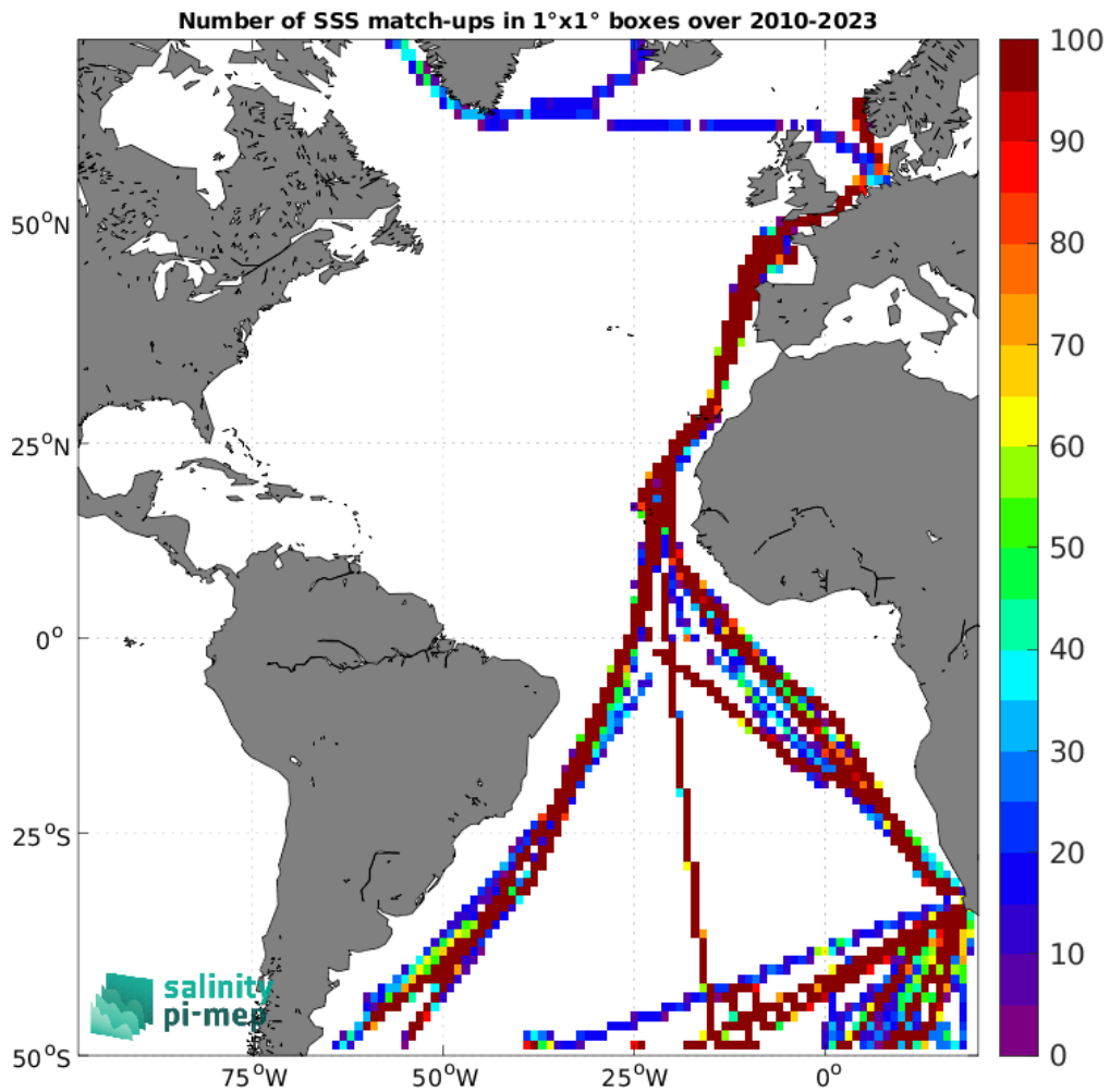
Figure 5: Number of SSS match-ups between TSG (Polarstern) SSS and the SMOS SSS L4 v1 - Daily (CMEMS-CNR) SSS product for the Atlantic Ocean Pi-MEP region over 1^\circ \times 1^\circ boxes and for the full satellite product period.
