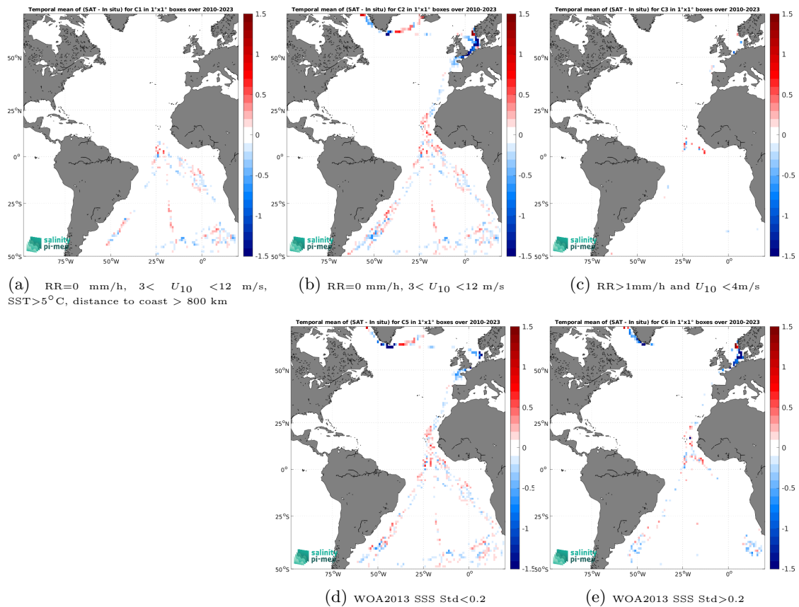
Figure 14: Temporal mean gridded over spatial boxes of size 1^\circ \times 1^\circ of \Delta SSS (SMOS SSS L4 v1 - Daily (CMEMS-CNR) - TSG (Polarstern)) for 5 different subdatasets corresponding to:RR=0 mm/h, 3 < U_{10} < 12 m/s, SST >5^\circ\text{C} , distance to coast > 800 km (a), RR=0 mm/h, 3 < U_{10} < 12 m/s (b), RR >1 mm/h and U_{10} < 4 m/s (c), WOA2013 SSS Std <0.2 (d), WOA2013 SSS Std >0.2 (e).
