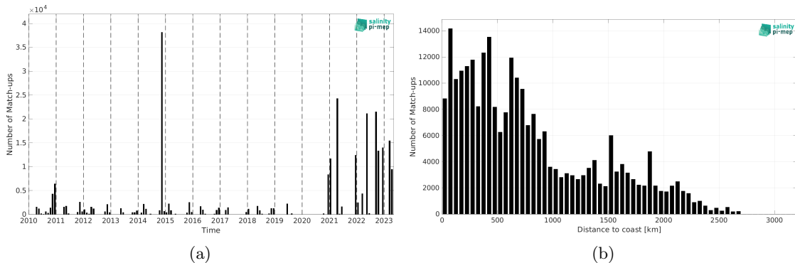
Figure 2: Number of match-ups between TSG (Polarstern) and SMOS SSS L4 v1 - Daily (CMEMS-CNR) SSS as a function of time (a) and as function of the distance to coast (b) over the Atlantic Ocean Pi-MEP region and for the full satellite product period.
