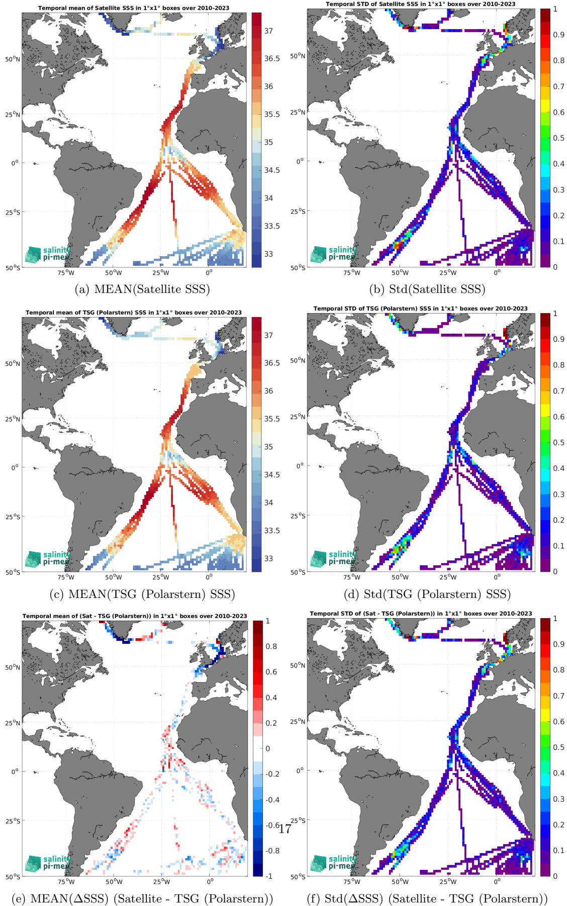
Figure 7: Temporal mean (left) and Std (right) of SSS from SMOS SSS L4 v1 - Daily (CMEMS-CNR) (top), TSG (Polarstern) (middle), and of \Delta SSS (Satellite - TSG (Polarstern)). Only match-up pairs are used to generate these maps.
