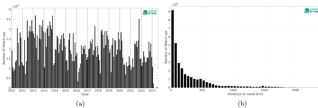
Figure 2: Number of match-ups between TSG (LEGOS-DM) and SMOS SSS L4 v1 - Daily (CMEMS-CNR) SSS as a function of time (a) and as function of the distance to coast (b) over the Atlantic Ocean Pi-MEP region and for the full satellite product period.
