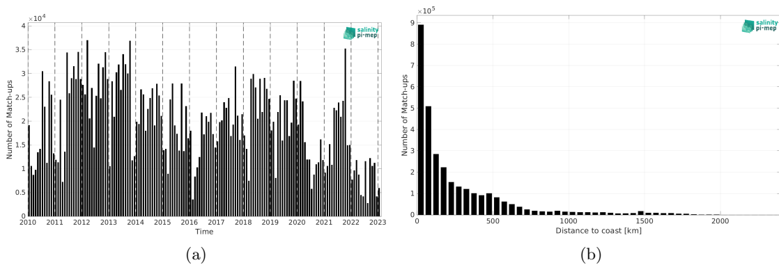
Figure 2: Number of match-ups between TSG (LEGOS-DM) and SMOS SSS L4 v1 - Daily (CMEMS-CNR) SSS as a function of time (a) and as function of the distance to coast (b) over the Atlantic Ocean Pi-MEP region and for the full satellite product period.
