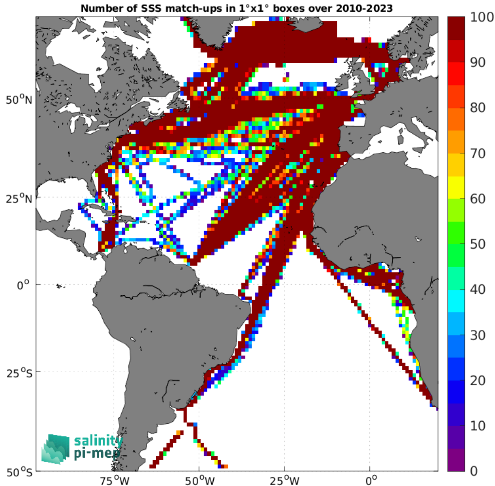
Figure 5: Number of SSS match-ups between TSG (LEGOS-DM) SSS and the SMOS SSS L4 v1 - Daily (CMEMS-CNR) SSS product for the Atlantic Ocean Pi-MEP region over 1^\circ \times 1^\circ boxes and for the full satellite product period.
