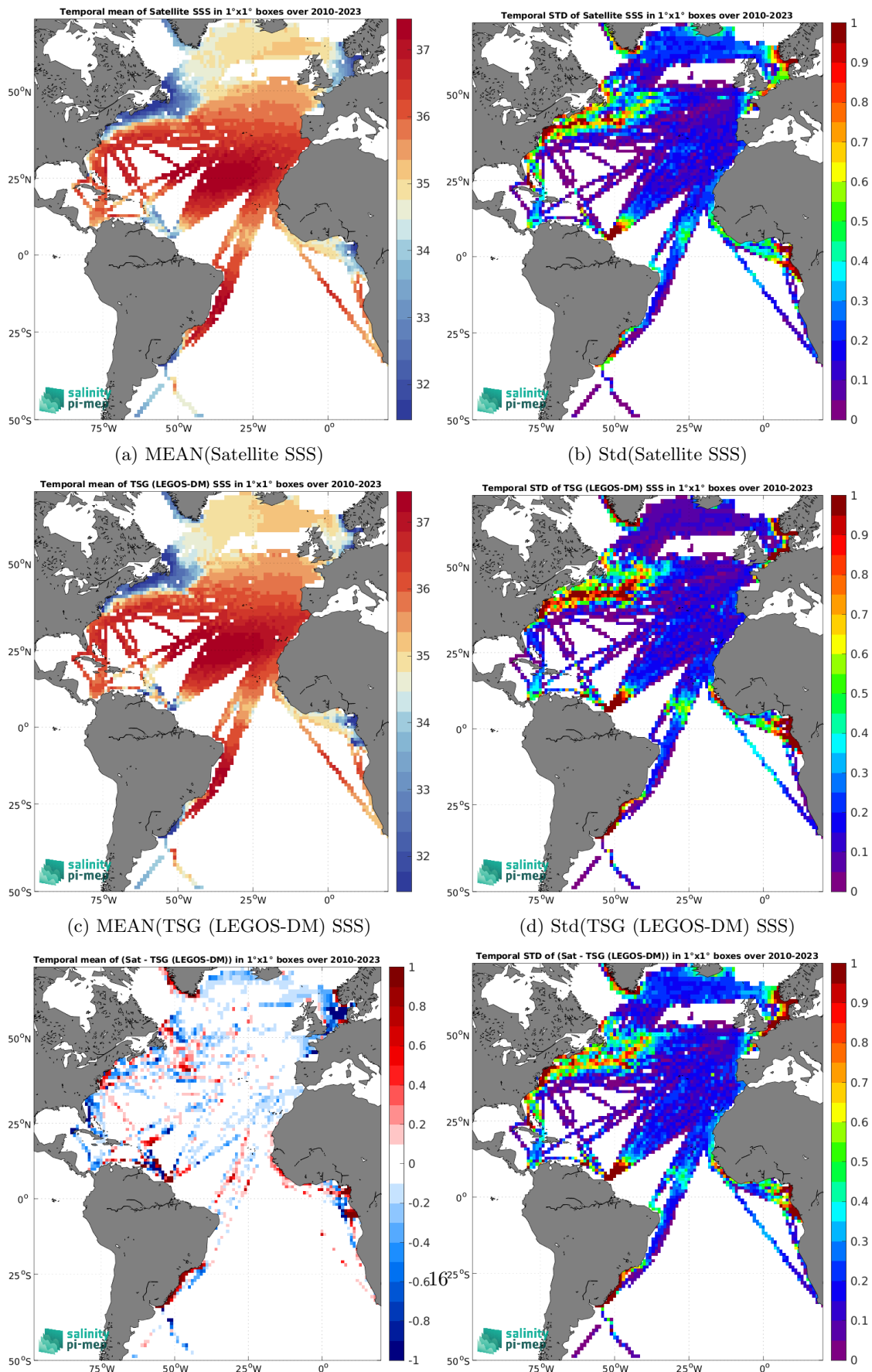
(e) MEAN( \Delta SSS) (Satellite - TSG (LEGOS-DM)) (f) Std( \Delta SSS) (Satellite - TSG (LEGOS-DM)) Figure 7: Temporal mean (left) and Std (right) of SSS from SMOS SSS L4 v1 - Daily (CMEMS-CNR) (top), TSG (LEGOS-DM) (middle), and of \Delta SSS (Satellite - TSG (LEGOS-DM)). Only match-up pairs are used to generate these maps.
