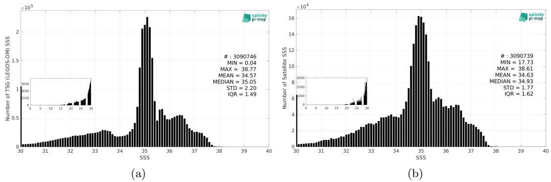
Figure 3: Histograms of SSS from TSG (LEGOS-DM) (a) and SMOS SSS L4 v1 - Daily (CMEMS-CNR) (b) considering all match-up pairs per bins of 0.1 over the Atlantic Ocean Pi-MEP region and for the full satellite product period.
