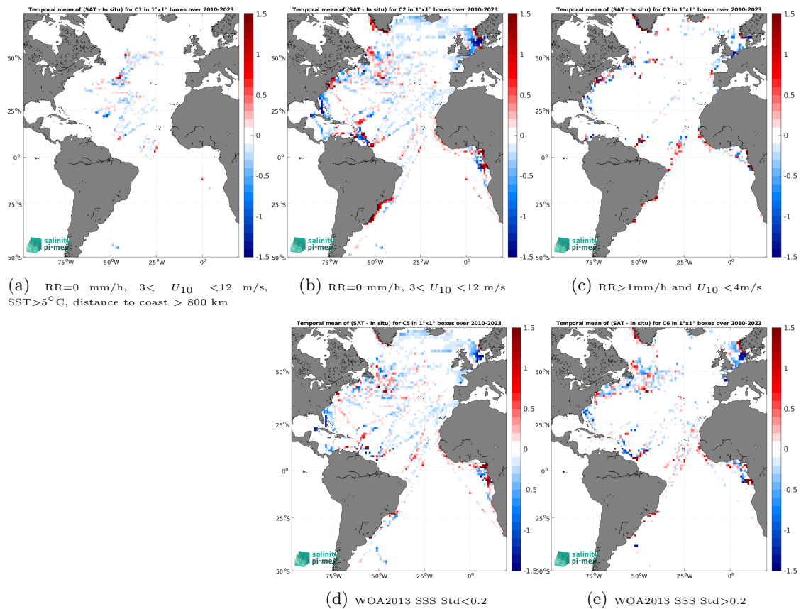
Figure 14: Temporal mean gridded over spatial boxes of size 1^\circ \times 1^\circ of \Delta SSS (SMOS SSS L4 v1 - Daily (CMEMS-CNR) - TSG (LEGOS-DM)) for 5 different subdatasets corresponding to:RR=0 mm/h, 3 < U_{10} < 12 m/s, SST >5^\circ\text{C} , distance to coast > 800 km (a), RR=0 mm/h, 3 < U_{10} < 12 m/s (b), RR >1 mm/h and U_{10} < 4 m/s (c), WOA2013 SSS Std <0.2 (d), WOA2013 SSS Std >0.2 (e).
