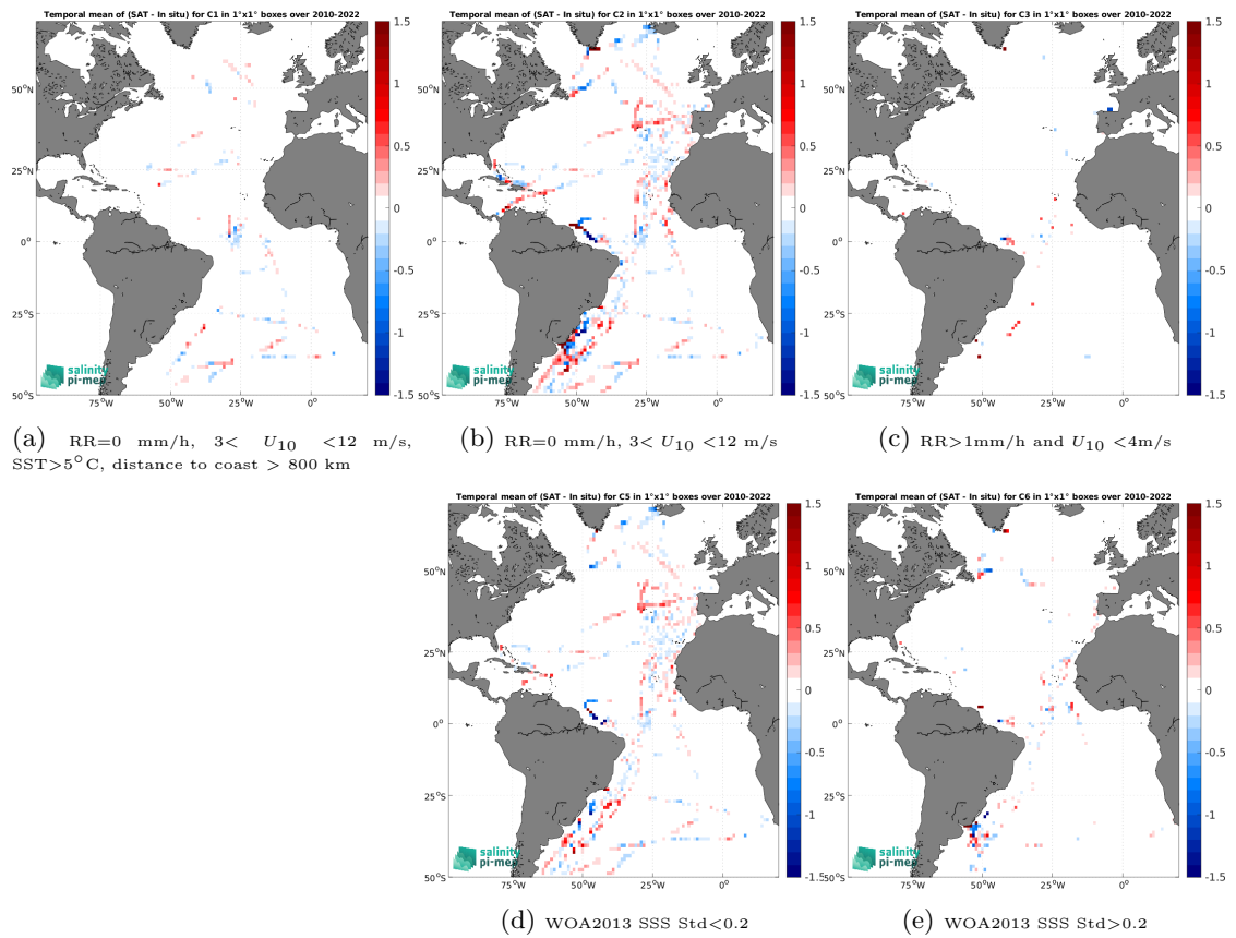
Figure 14: Temporal mean gridded over spatial boxes of size 1^\circ \times 1^\circ of \Delta SSS (SMOS SSS L4 v1 - Daily (CMEMS-CNR) - TSG (CSIC-UTM)) for 5 different subdatasets corresponding to:RR=0 mm/h, 3 < U_{10} < 12 m/s, SST >5^\circ\text{C} , distance to coast > 800 km (a), RR=0 mm/h, 3 < U_{10} < 12 m/s (b), RR >1 mm/h and U_{10} < 4 m/s (c), WOA2013 SSS Std <0.2 (d), WOA2013 SSS Std >0.2 (e).
