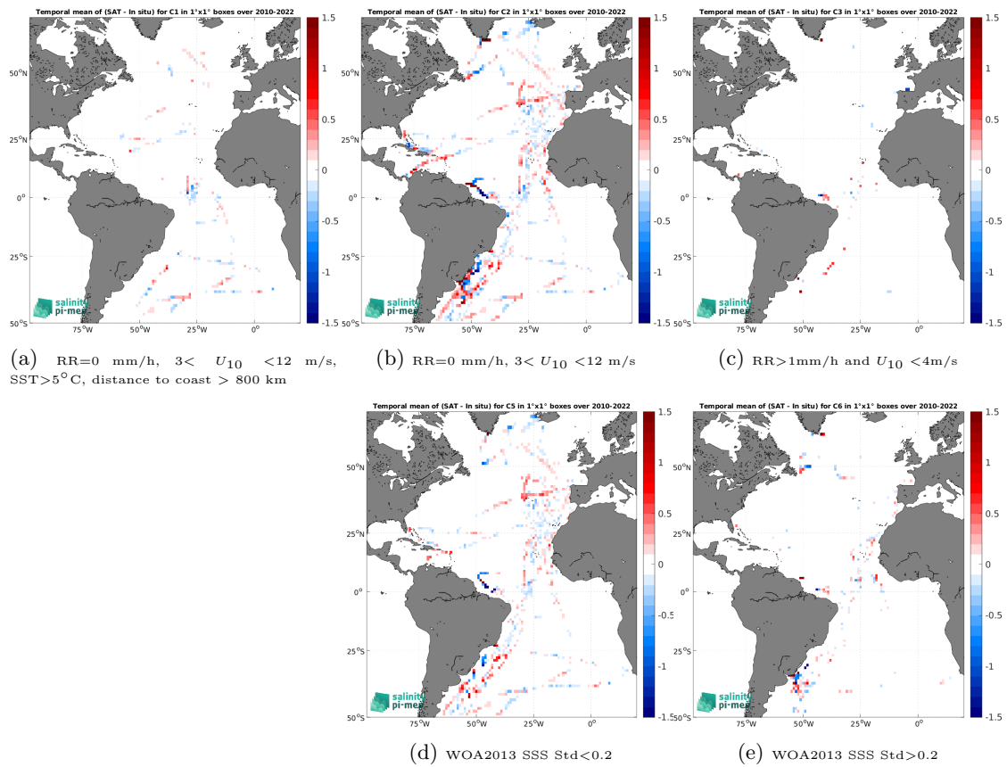
Figure 14: Temporal mean gridded over spatial boxes of size 1^\circ \times 1^\circ of \Delta SSS (SMOS SSS L4 v1 - Daily (CMEMS-CNR) - TSG (CSIC-UTM)) for 5 different subdatasets corresponding to:RR=0 mm/h, 3 < U_{10} < 12 m/s, SST >5^\circ\text{C} , distance to coast > 800 km (a), RR=0 mm/h, 3 < U_{10} < 12 m/s (b), RR >1 mm/h and U_{10} < 4 m/s (c), WOA2013 SSS Std <0.2 (d), WOA2013 SSS Std >0.2 (e).
