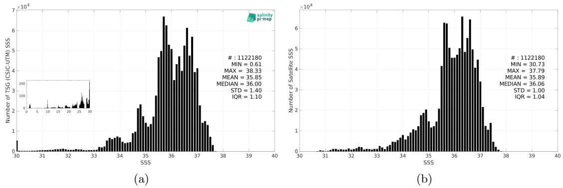
Figure 3: Histograms of SSS from TSG (CSIC-UTM) (a) and SMOS SSS L4 v1 - Daily (CMEMS-CNR) (b) considering all match-up pairs per bins of 0.1 over the Atlantic Ocean Pi-MEP region and for the full satellite product period.
