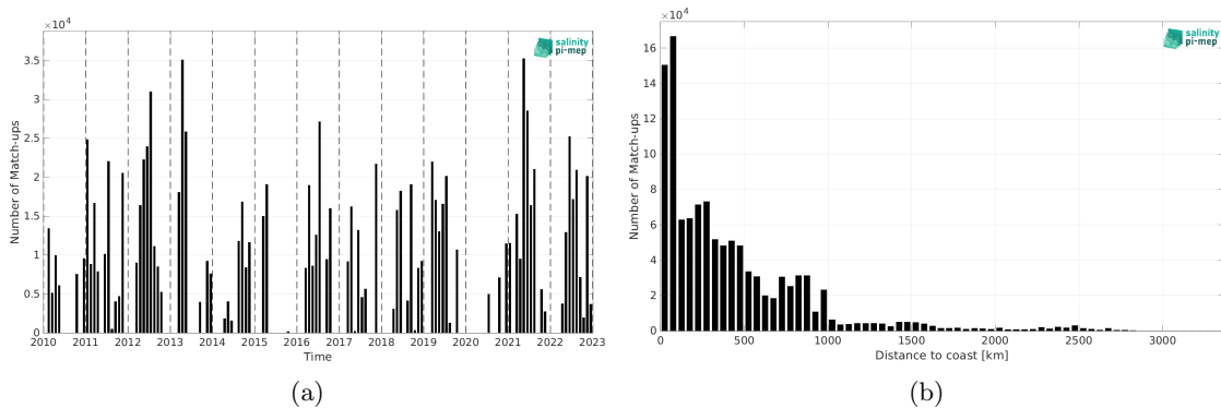
Figure 2: Number of match-ups between TSG (CSIC-UTM) and SMOS SSS L4 v1 - Daily (CMEMS-CNR) SSS as a function of time (a) and as function of the distance to coast (b) over the Atlantic Ocean Pi-MEP region and for the full satellite product period.
