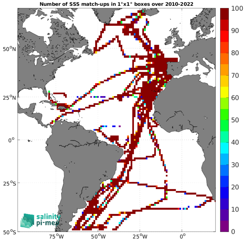
Figure 5: Number of SSS match-ups between TSG (CSIC-UTM) SSS and the SMOS SSS L4 v1 - Daily (CMEMS-CNR) SSS product for the Atlantic Ocean Pi-MEP region over 1^\circ \times 1^\circ boxes and for the full satellite product period.
