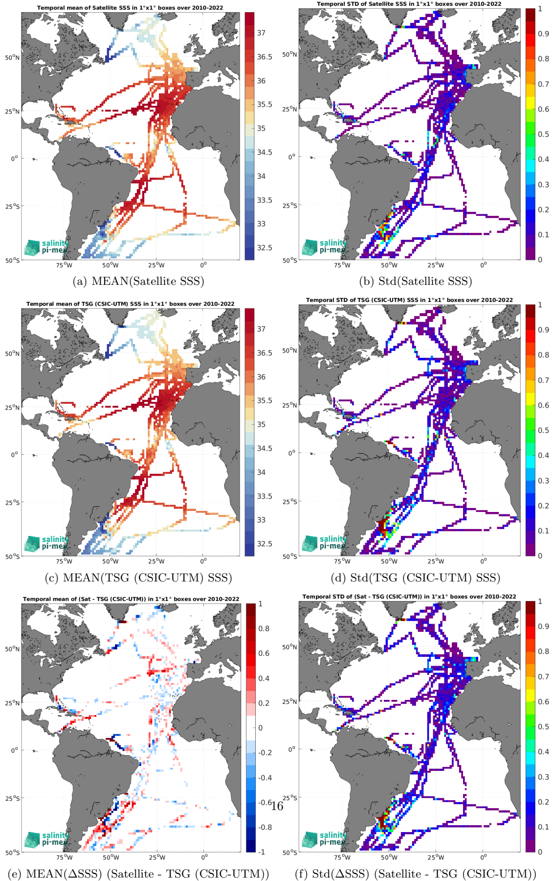
Figure 7: Temporal mean (left) and Std (right) of SSS from SMOS SSS L4 v1 - Daily (CMEMS-CNR) (top), TSG (CSIC-UTM) (middle), and of \Delta SSS (Satellite - TSG (CSIC-UTM)). Only match-up pairs are used to generate these maps.
