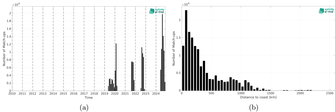
Figure 2: Number of match-ups between Saildrone and SMOS SSS L4 v1 - Daily (CMEMS-CNR) SSS as a function of time (a) and as function of the distance to coast (b) over the Atlantic Ocean Pi-MEP region and for the full satellite product period.
