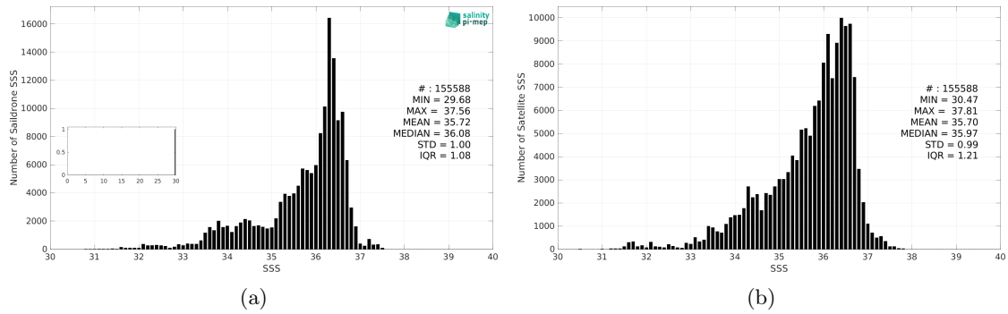
Figure 3: Histograms of SSS from Saildrone (a) and SMOS SSS L4 v1 - Daily (CMEMS-CNR) (b) considering all match-up pairs per bins of 0.1 over the Atlantic Ocean Pi-MEP region and for the full satellite product period.
