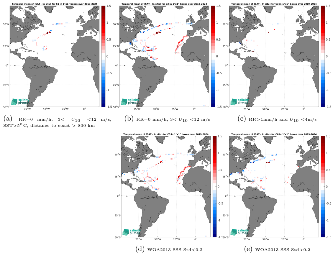
Figure 14: Temporal mean gridded over spatial boxes of size 1^\circ \times 1^\circ of \Delta\text{SSS} (SMOS SSS L4 v1 - Daily (CMEMS-CNR) - Sailydrone) for 5 different subdatasets corresponding to:RR=0 mm/h, 3 < U_{10} < 12 m/s, SST >5^\circ\text{C} , distance to coast > 800 km (a), RR=0 mm/h, 3 < U_{10} < 12 m/s (b), RR >1 mm/h and U_{10} < 4 m/s (c), WOA2013 SSS Std <0.2 (d), WOA2013 SSS Std >0.2 (e).
