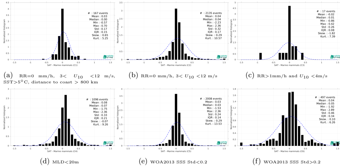
Figure 15: Normalized histogram of \Delta\text{SSS} (SMOS SSS L4 v1 - Daily (CMEMS-CNR) - Marine mammals) for 6 different subdatasets corresponding to: RR=0 mm/h, 3 < U_{10} < 12 m/s, SST>5°C, distance to coast > 800 km (a), RR=0 mm/h, 3 < U_{10} < 12 m/s (b), RR>1mm/h and U_{10} < 4 m/s (c), MLD<20m (d), WOA2013 SSS Std<0.2 (e), WOA2013 SSS Std>0.2 (f).
