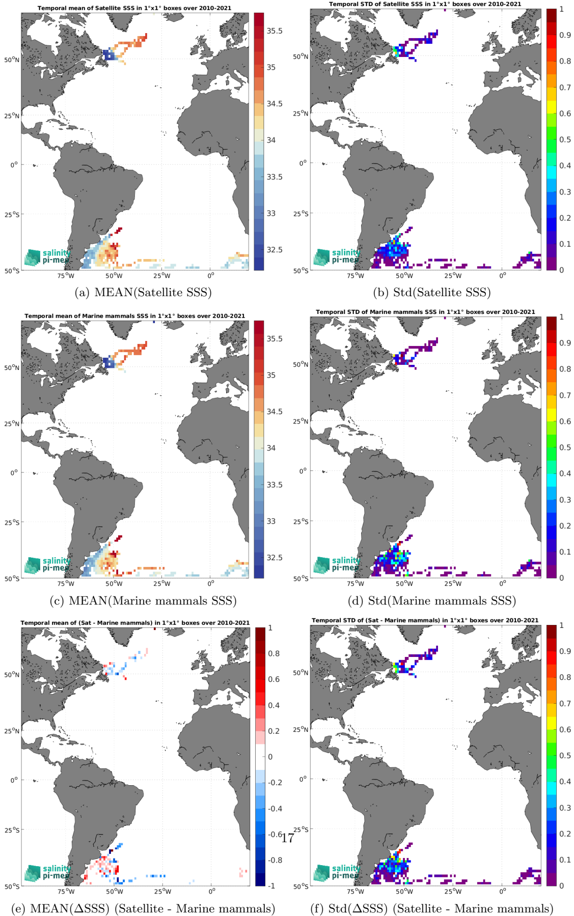
Figure 7: Temporal mean (left) and Std (right) of SSS from SMOS SSS L4 v1 - Daily (CMEMS-CNR) (top), Marine mammals (middle), and of \Delta SSS (Satellite - Marine mammals). Only match-up pairs are used to generate these maps.
