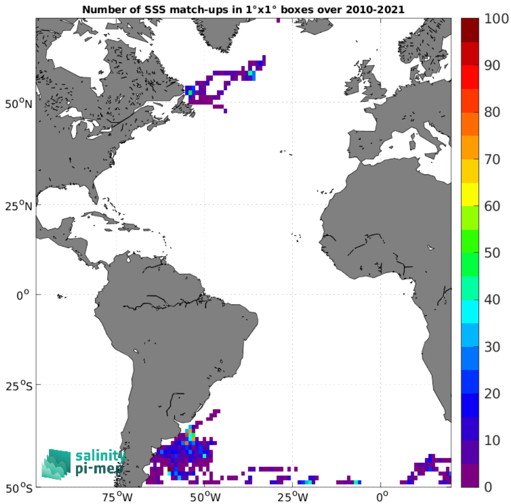
Figure 5: Number of SSS match-ups between Marine mammals SSS and the SMOS SSS L4 v1 - Daily (CMEMS-CNR) SSS product for the Atlantic Ocean Pi-MEP region over 1°x1° boxes and for the full satellite product period.
