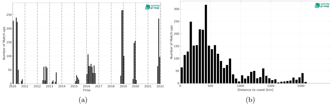
Figure 2: Number of match-ups between Marine mammals and SMOS SSS L4 v1 - Daily (CMEMS-CNR) SSS as a function of time (a) and as function of the distance to coast (b) over the Atlantic Ocean Pi-MEP region and for the full satellite product period.
