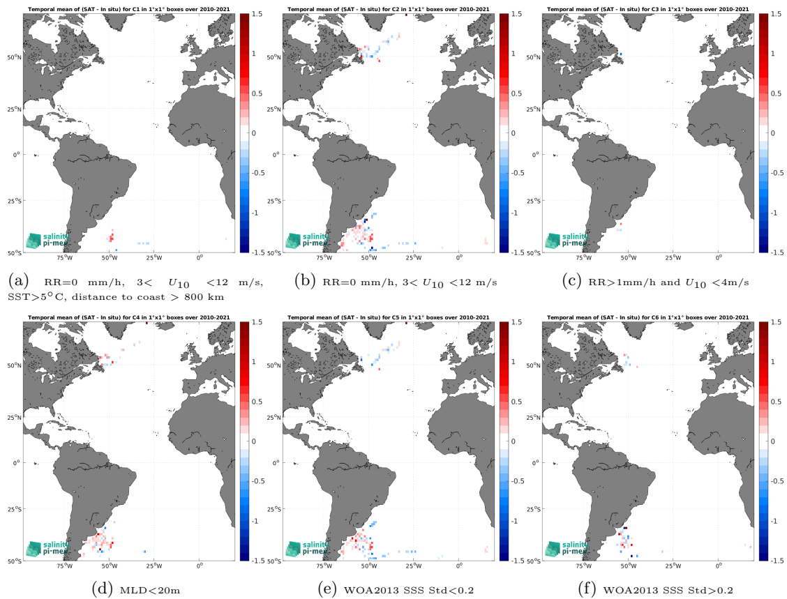
Figure 14: Temporal mean gridded over spatial boxes of size 1^\circ \times 1^\circ of \Delta SSS (SMOS SSS L4 v1 - Daily (CMEMS-CNR) - Marine mammals) for 6 different subdatasets corresponding to:RR=0 mm/h, 3 < U_{10} < 12 m/s, SST >5^\circ C, distance to coast > 800 km (a), RR=0 mm/h, 3 < U_{10} < 12 m/s (b), RR >1 mm/h and U_{10} < 4 m/s (c),MLD <20 m (d),WOA2013 SSS Std <0.2 (e),WOA2013 SSS Std >0.2 (f).
