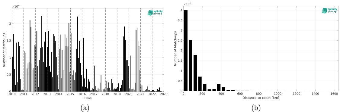
Figure 2: Number of match-ups between ICES and SMOS SSS L4 v1 - Daily (CMEMS-CNR) SSS as a function of time (a) and as function of the distance to coast (b) over the Atlantic Ocean Pi-MEP region and for the full satellite product period.
