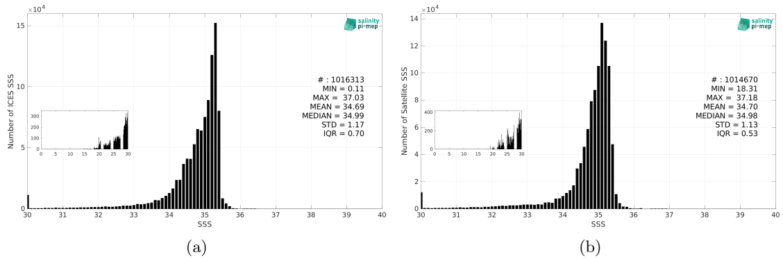
Figure 3: Histograms of SSS from ICES (a) and SMOS SSS L4 v1 - Daily (CMEMS-CNR) (b) considering all match-up pairs per bins of 0.1 over the Atlantic Ocean Pi-MEP region and for the full satellite product period.
