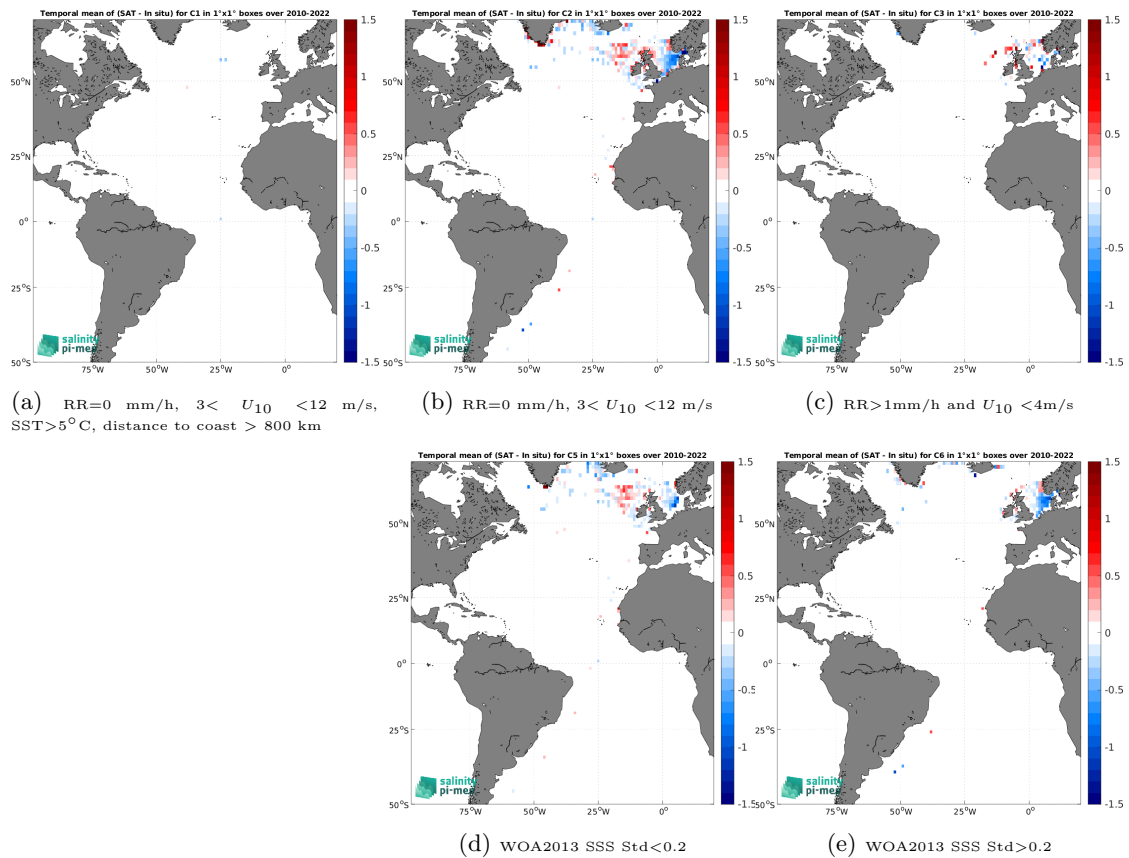
Figure 14: Temporal mean gridded over spatial boxes of size 1^\circ \times 1^\circ of \Delta\text{SSS} (SMOS SSS L4 v1 - Daily (CMEMS-CNR) - ICES) for 5 different subdatasets corresponding to:RR=0 mm/h, 3 < U_{10} < 12 m/s, SST>5°C, distance to coast > 800 km (a), RR=0 mm/h, 3 < U_{10} < 12 m/s (b), RR>1mm/h and U_{10} < 4 m/s (c), WOA2013 SSS Std<0.2 (d), WOA2013 SSS Std>0.2 (e).
