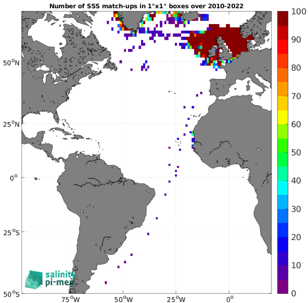
Figure 5: Number of SSS match-ups between ICES SSS and the SMOS SSS L4 v1 - Daily (CMEMS-CNR) SSS product for the Atlantic Ocean Pi-MEP region over 1^\circ \times 1^\circ boxes and for the full satellite product period.
