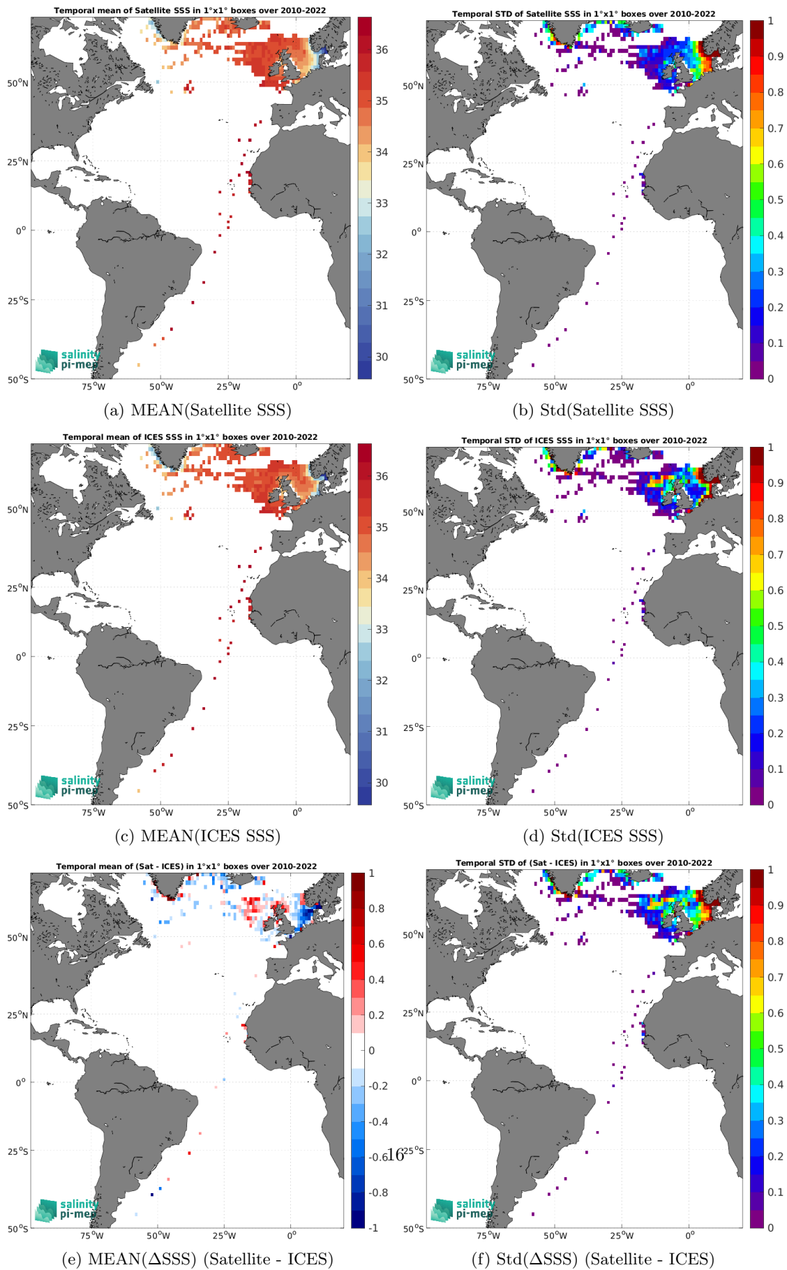
Figure 7: Temporal mean (left) and Std (right) of SSS from SMOS SSS L4 v1 - Daily (CMEMS-CNR) (top), ICES (middle), and of \Delta SSS (Satellite - ICES). Only match-up pairs are used to generate these maps.
