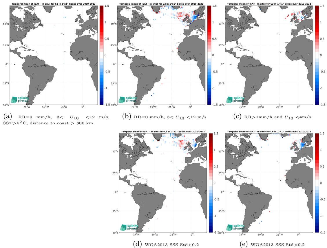
Figure 14: Temporal mean gridded over spatial boxes of size 1^\circ \times 1^\circ of \Delta SSS (SMOS SSS L4 v1 - Daily (CMEMS-CNR) - ICES) for 5 different subdatasets corresponding to:RR=0 mm/h, 3 < U_{10} < 12 m/s, SST >5^\circ\text{C} , distance to coast > 800 km (a), RR=0 mm/h, 3 < U_{10} < 12 m/s (b), RR >1 mm/h and U_{10} < 4 m/s (c), WOA2013 SSS Std <0.2 (d), WOA2013 SSS Std >0.2 (e).
