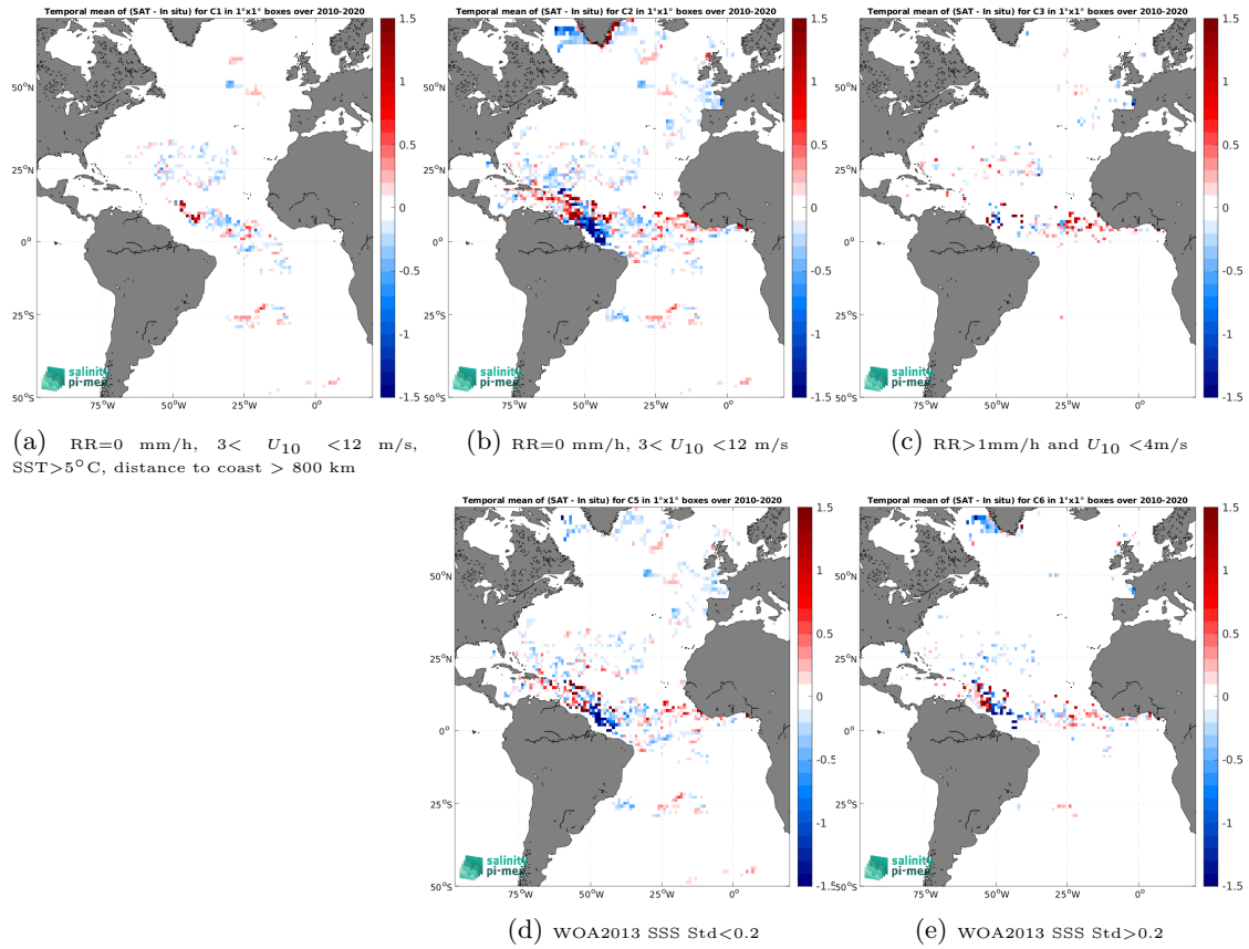
Figure 13: Temporal mean gridded over spatial boxes of size 1^\circ \times 1^\circ of \Delta SSS (SMOS SSS L4 v1 - Daily (CMEMS-CNR) - Surface drifters) for 5 different subdatasets corresponding to:RR=0 mm/h, 3 < U_{10} < 12 m/s, SST >5^\circ\text{C} , distance to coast > 800 km (a), RR=0 mm/h, 3 < U_{10} < 12 m/s (b), RR >1 mm/h and U_{10} < 4 m/s (c), WOA2013 SSS Std <0.2 (d), WOA2013 SSS Std >0.2 (e).
