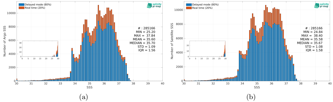
Figure 3: Histograms of SSS from Argo (a) and SMOS SSS L4 v1 - Daily (CMEMS-CNR) (b) considering all match-up pairs per bins of 0.1 over the Atlantic Ocean Pi-MEP region and for the full satellite product period.
