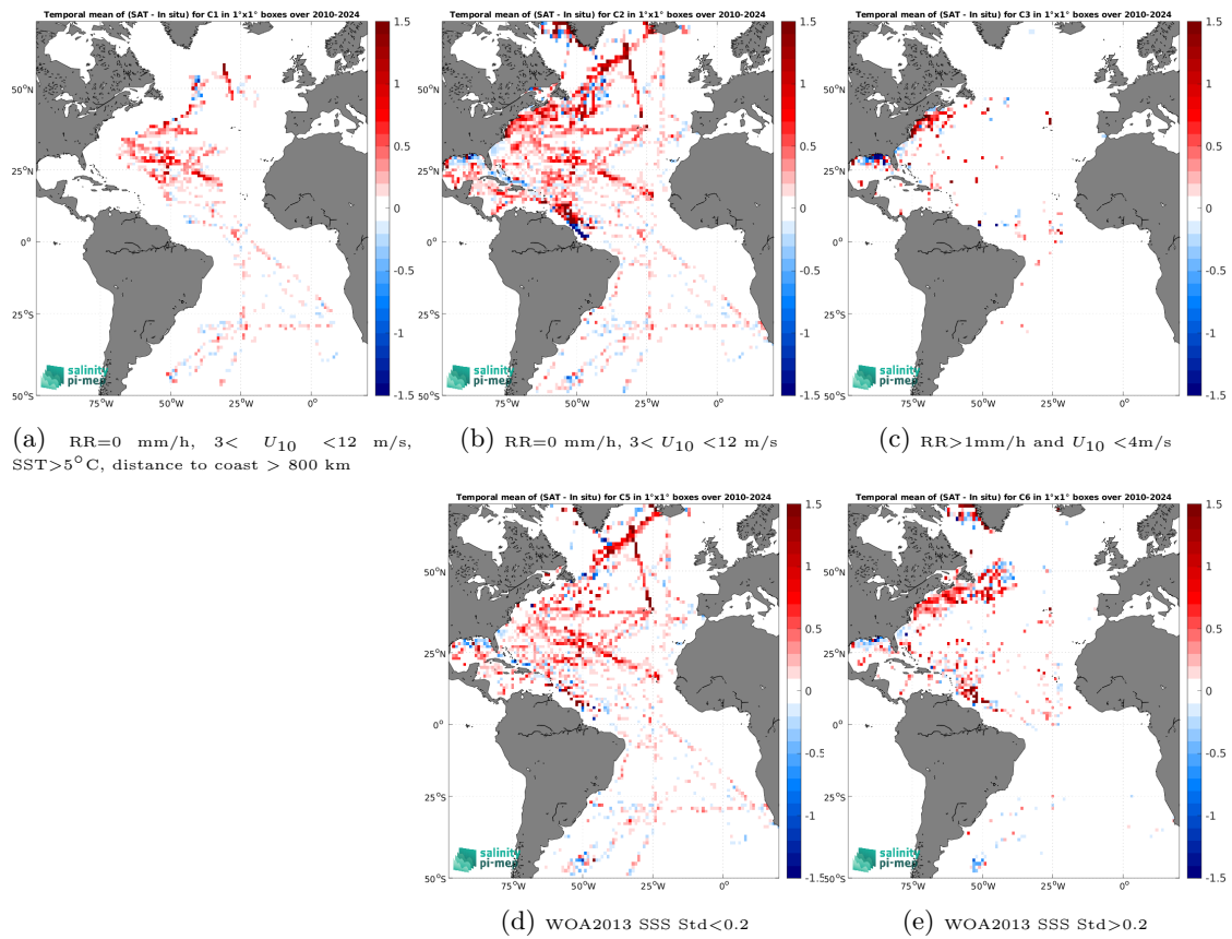
Figure 14: Temporal mean gridded over spatial boxes of size 1^\circ \times 1^\circ of \Delta\text{SSS} (SMOS SSS L4 OI v346 - Weekly (CMEMS-CATDS-LOPS) - TSG (SAMOS)) for 5 different subdatasets corresponding to:RR=0 mm/h, 3 < U_{10} < 12 m/s, SST >5^\circ\text{C} , distance to coast > 800 km (a), RR=0 mm/h, 3 < U_{10} < 12 m/s (b), RR >1 mm/h and U_{10} < 4 m/s (c), WOA2013 SSS Std <0.2 (d), WOA2013 SSS Std >0.2 (e).
