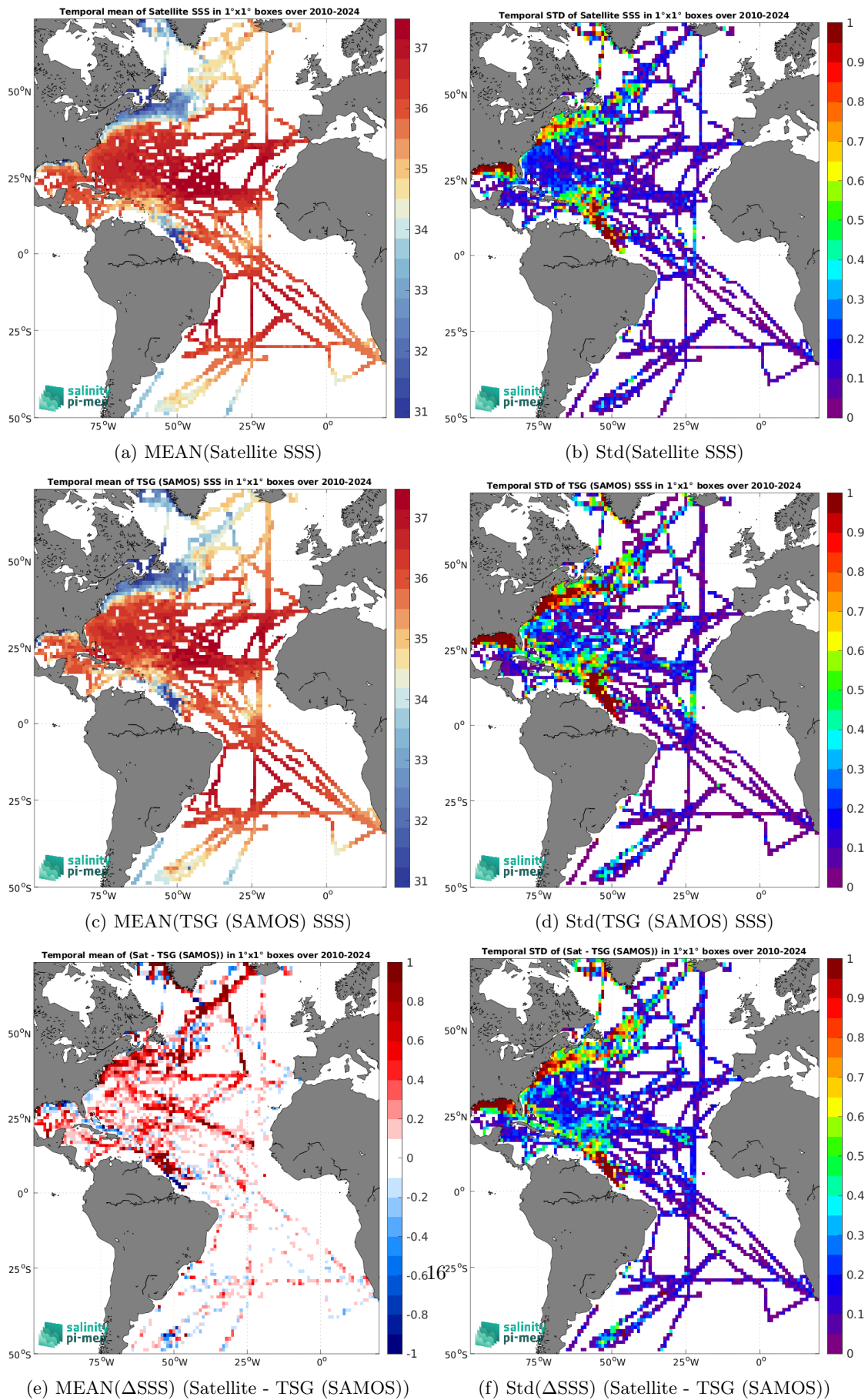
Figure 7: Temporal mean (left) and Std (right) of SSS from SMOS SSS L4 OI v346 - Weekly (CMEMS-CATDS-LOPS) (top), TSG (SAMOS) (middle), and of \Delta SSS (Satellite - TSG (SAMOS)). Only match-up pairs are used to generate these maps.
