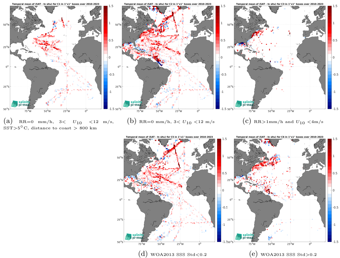
Figure 14: Temporal mean gridded over spatial boxes of size 1^\circ \times 1^\circ of \Delta SSS (SMOS SSS L4 OI v346 - Weekly (CMEMS-CATDS-LOPS) - TSG (SAMOS)) for 5 different subdatasets corresponding to:RR=0 mm/h, 3 < U_{10} < 12 m/s, SST>5°C, distance to coast > 800 km (a), RR=0 mm/h, 3 < U_{10} < 12 m/s (b), RR>1mm/h and U_{10} < 4 m/s (c), WOA2013 SSS Std<0.2 (d), WOA2013 SSS Std>0.2 (e).
