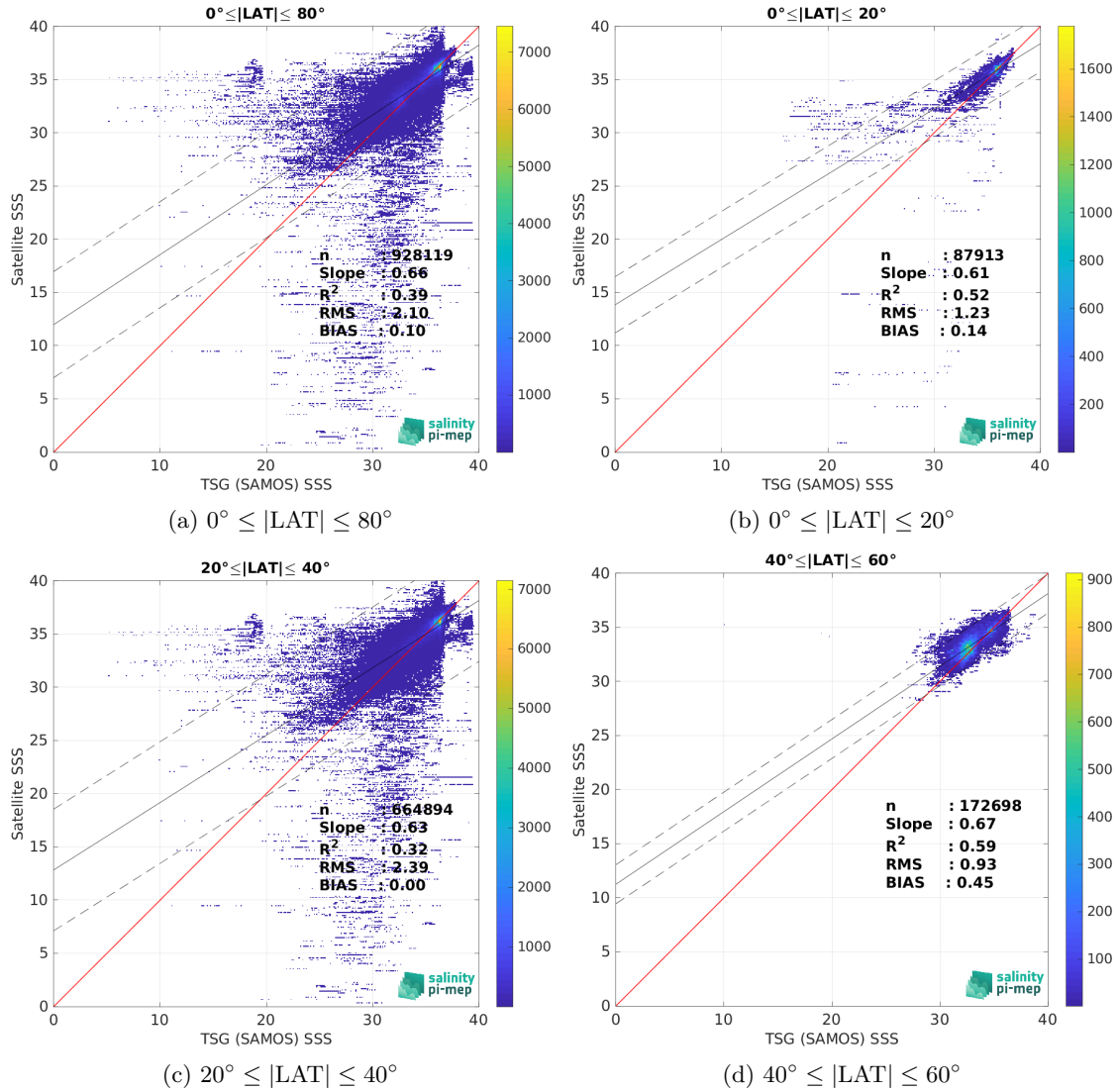
Figure 10: Contour maps of the concentration of SMOS SSS L4 OI v346 - Weekly (CMEMS-CATDS-LOPS) SSS (y-axis) versus TSG (SAMOS) SSS (x-axis) at match-up pairs for different latitude bands. For each plot, the red line shows x=y . The black thin and dashed lines indicate a linear fit through the data cloud and the \pm 95\% confidence levels, respectively. The number match-up pairs n , the slope and R^2 coefficient of the linear fit, the root mean square (RMS) and the mean bias between satellite and in situ data are indicated for each latitude band in each plots.
