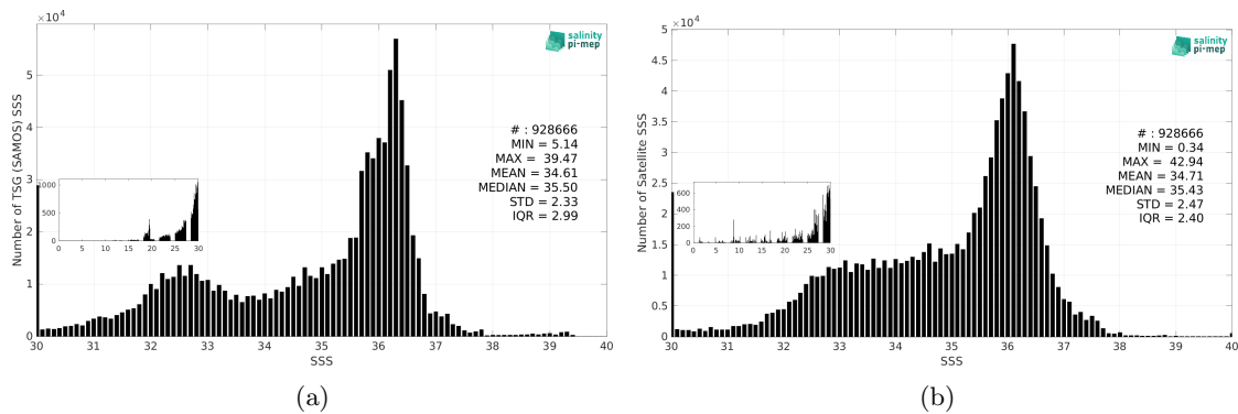
Figure 3: Histograms of SSS from TSG (SAMOS) (a) and SMOS SSS L4 OI v346 - Weekly (CMEMS-CATDS-LOPS) (b) considering all match-up pairs per bins of 0.1 over the Atlantic Ocean Pi-MEP region and for the full satellite product period.
