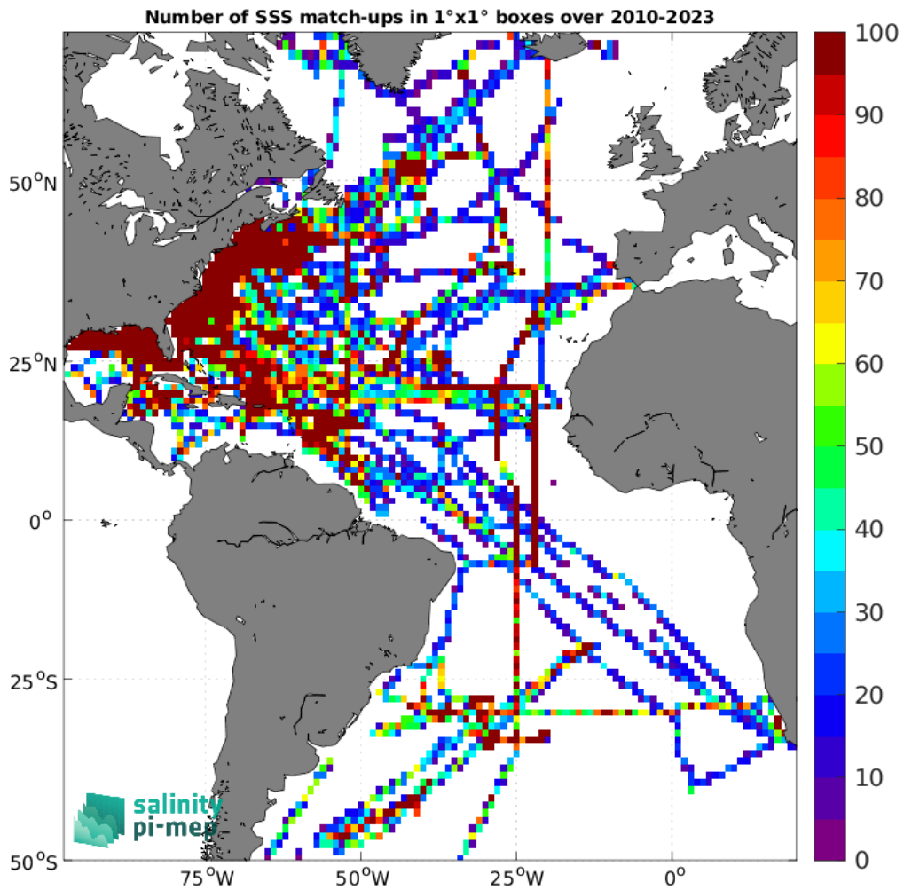
Figure 5: Number of SSS match-ups between TSG (SAMOS) SSS and the SMOS SSS L4 OI v346 - Weekly (CMEMS-CATDS-LOPS) SSS product for the Atlantic Ocean Pi-MEP region over 1^\circ \times 1^\circ boxes and for the full satellite product period.
