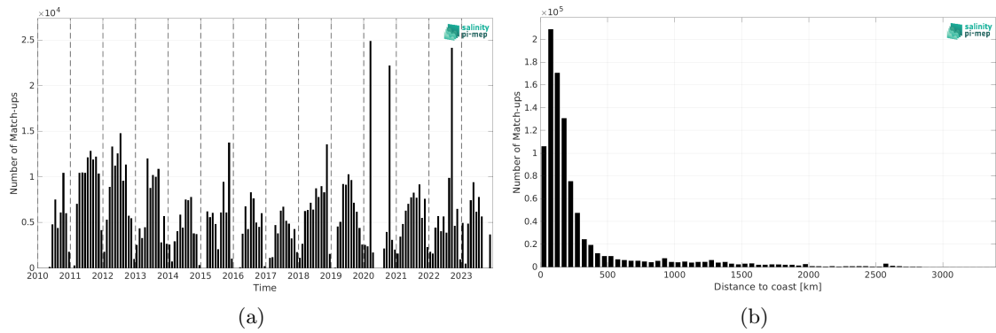
Figure 2: Number of match-ups between TSG (SAMOS) and SMOS SSS L4 OI v346 - Weekly (CMEMS-CATDS-LOPS) SSS as a function of time (a) and as function of the distance to coast (b) over the Atlantic Ocean Pi-MEP region and for the full satellite product period.
