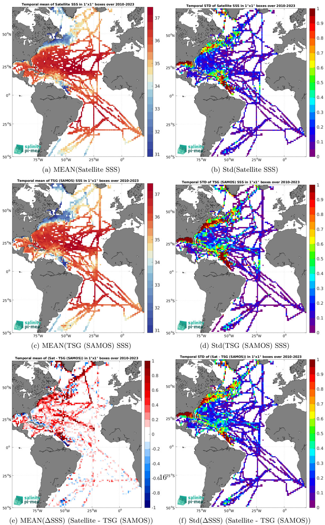
(e) MEAN( \Delta SSS) (Satellite - TSG (SAMOS)) (f) Std( \Delta SSS) (Satellite - TSG (SAMOS)) Figure 7: Temporal mean (left) and Std (right) of SSS from SMOS SSS L4 OI v346 - Weekly (CMEMS-CATDS-LOPS) (top), TSG (SAMOS) (middle), and of \Delta SSS (Satellite - TSG (SAMOS)). Only match-up pairs are used to generate these maps.
