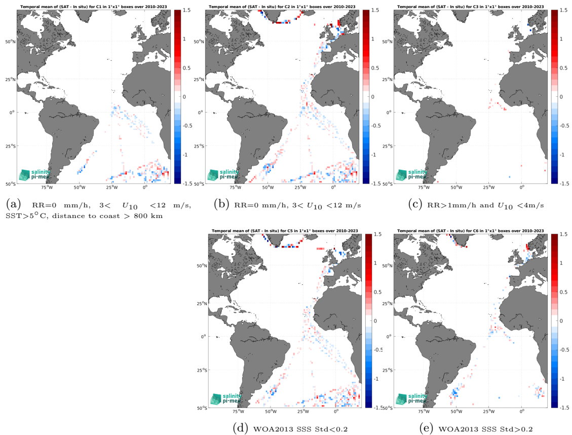
Figure 14: Temporal mean gridded over spatial boxes of size 1^\circ \times 1^\circ of \Delta\text{SSS} (SMOS SSS L4 OI v346 - Weekly (CMEMS-CATDS-LOPS) - TSG (Polarstern)) for 5 different subdatasets corresponding to:RR=0 mm/h, 3 < U_{10} < 12 m/s, SST >5^\circ\text{C} , distance to coast > 800 km (a), RR=0 mm/h, 3 < U_{10} < 12 m/s (b), RR >1 mm/h and U_{10} < 4 m/s (c), WOA2013 SSS Std <0.2 (d), WOA2013 SSS Std >0.2 (e).
