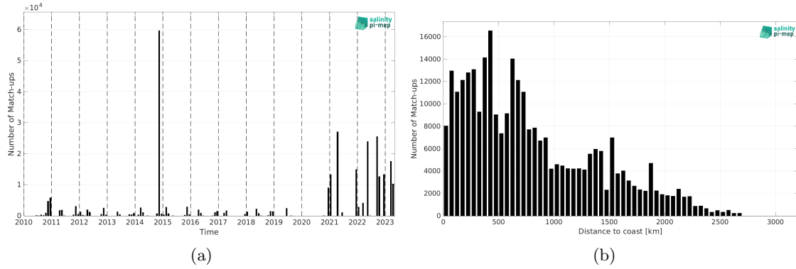
Figure 2: Number of match-ups between TSG (Polarstern) and SMOS SSS L4 OI v346 - Weekly (CMEMS-CATDS-LOPS) SSS as a function of time (a) and as function of the distance to coast (b) over the Atlantic Ocean Pi-MEP region and for the full satellite product period.
