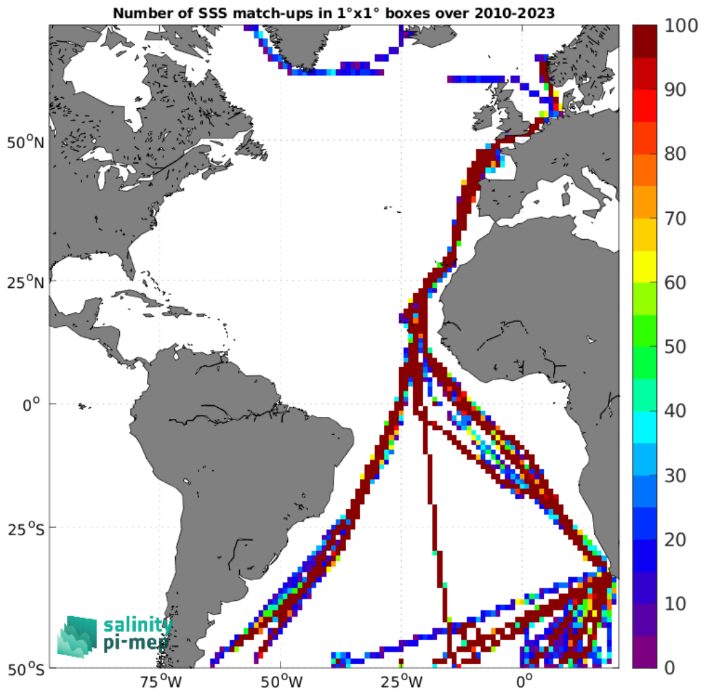
Figure 5: Number of SSS match-ups between TSG (Polarstern) SSS and the SMOS SSS L4 OI v346 - Weekly (CMEMS-CATDS-LOPS) SSS product for the Atlantic Ocean Pi-MEP region over 1°x1° boxes and for the full satellite product period.
