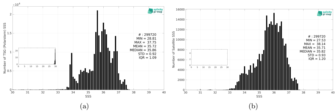
Figure 3: Histograms of SSS from TSG (Polarstern) (a) and SMOS SSS L4 OI v346 - Weekly (CMEMS-CATDS-LOPS) (b) considering all match-up pairs per bins of 0.1 over the Atlantic Ocean Pi-MEP region and for the full satellite product period.
