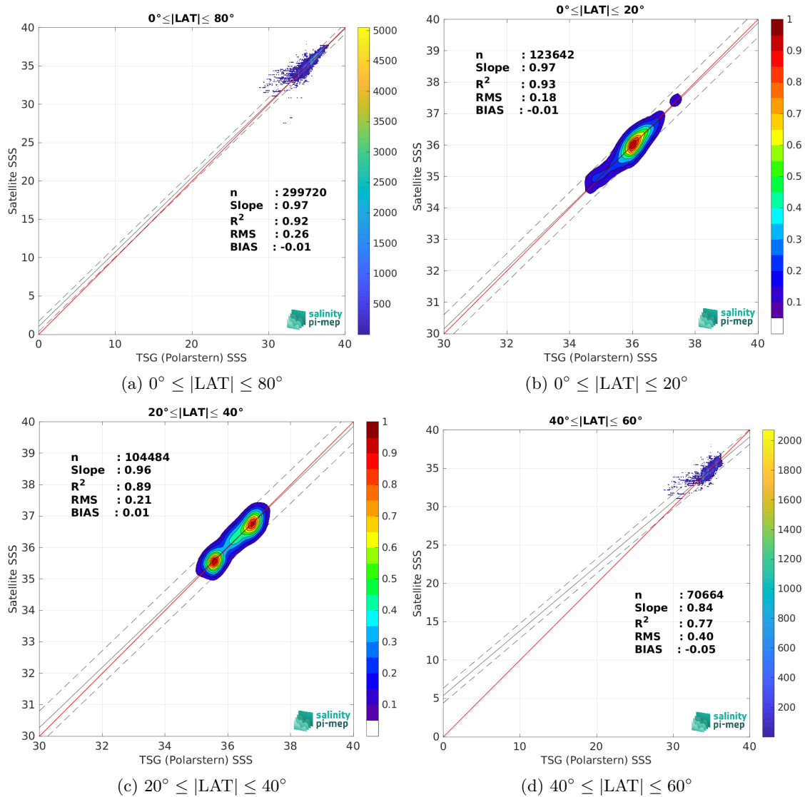
Figure 10: Contour maps of the concentration of SMOS SSS L4 OI v346 - Weekly (CMEMS-CATDS-LOPS) SSS (y-axis) versus TSG (Polarstern) SSS (x-axis) at match-up pairs for different latitude bands. For each plot, the red line shows x=y . The black thin and dashed lines indicate a linear fit through the data cloud and the \pm 95\% confidence levels, respectively. The number match-up pairs n , the slope and R^2 coefficient of the linear fit, the root mean square (RMS) and the mean bias between satellite and in situ data are indicated for each latitude band in each plots.
